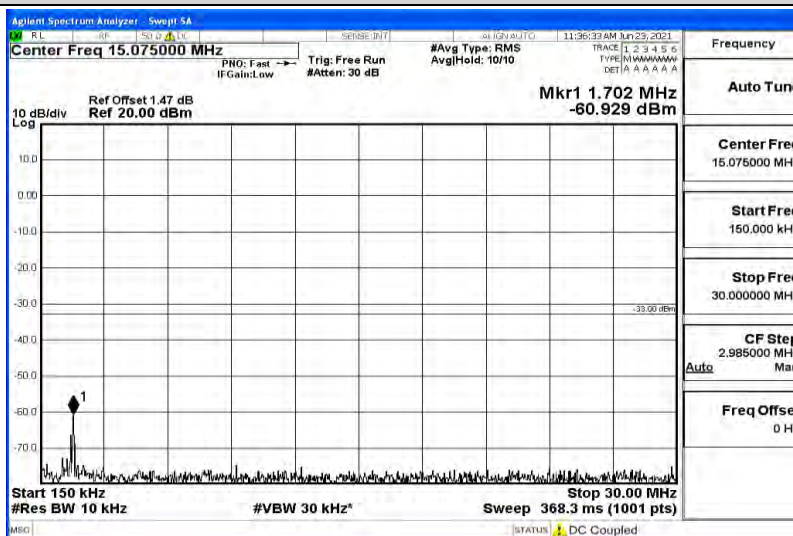
Band2-10MHz-QPSK-18900-1RB#0-Range3:30~1000MHz
