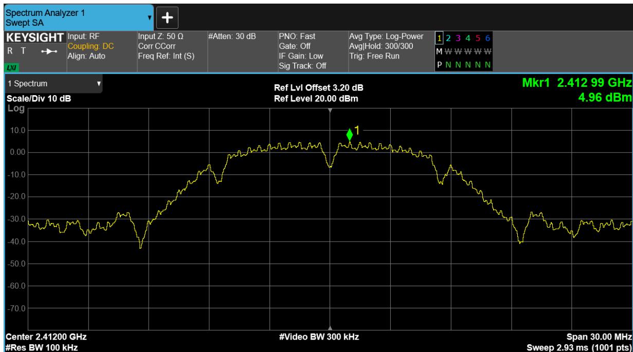
Band Edge NVNT b 2412MHz Ant1 Emission
