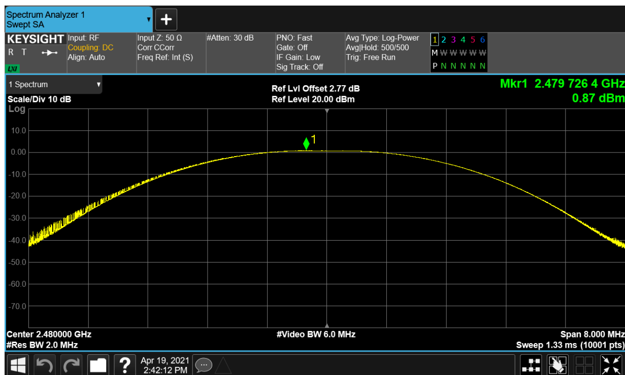
-6dB Bandwidth
