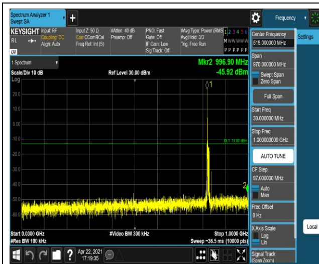
Band5-10MHz-QPSK-20525-1RB#0-Range1:30~1000MHz
