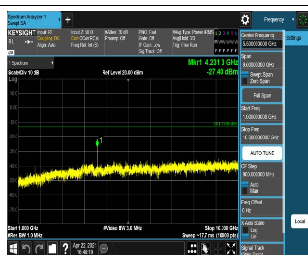
Band5-3MHz-16QAM-20415-1RB#0-Range2:1000~10000MHz
