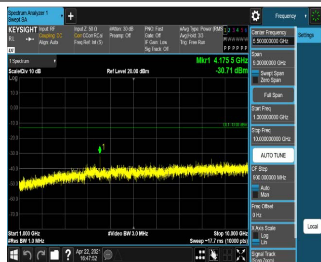
Band5-3MHz-16QAM-20525-1RB#0-Range2:1000~10000MHz
