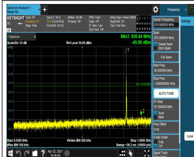
Band5-3MHz-16QAM-20525-1RB#0-Range1:30~1000MHz
