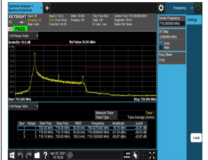
Band17-10MHz-QPSK-23800-50RB#0
