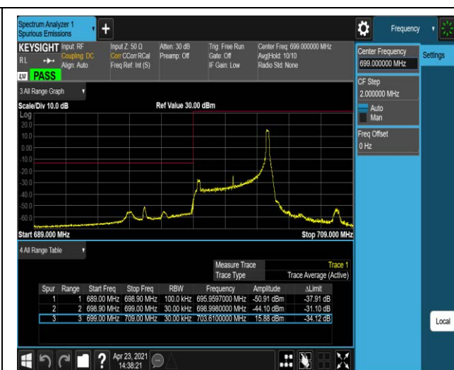
Band12-5MHz-QPSK-23155-1RB#0
