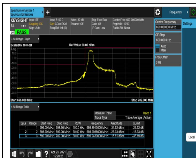
Band12-1.4MHz-QPSK-23017-6RB#0
