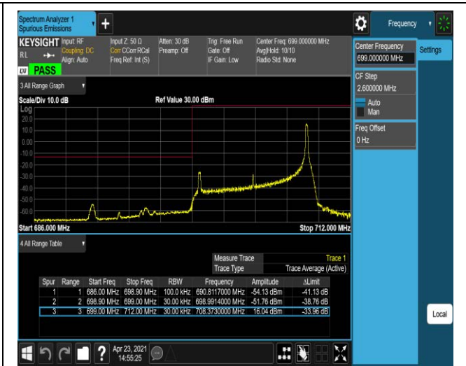
Band12-10MHz-QPSK-23130-1RB#0
