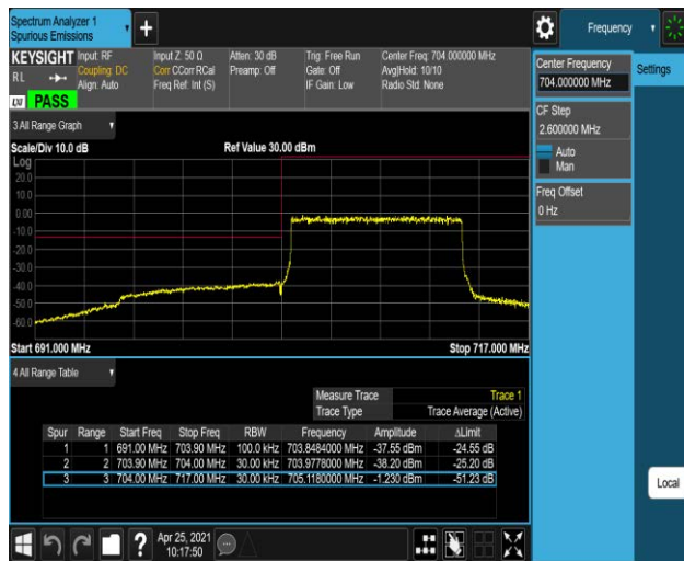
Band17-10MHz-QPSK-23800-1RB#49
