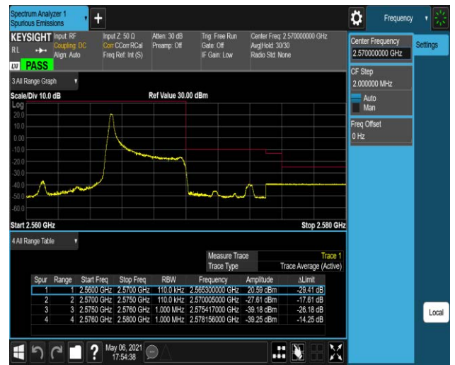
Band7-5MHz-QPSK-21425-25RB#0
