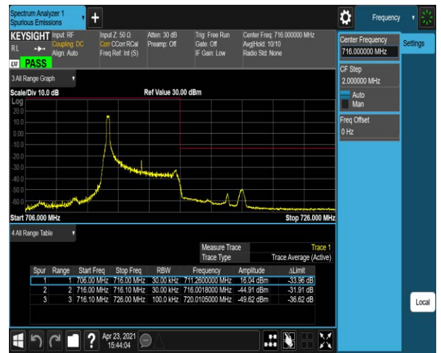
Band17-5MHz-QPSK-23825-25RB#0
