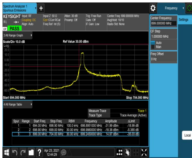
Band12-3MHz-16QAM-23025-15RB#0
