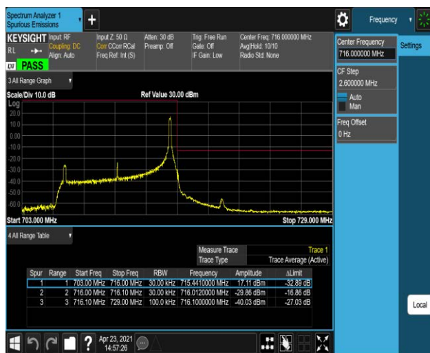
Band12-10MHz-16QAM-23060-1RB#0
