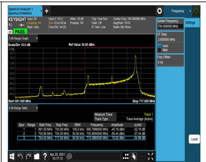
Band17-10MHz-QPSK-23800-1RB#0
