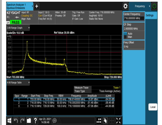
Band12-10MHz-QPSK-23130-50RB#0
