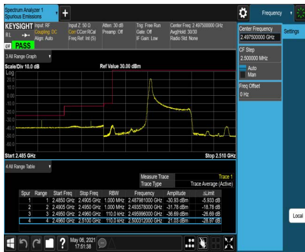
Band7-5MHz-QPSK-20775-25RB#0
