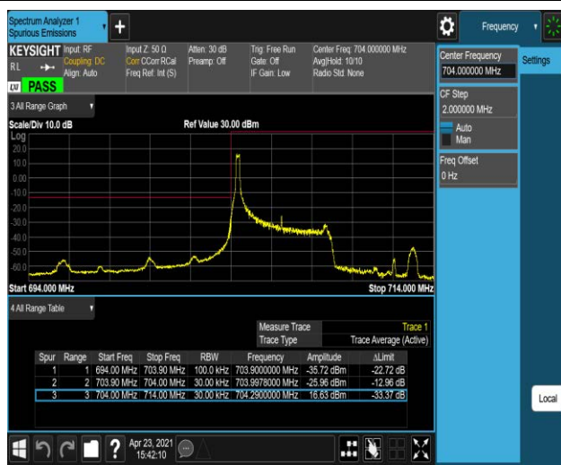
Band17-5MHz-QPSK-23755-25RB#0
