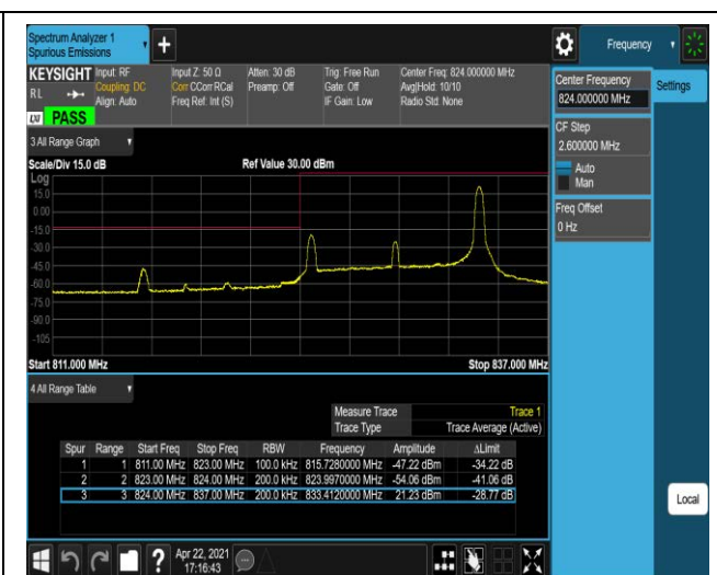
Band5-10MHz-16QAM-20600-1RB#0
