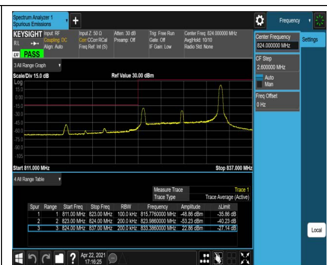
Band5-10MHz-QPSK-20600-1RB#0
