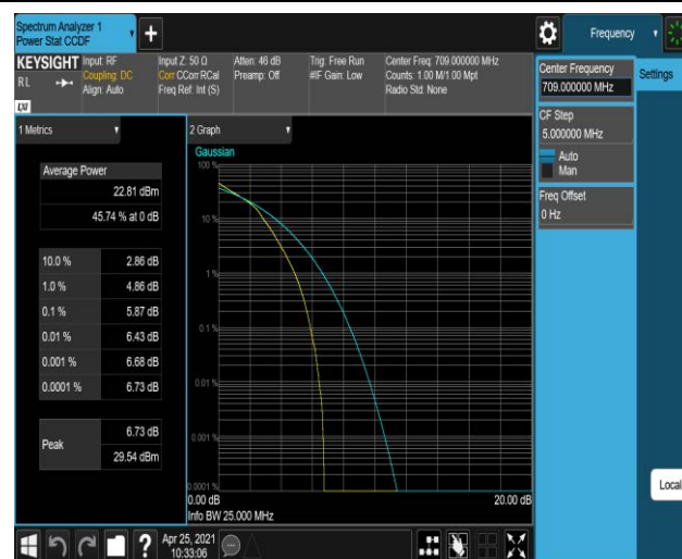
Band17-10MHz-16QAM-23780-50RB#0
