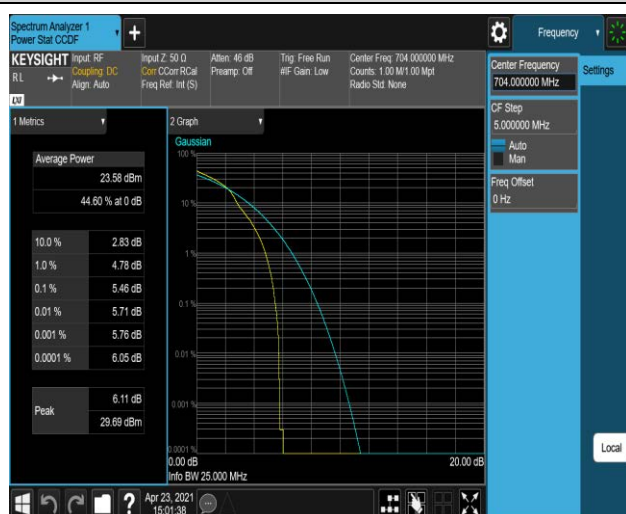
Band12-10MHz-16QAM-23060-1RB#0
