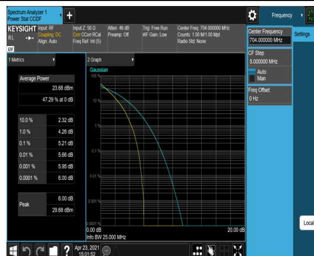
Band12-10MHz-QPSK-23060-50RB#0
