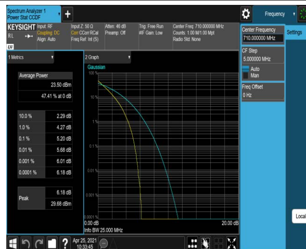
Band17-10MHz-QPSK-23800-50RB#0
