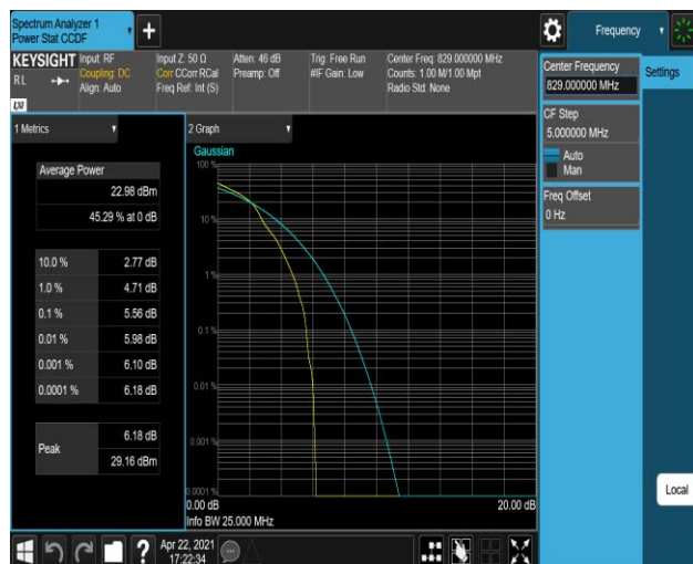
Band5-10MHz-16QAM-20525-1RB#0
