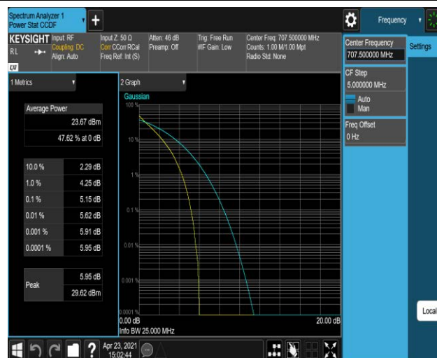
Band12-10MHz-QPSK-23130-50RB#0
