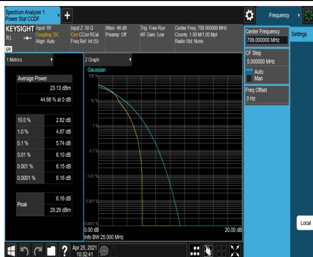
Band17-10MHz-16QAM-23780-1RB#0
