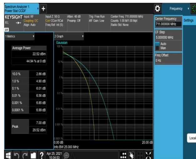
Band17-10MHz-16QAM-23800-50RB#0
