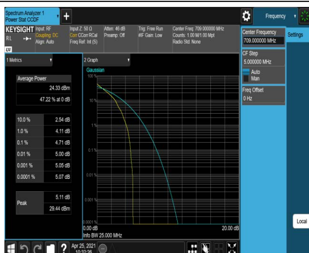
Band17-10MHz-QPSK-23780-1RB#0
