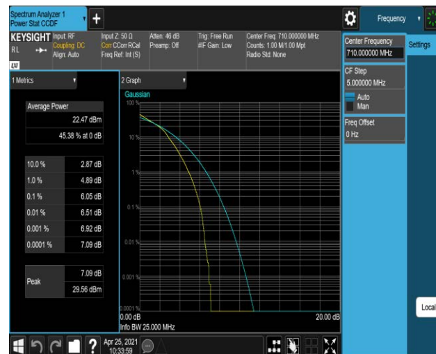
Band17-10MHz-16QAM-23800-50RB#0
