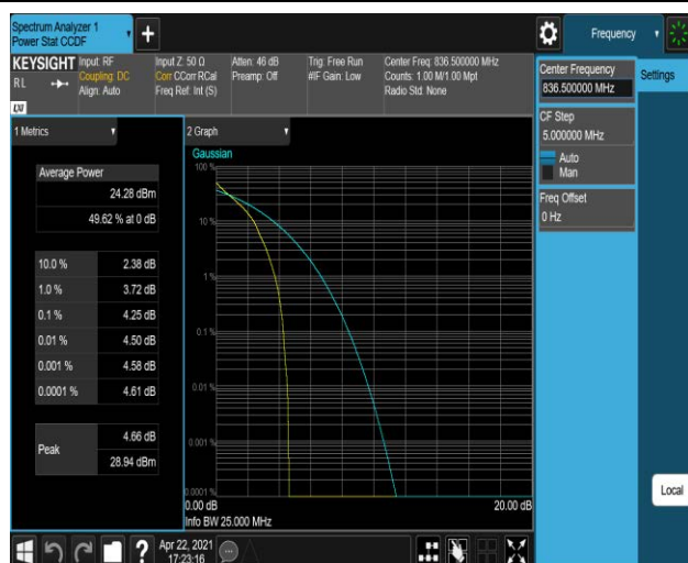
Band5-10MHz-QPSK-20525-1RB#0
