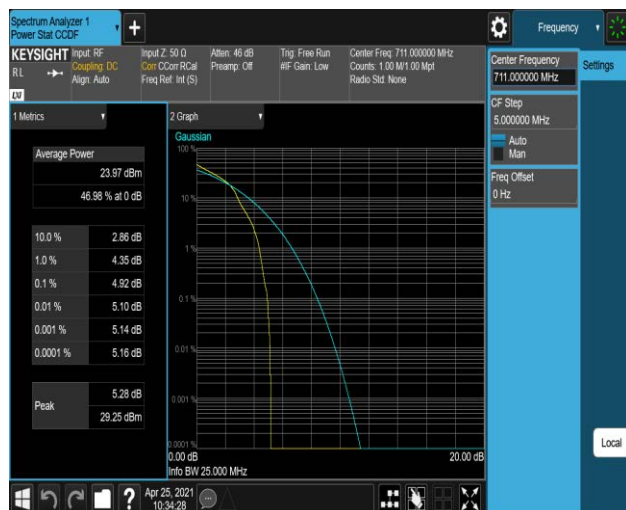
Band17-10MHz-16QAM-23800-1RB#0
