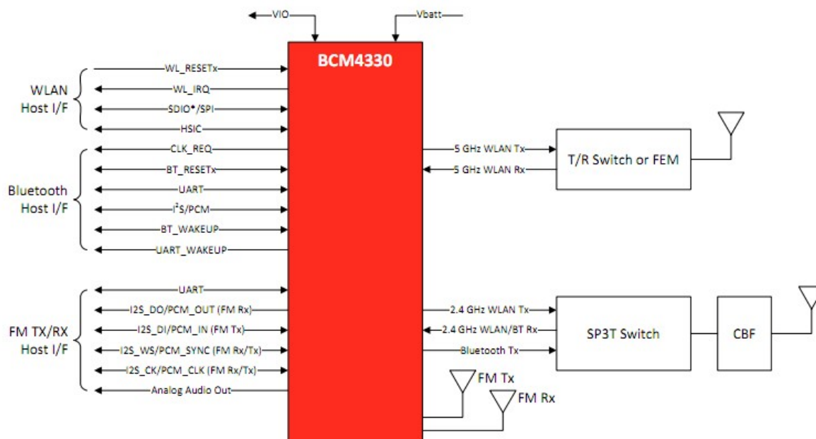
WIFI/BT operation block
