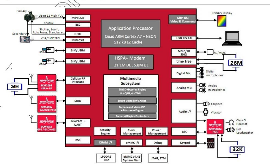
Figure 1: Functional Block Diagram of a BCM23550-Based 3G Platform Solution
