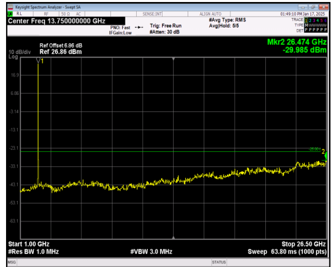
Band7-20MHz-16QAM-21100-1RB#0-Range2:1000~26500MHz
