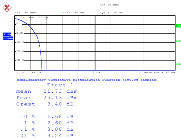
UMTS 1900 RMC
