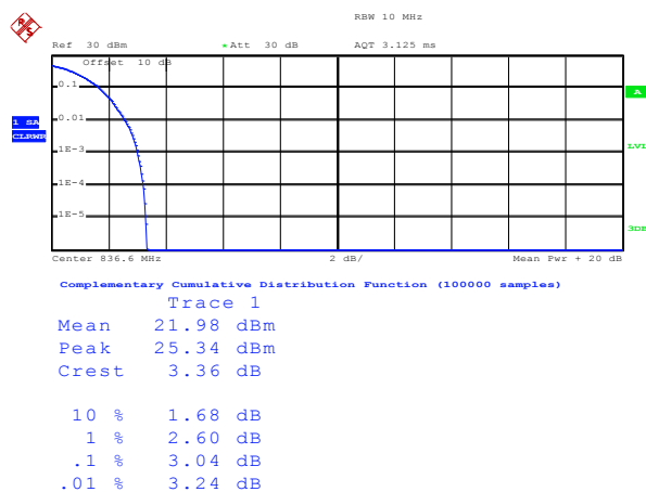
UMTS 850 RMC
