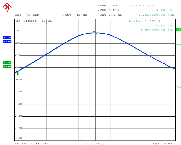
PCS 1900
