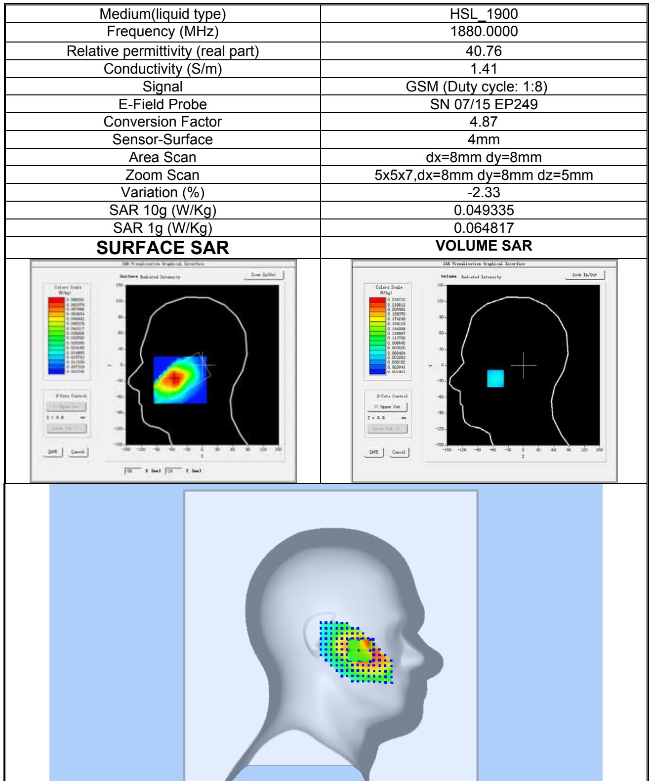
Plot 3: GSM1900, Middle channel (Left Head Cheek) Product Description: 1.77 Inch 3G Wireless Fixed Phone Test Date: 2018-03-21
