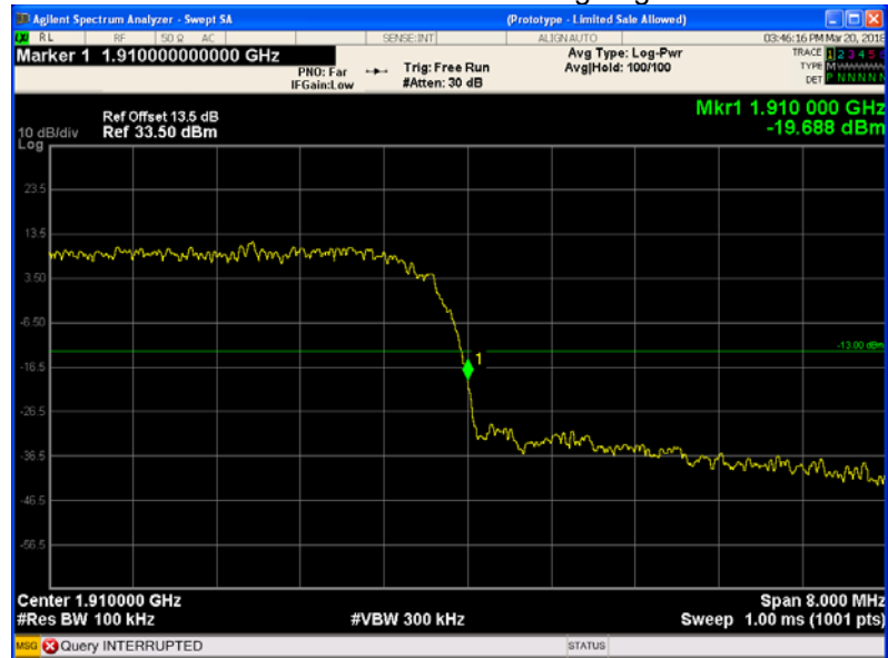
WCDMA band II band edge-right side
