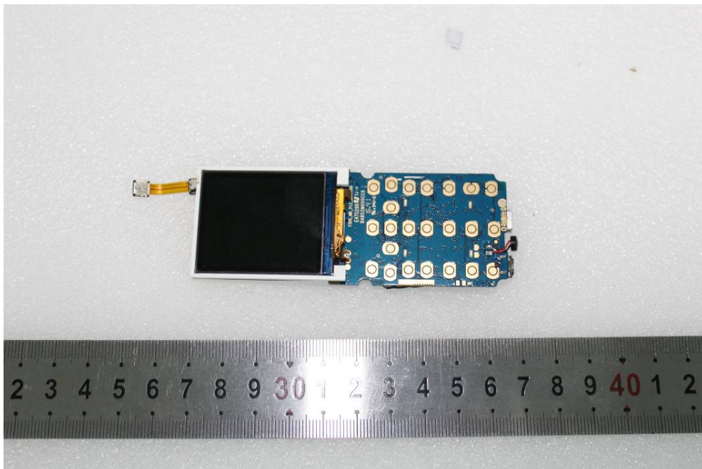
EUT – Main Board Top Shilding off View 1
