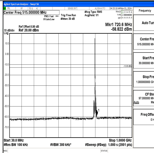
Band12-5MHz-QPSK-23095-1RB#0-30~1000-PASS
