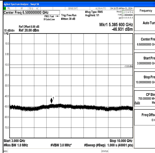
Band12-3MHz-16QAM-23165-1RB#0-3000~10000-PASS
