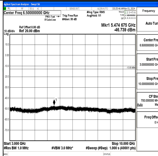
Band12-1.4MHz-16QAM-23095-1RB#0-3000~10000-PASS
