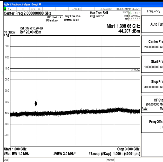
Band12-5MHz-QPSK-23035-1RB#0-1000~3000-PASS
