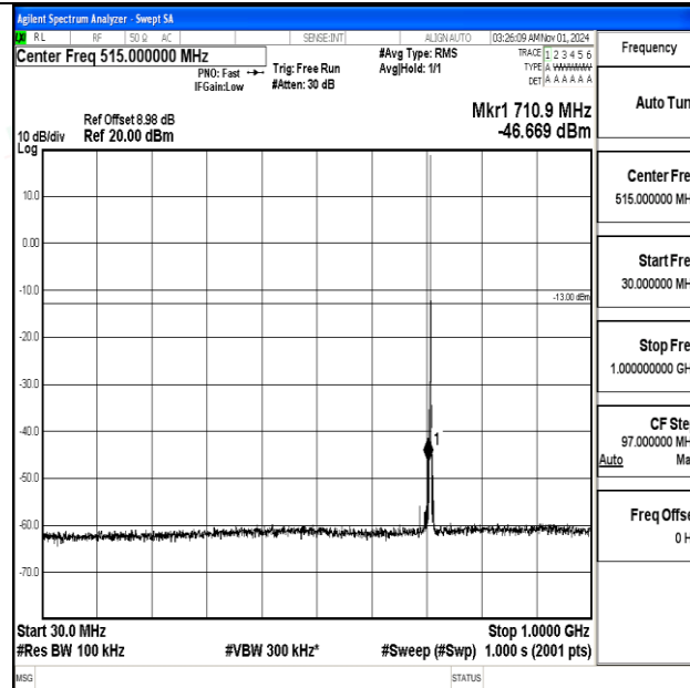
Band12-1.4MHz-QPSK-23173-1RB#0-30~1000-PASS
