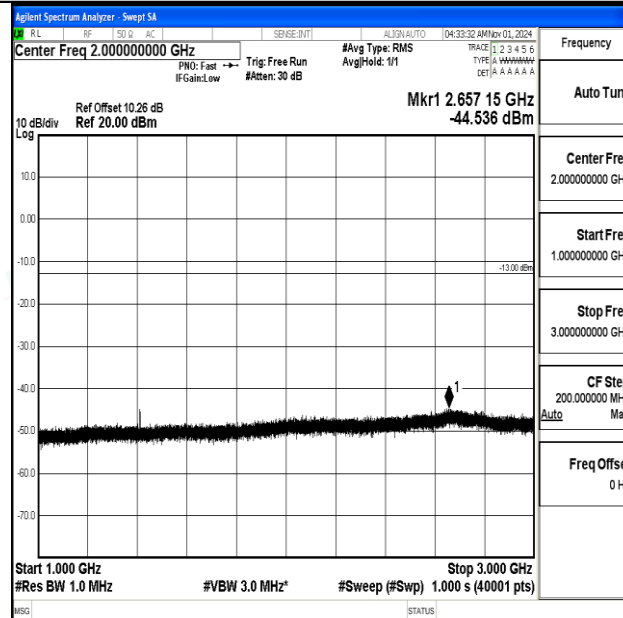
Band12-5MHz-QPSK-23095-1RB#0-1000~3000-PASS
