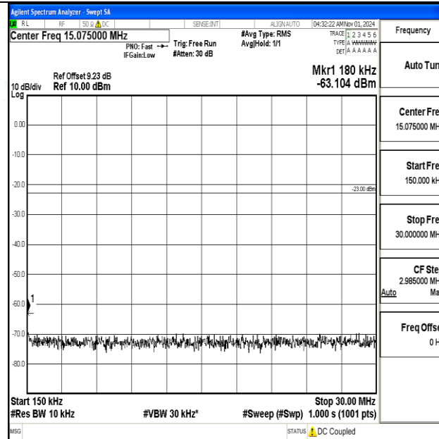
Band12-5MHz-16QAM-23035-1RB#0-0.15~30-PASS
