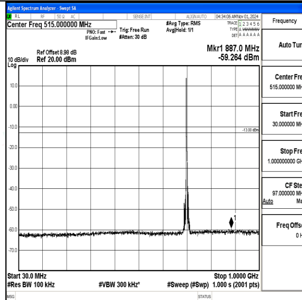
Band12-5MHz-16QAM-23095-1RB#0-30~1000-PASS
