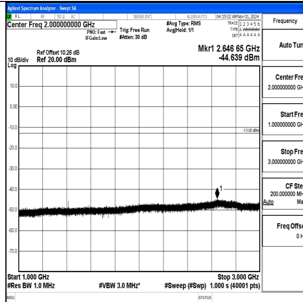
Band12-3MHz-16QAM-23095-1RB#0-1000~3000-PASS
