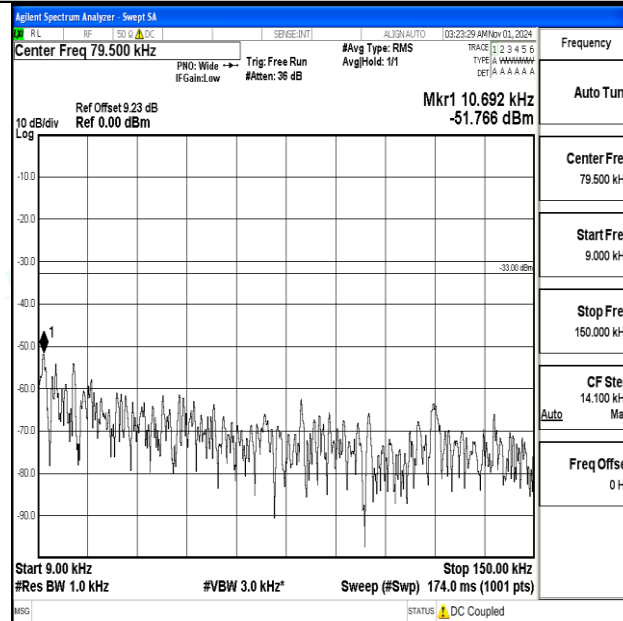
Band12-1.4MHz-16QAM-23017-1RB#0-0.009~0.15-PASS
