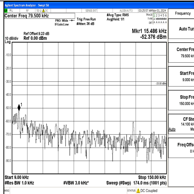
Band12-1.4MHz-QPSK-23173-1RB#0-0.009~0.15-PASS
