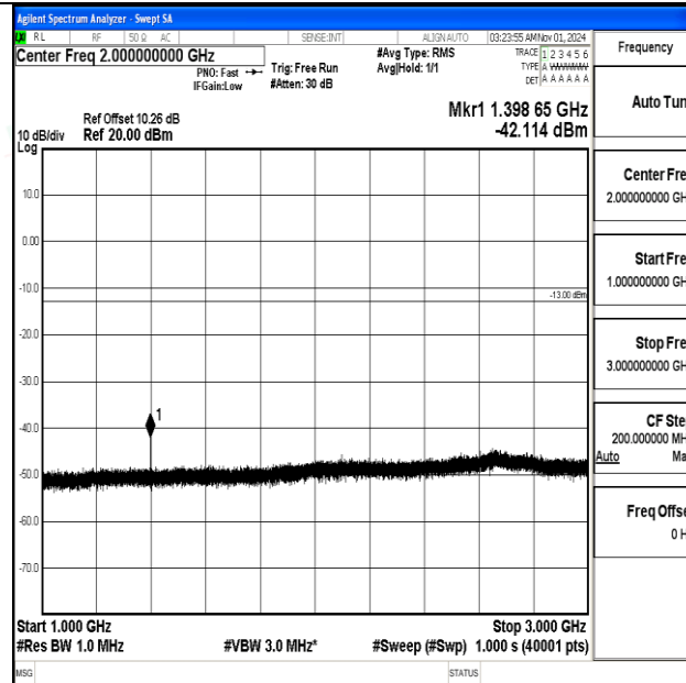
Band12-1.4MHz-16QAM-23017-1RB#0-1000~3000-PASS
