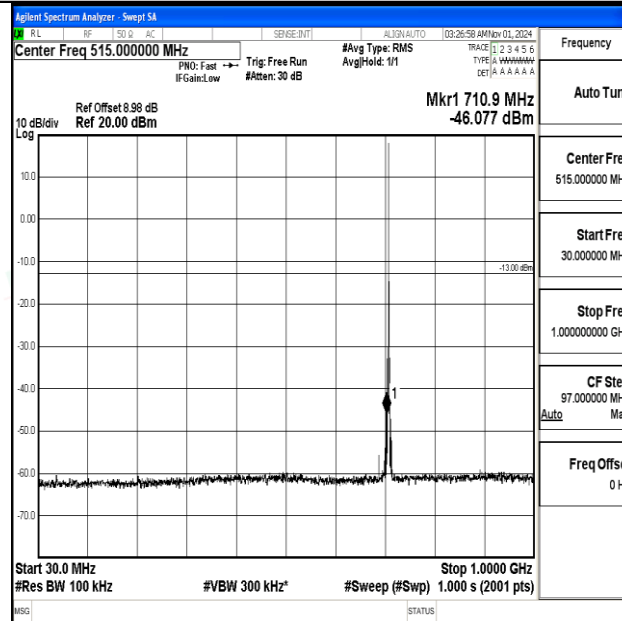
Band12-1.4MHz-16QAM-23173-1RB#0-30~1000-PASS
