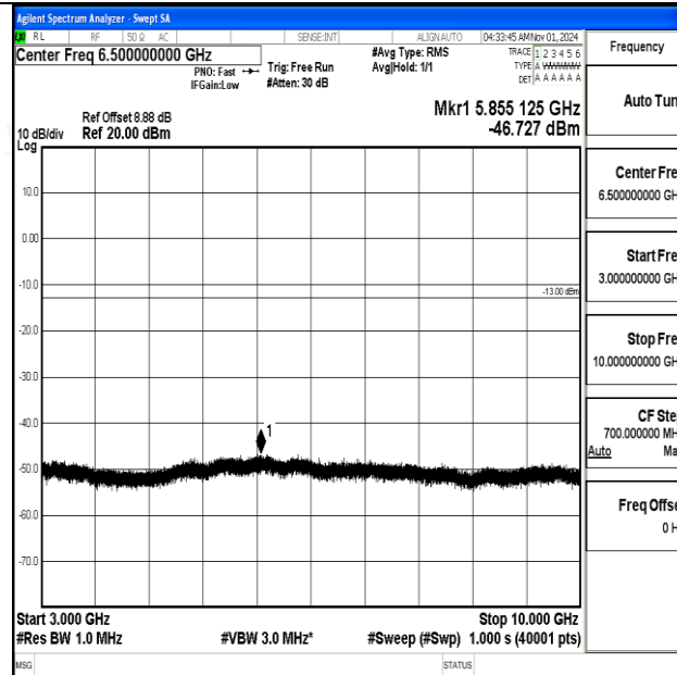
Band12-5MHz-QPSK-23095-1RB#0-3000~10000-PASS
