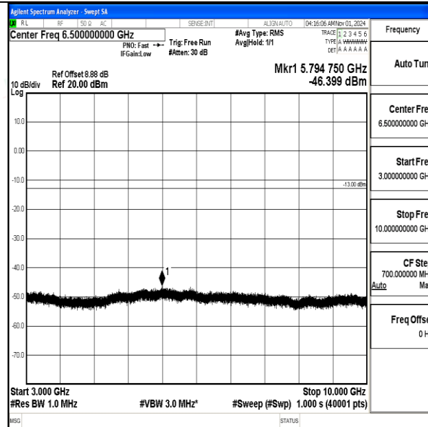
Band12-3MHz-QPSK-23165-1RB#0-3000~10000-PASS
