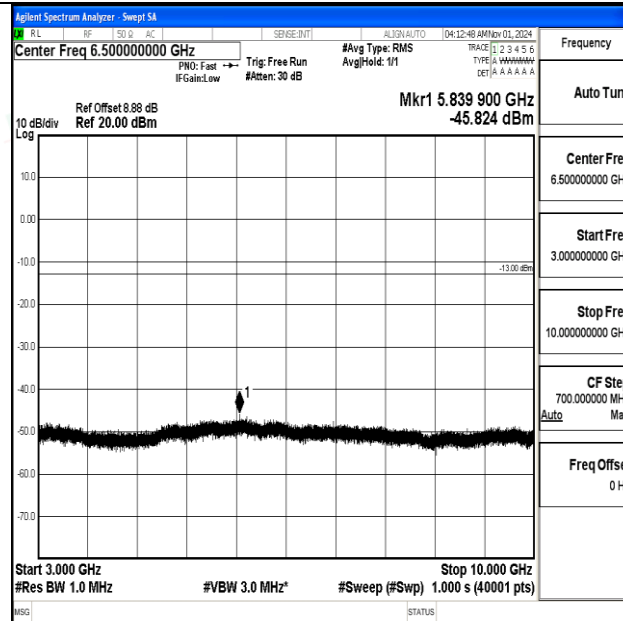
Band12-3MHz-QPSK-23025-1RB#0-3000~10000-PASS
