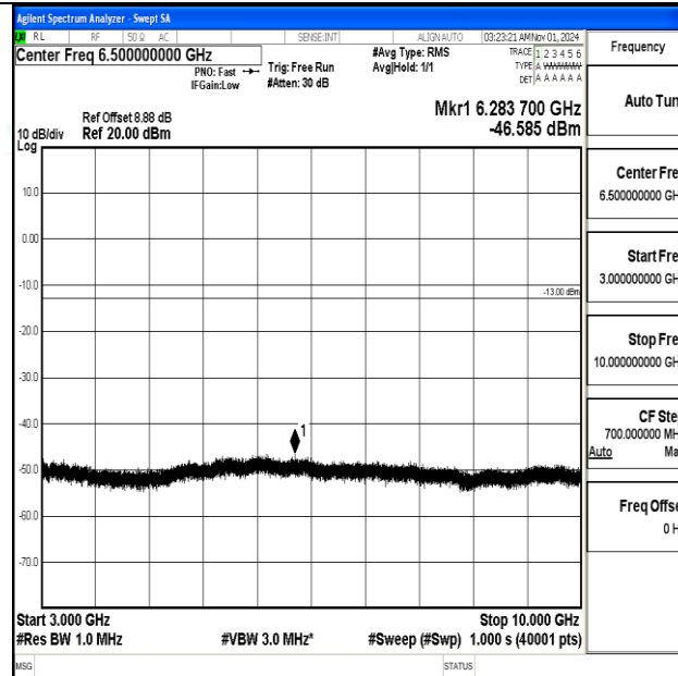
Band12-1.4MHz-QPSK-23017-1RB#0-3000~10000-PASS
