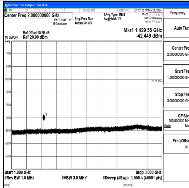
Band12-1.4MHz-16QAM-23173-1RB#0-1000~3000-PASS
