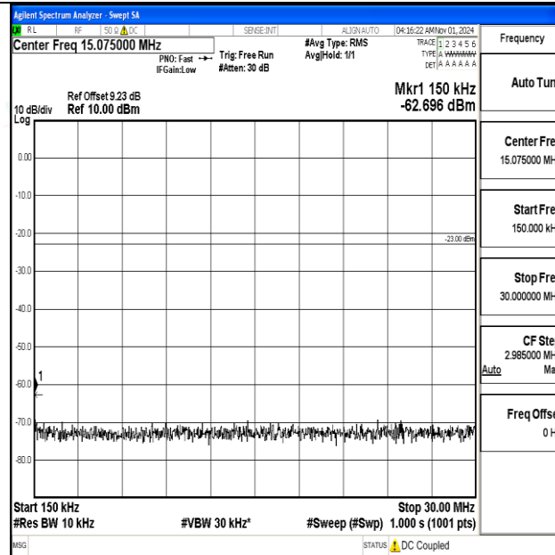
Band12-3MHz-16QAM-23165-1RB#0-0.15~30-PASS
