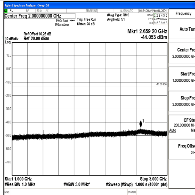
Band12-5MHz-16QAM-23095-1RB#0-1000~3000-PASS
