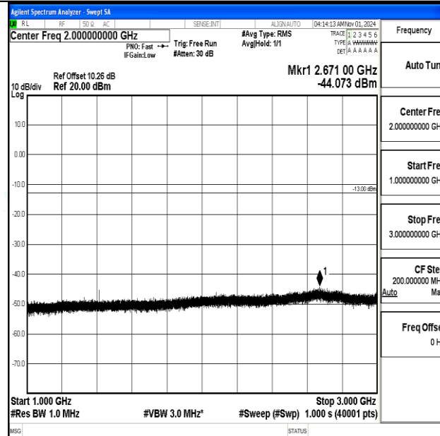
Band12-3MHz-QPSK-23095-1RB#0-1000~3000-PASS
