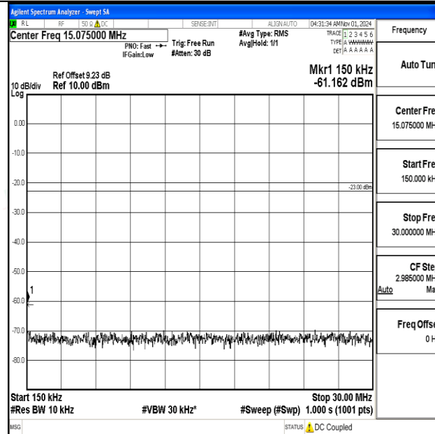
Band12-5MHz-QPSK-23035-1RB#0-0.15~30-PASS
