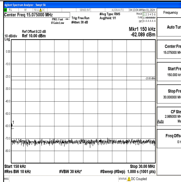
Band12-3MHz-16QAM-23025-1RB#0-0.15~30-PASS
