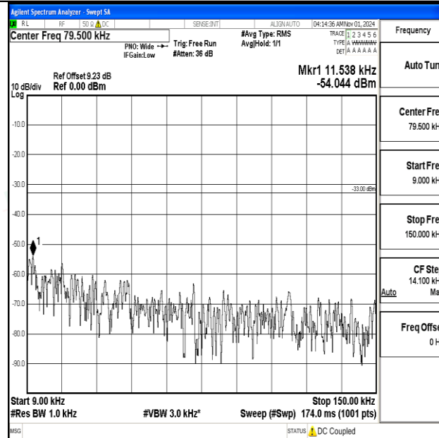
Band12-3MHz-16QAM-23095-1RB#0-0.009~0.15-PASS
