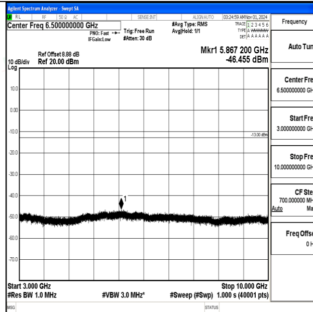
Band12-1.4MHz-QPSK-23095-1RB#0-3000~10000-PASS
