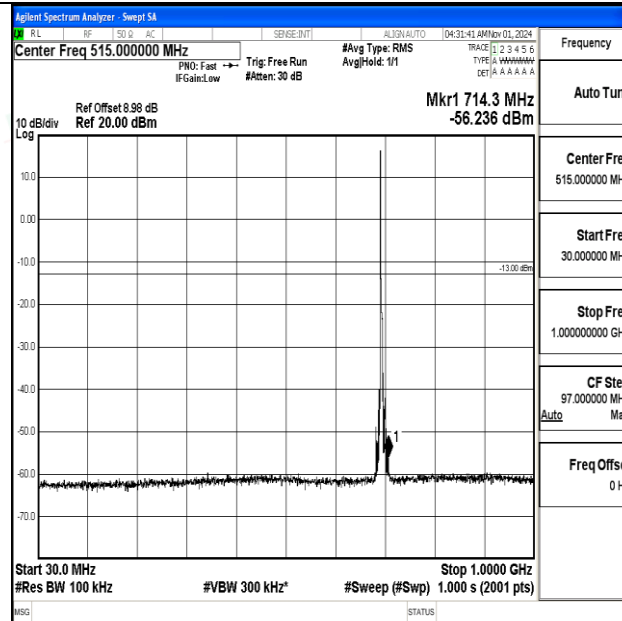
Band12-5MHz-QPSK-23035-1RB#0-30~1000-PASS
