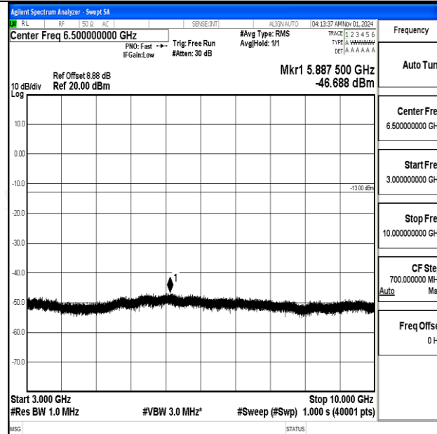
Band12-3MHz-16QAM-23025-1RB#0-3000~10000-PASS
