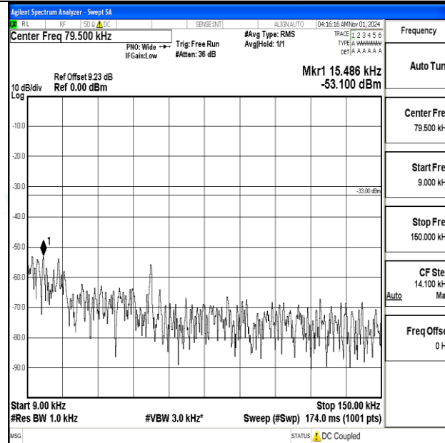
Band12-3MHz-16QAM-23165-1RB#0-0.009~0.15-PASS
