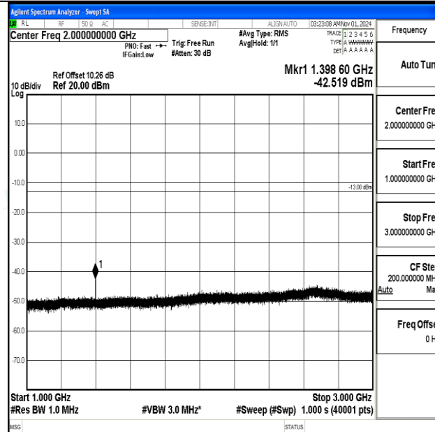
Band12-1.4MHz-QPSK-23017-1RB#0-1000~3000-PASS
