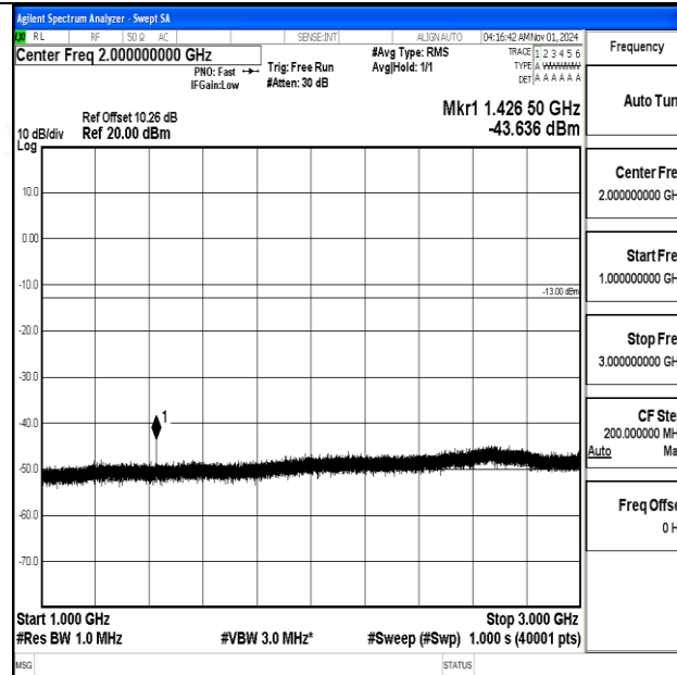
Band12-3MHz-16QAM-23165-1RB#0-1000~3000-PASS
