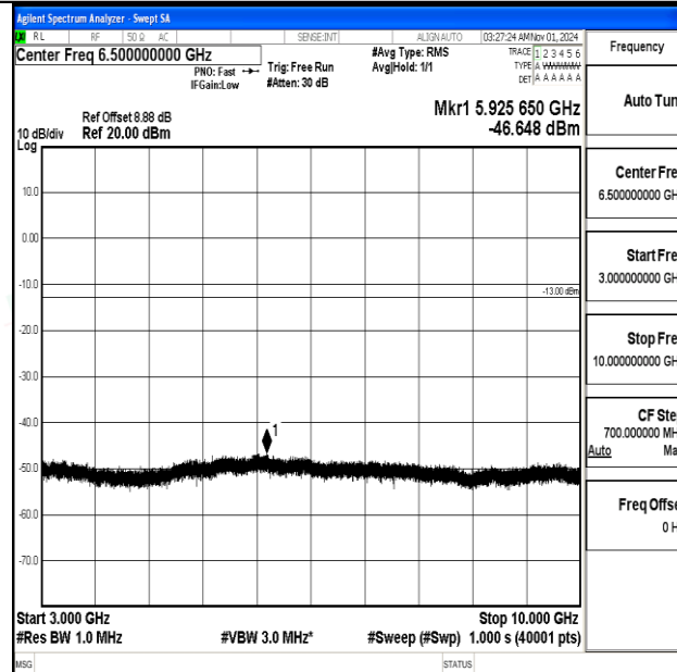
Band12-1.4MHz-16QAM-23173-1RB#0-3000~10000-PASS
