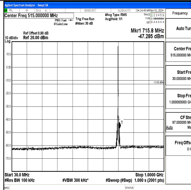
Band12-3MHz-16QAM-23095-1RB#0-30~1000-PASS
