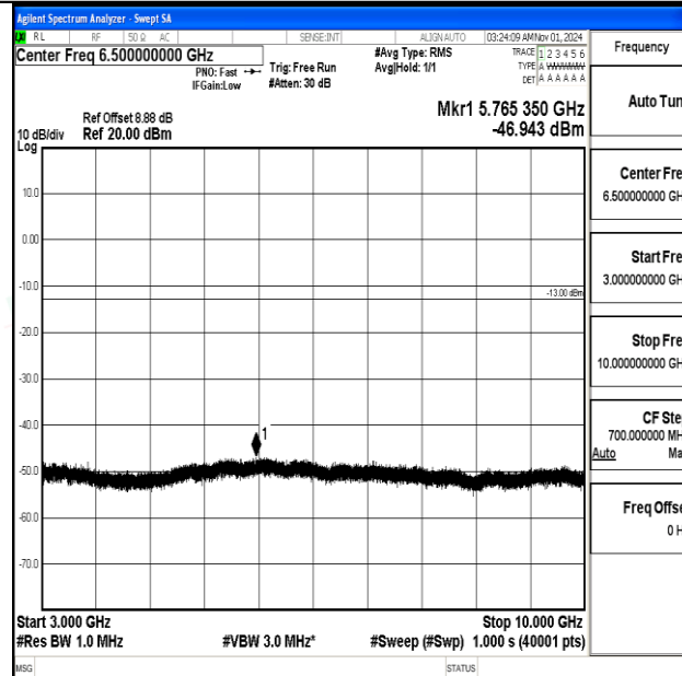
Band12-1.4MHz-16QAM-23017-1RB#0-3000~10000-PASS
