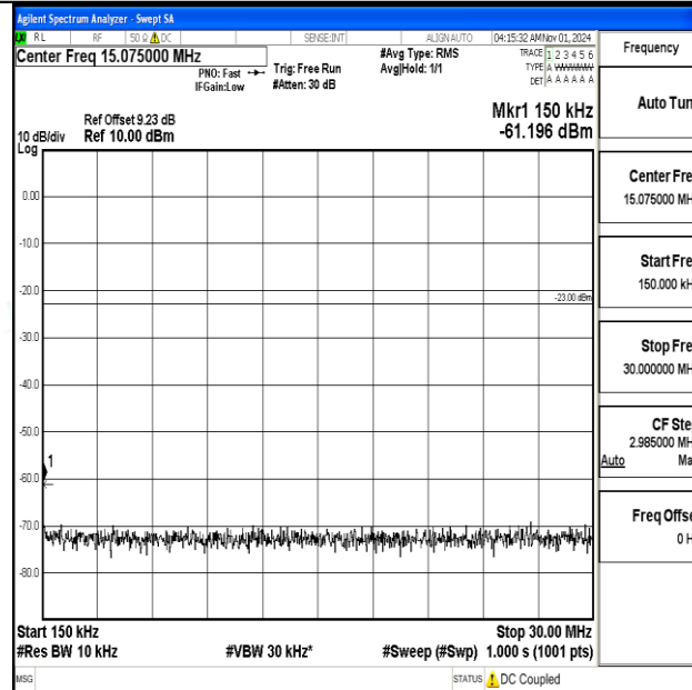
Band12-3MHz-QPSK-23165-1RB#0-0.15~30-PASS
