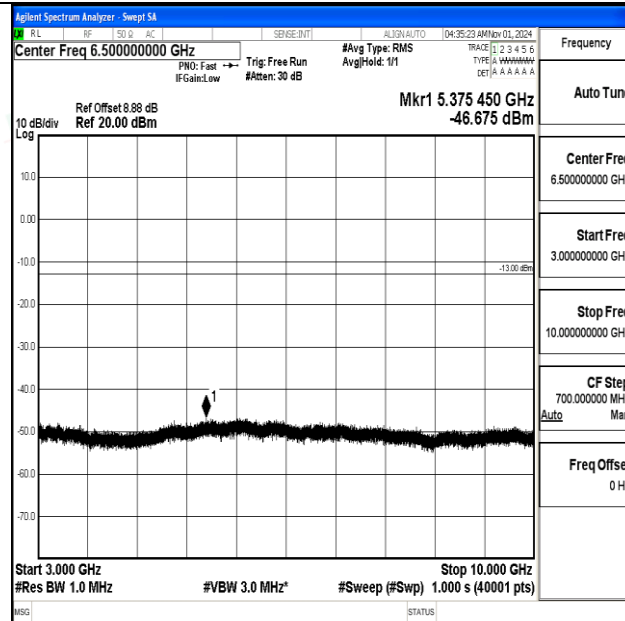
Band12-5MHz-QPSK-23155-1RB#0-3000~10000-PASS
