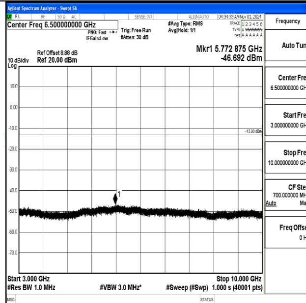
Band12-5MHz-16QAM-23095-1RB#0-3000~10000-PASS
