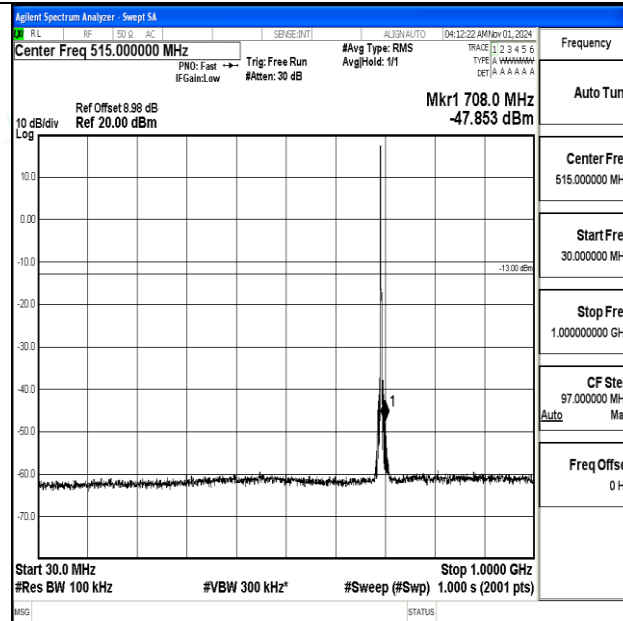
Band12-3MHz-QPSK-23025-1RB#0-30~1000-PASS
