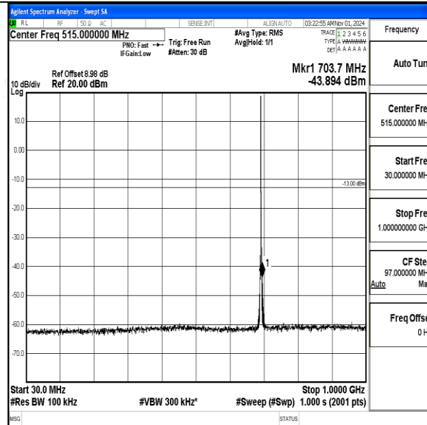
Band12-1.4MHz-QPSK-23017-1RB#0-30~1000-PASS
