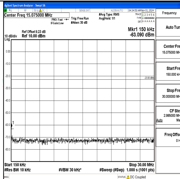
Band12-5MHz-QPSK-23155-1RB#0-0.15~30-PASS
