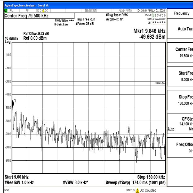
Band12-5MHz-QPSK-23155-1RB#0-0.009~0.15-PASS
