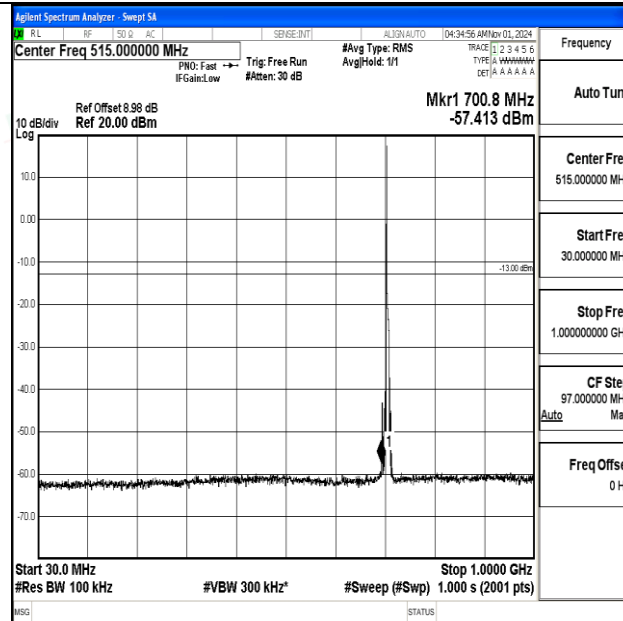
Band12-5MHz-QPSK-23155-1RB#0-30~1000-PASS
