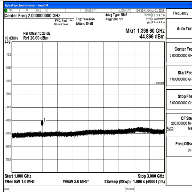
Band12-5MHz-16QAM-23035-1RB#0-1000~3000-PASS
