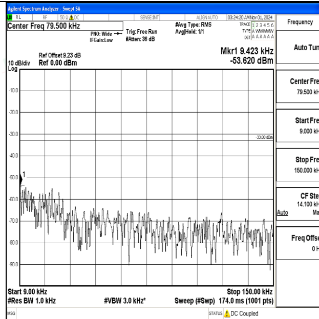
Band12-1.4MHz-QPSK-23095-1RB#0-0.009~0.15-PASS
