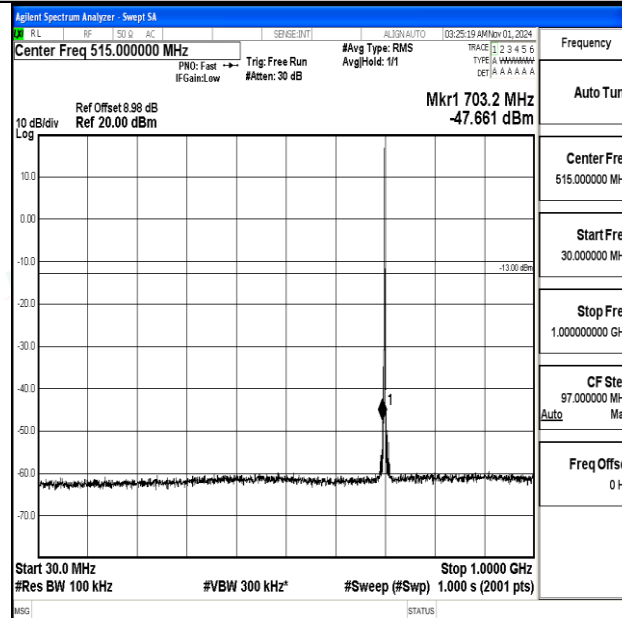
Band12-1.4MHz-16QAM-23095-1RB#0-30~1000-PASS
