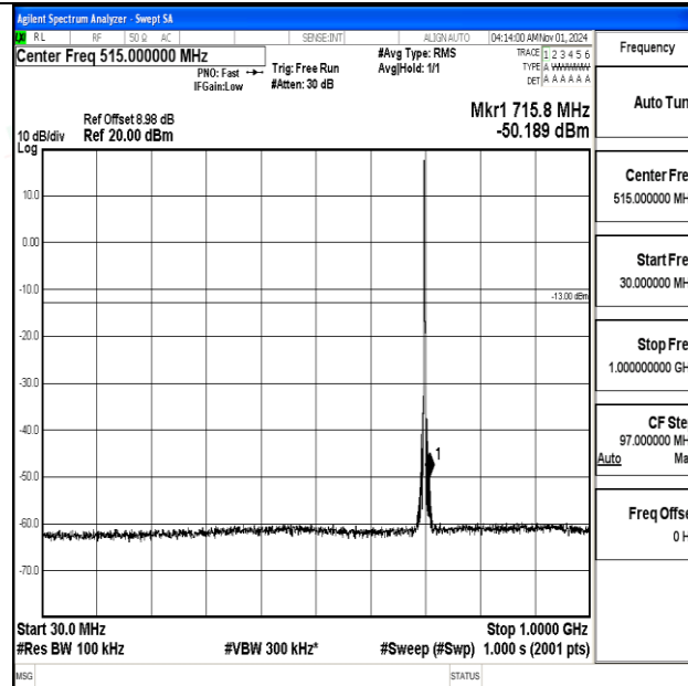
Band12-3MHz-QPSK-23095-1RB#0-30~1000-PASS
