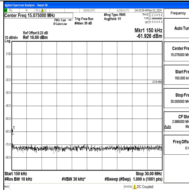
Band12-5MHz-16QAM-23095-1RB#0-0.15~30-PASS
