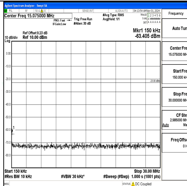
Band12-3MHz-QPSK-23095-1RB#0-0.15~30-PASS
