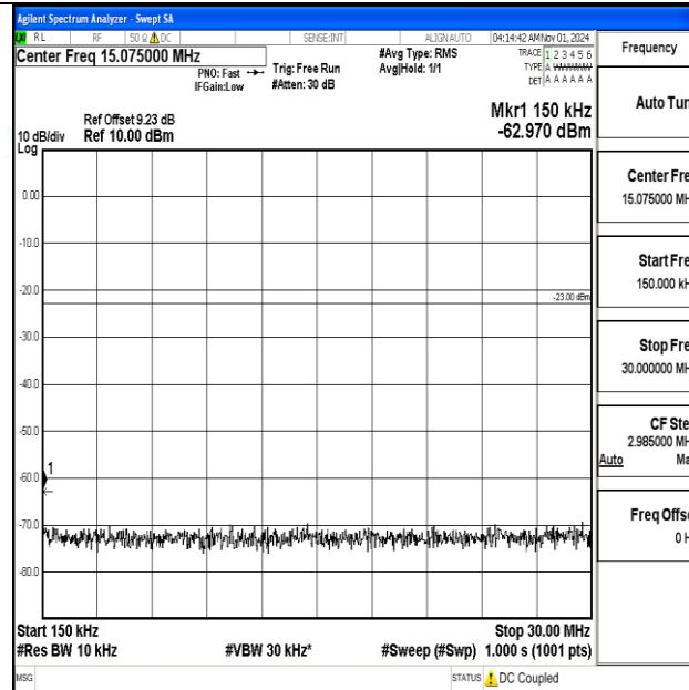
Band12-3MHz-16QAM-23095-1RB#0-0.15~30-PASS
