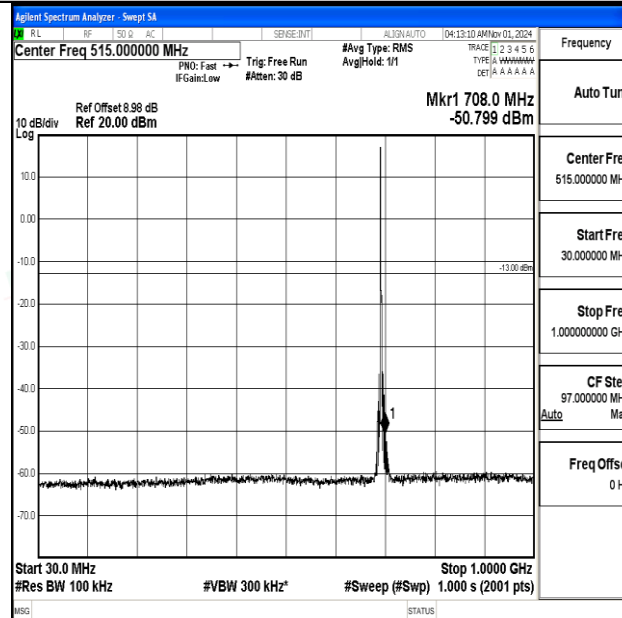
Band12-3MHz-16QAM-23025-1RB#0-30~1000-PASS
