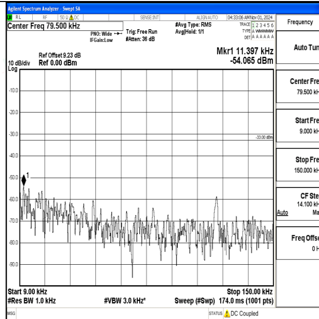
Band12-5MHz-QPSK-23095-1RB#0-0.009~0.15-PASS
