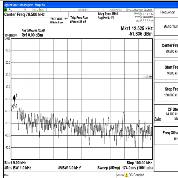
Band12-5MHz-QPSK-23035-1RB#0-0.009~0.15-PASS
