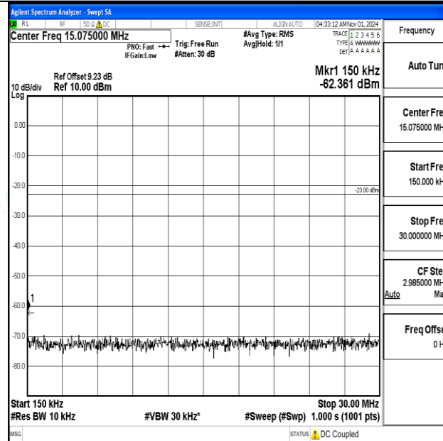
Band12-5MHz-QPSK-23095-1RB#0-0.15~30-PASS
