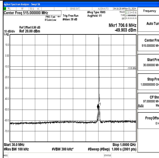
Band12-3MHz-16QAM-23165-1RB#0-30~1000-PASS
