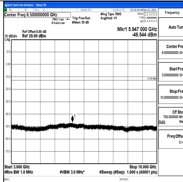
Band12-1.4MHz-QPSK-23173-1RB#0-3000~10000-PASS
