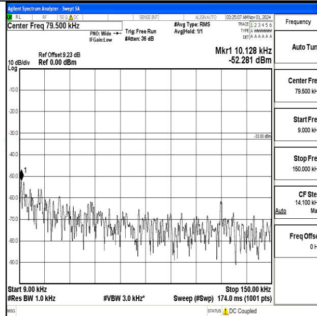
Band12-1.4MHz-16QAM-23095-1RB#0-0.009~0.15-PASS
