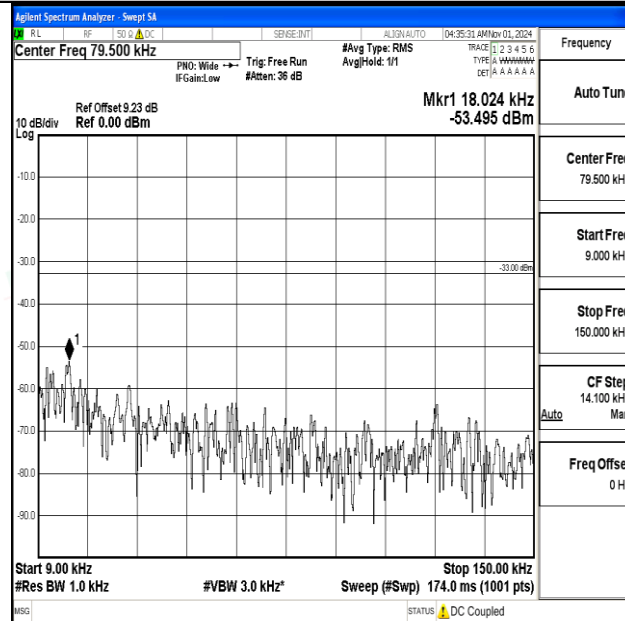
Band12-5MHz-16QAM-23155-1RB#0-0.009~0.15-PASS
