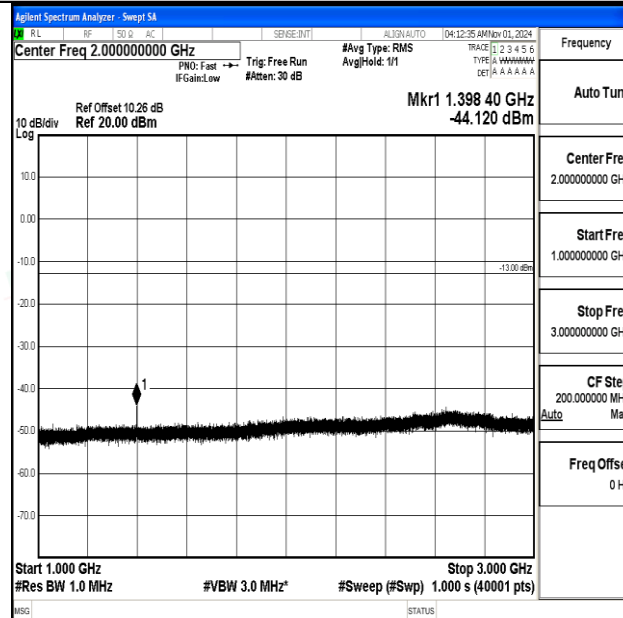
Band12-3MHz-QPSK-23025-1RB#0-1000~3000-PASS
