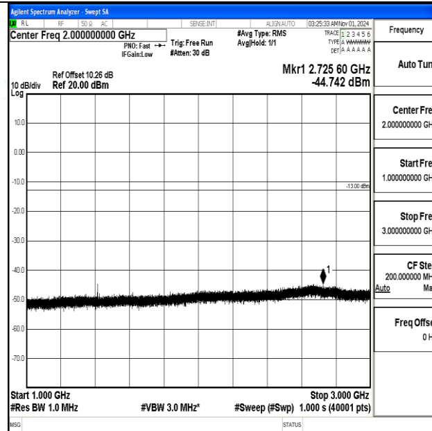
Band12-1.4MHz-16QAM-23095-1RB#0-1000~3000-PASS
