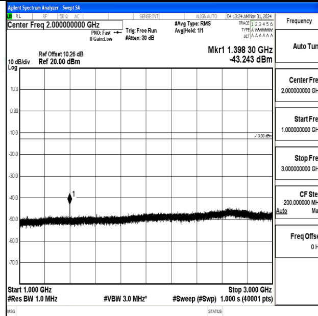
Band12-3MHz-16QAM-23025-1RB#0-1000~3000-PASS
