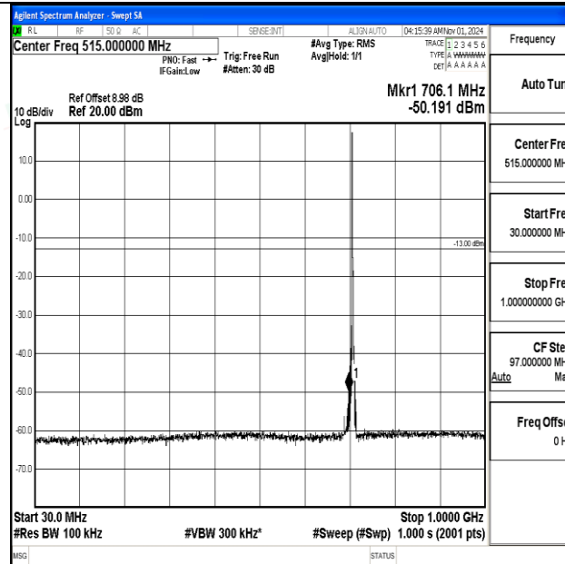
Band12-3MHz-QPSK-23165-1RB#0-30~1000-PASS
