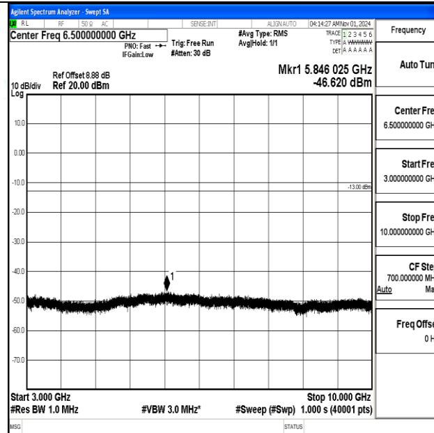
Band12-3MHz-QPSK-23095-1RB#0-3000~10000-PASS
