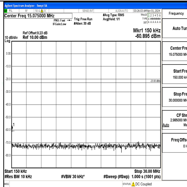
Band12-1.4MHz-QPSK-23173-1RB#0-0.15~30-PASS
