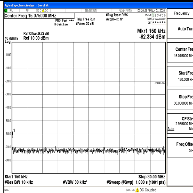
Band12-1.4MHz-QPSK-23095-1RB#0-0.15~30-PASS
