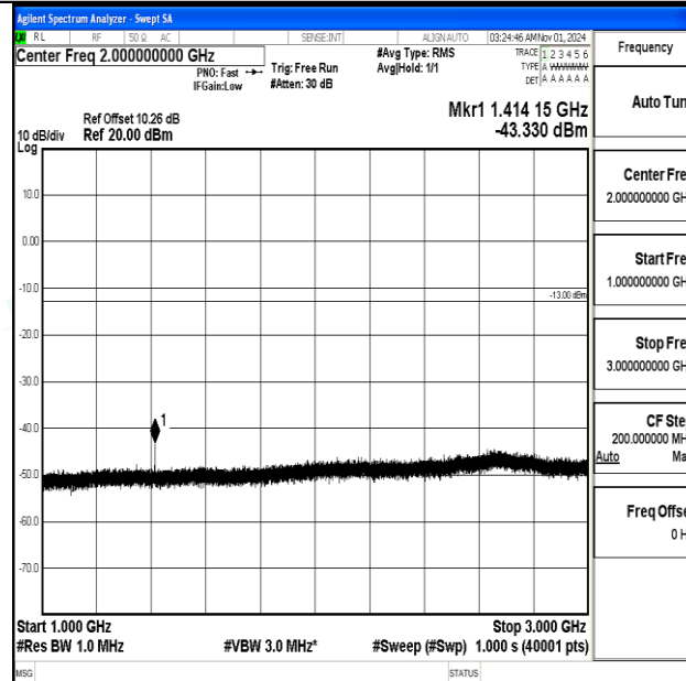
Band12-1.4MHz-QPSK-23095-1RB#0-1000~3000-PASS
