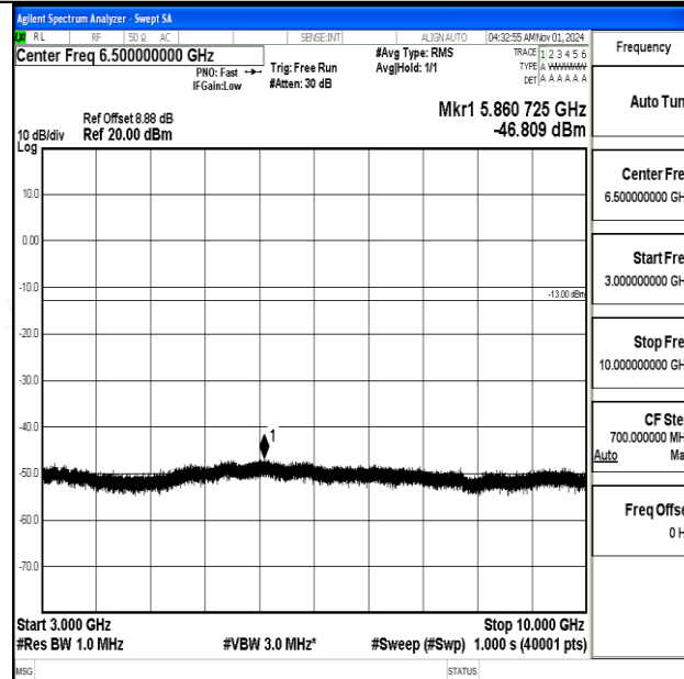
Band12-5MHz-16QAM-23035-1RB#0-3000~10000-PASS
