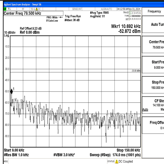
Band12-3MHz-16QAM-23025-1RB#0-0.009~0.15-PASS
