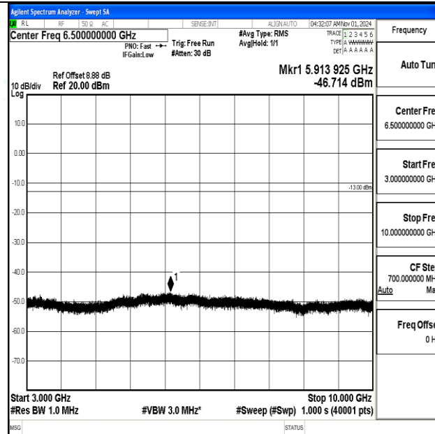
Band12-5MHz-QPSK-23035-1RB#0-3000~10000-PASS
