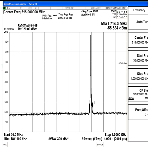
Band12-5MHz-16QAM-23035-1RB#0-30~1000-PASS
