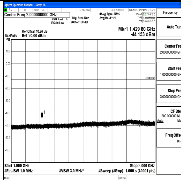
Band12-1.4MHz-QPSK-23173-1RB#0-1000~3000-PASS
