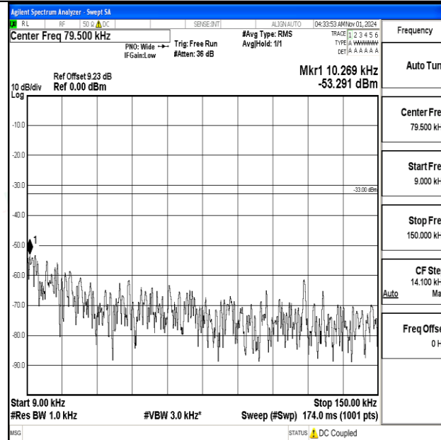
Band12-5MHz-16QAM-23095-1RB#0-0.009~0.15-PASS
