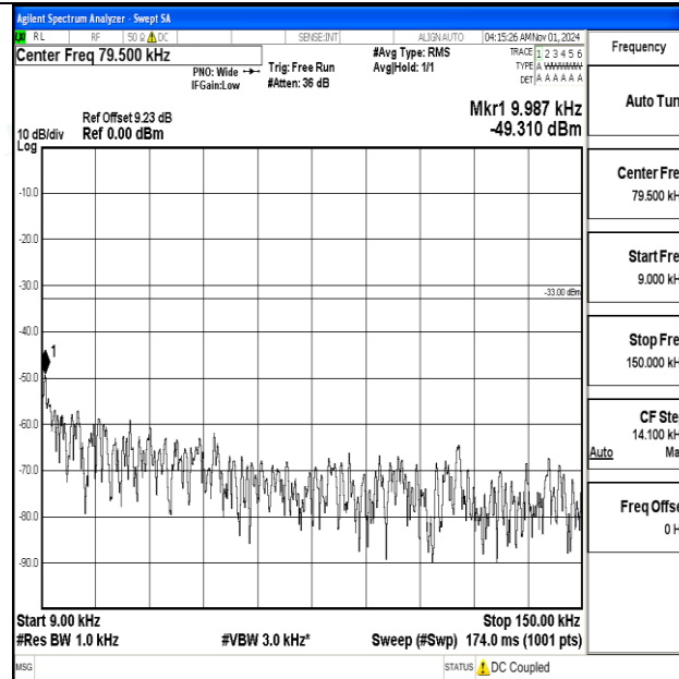
Band12-3MHz-QPSK-23165-1RB#0-0.009~0.15-PASS
