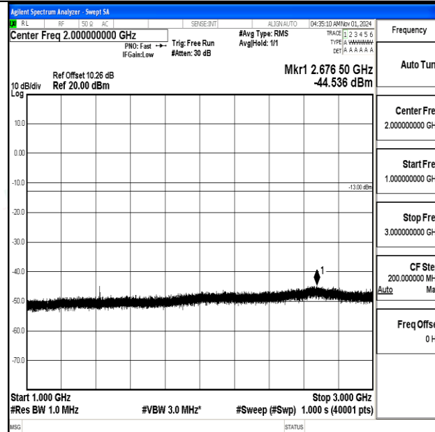
Band12-5MHz-QPSK-23155-1RB#0-1000~3000-PASS
