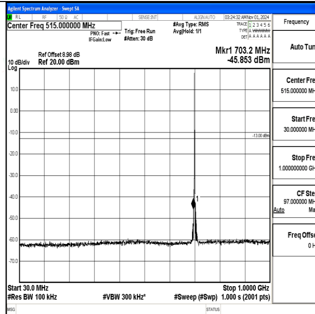
Band12-1.4MHz-QPSK-23095-1RB#0-30~1000-PASS
