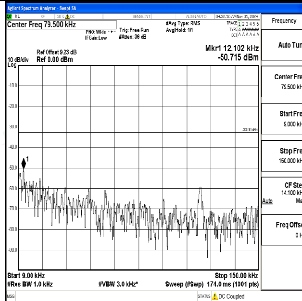
Band12-5MHz-16QAM-23035-1RB#0-0.009~0.15-PASS
