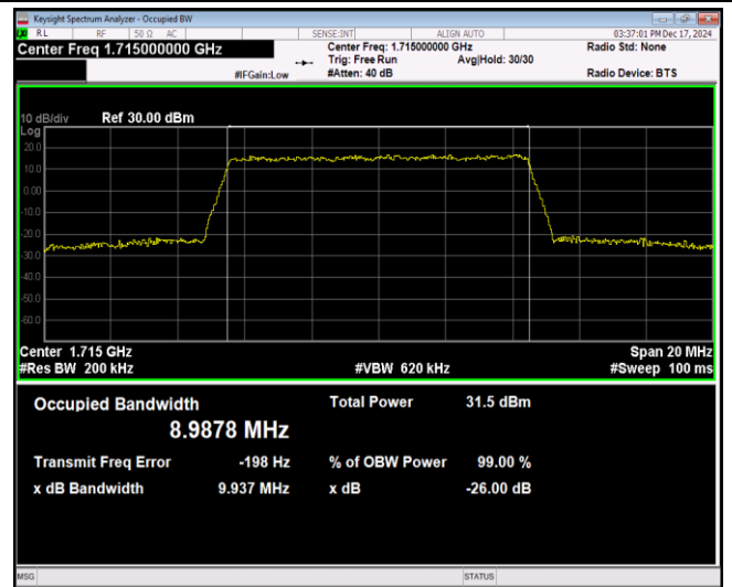
Band4-10MHz-16QAM-20350-50RB#0
