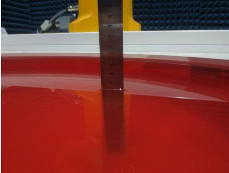
Fig. 9.1 Photo of Liquid Height for Body SAR of ELI V5.0 (2000MHz~2600MHz) (depth>15cm)
