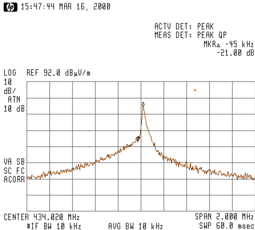
Figure 11. Fundamental Emission
