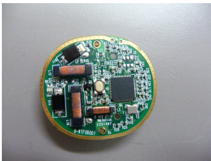
Photograph 7.4.1 Antenna assembly
