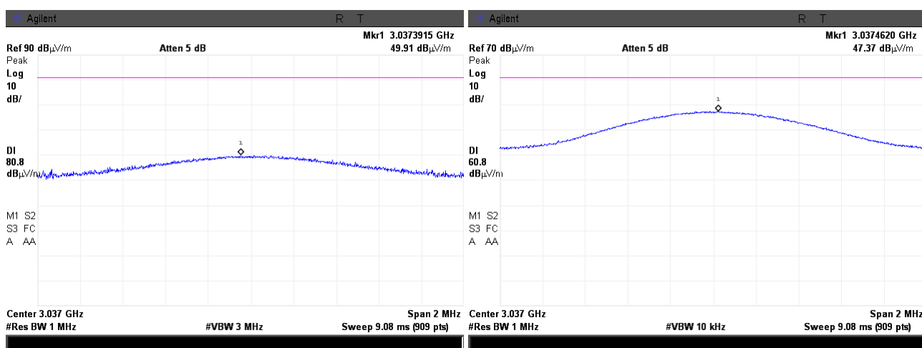
Plot 7.2.18 Radiated emission measurements at the seventh harmonic frequency
