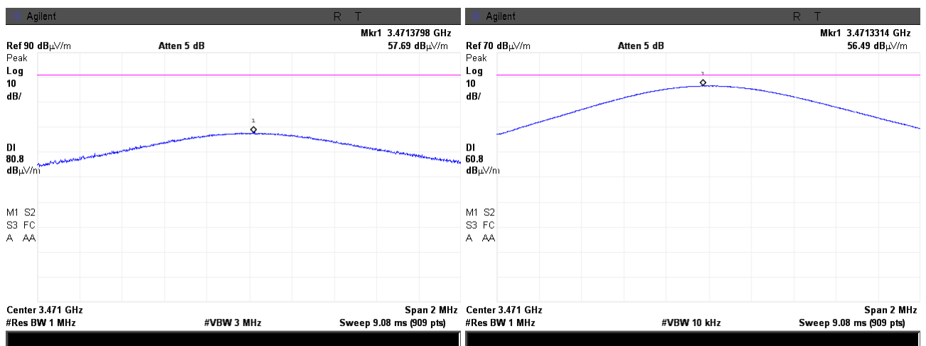
Plot 7.2.20 Radiated emission measurements at the eighth harmonic frequency
