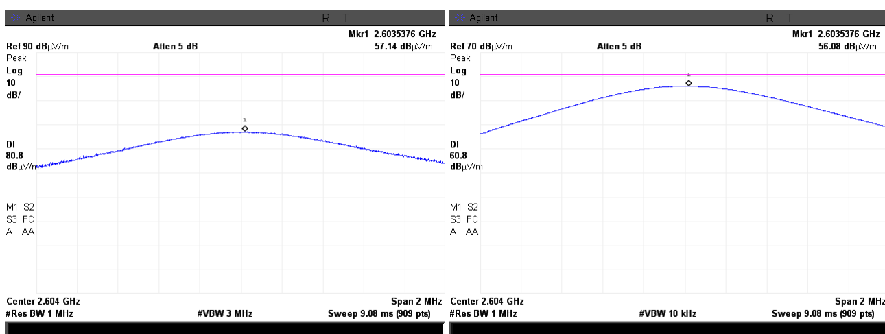
Plot 7.2.16 Radiated emission measurements at the sixth harmonic frequency
