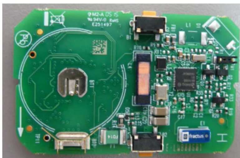
Photograph 7.6.1 Antenna assembly
