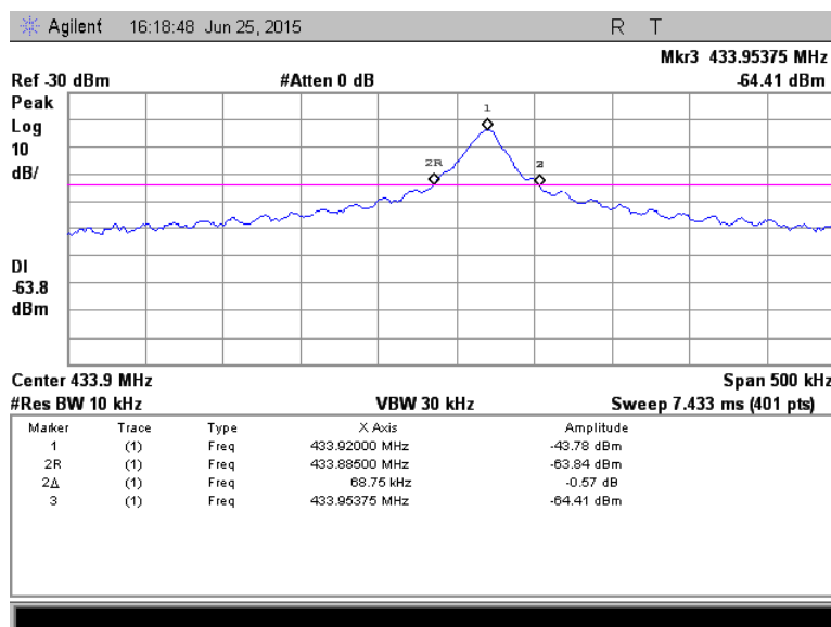
Plot 7.3.2 Occupied bandwidth test result, 99% power
