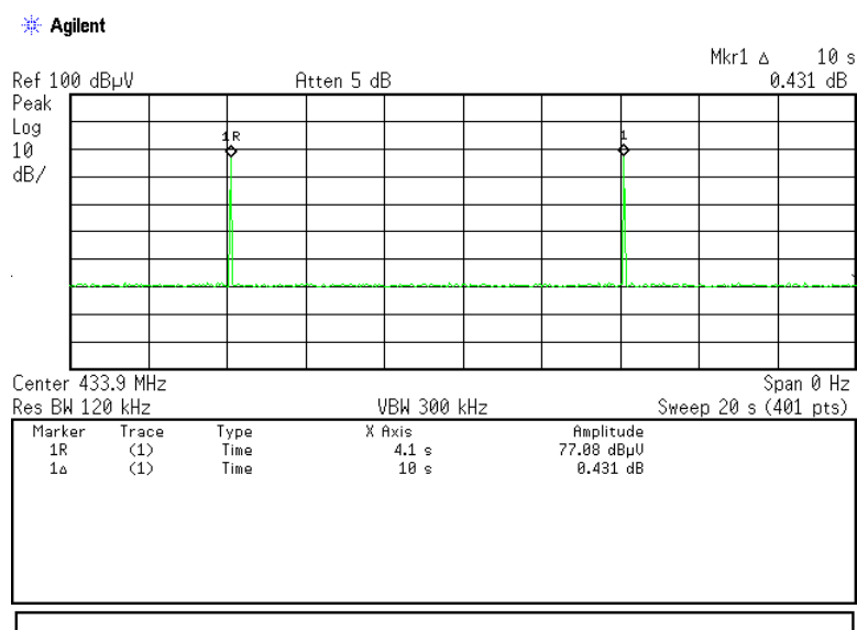
Plot 7.2.14 Transmission pulse period
