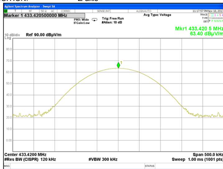
Plot 7.2.6 Radiated emission measurements at the fundamental frequency
