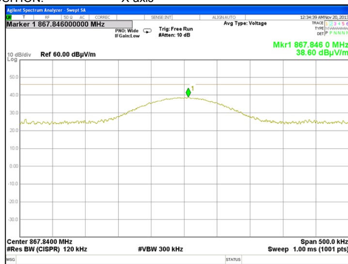
Plot 7.3.8 Radiated emission measurements at the second harmonic frequency
