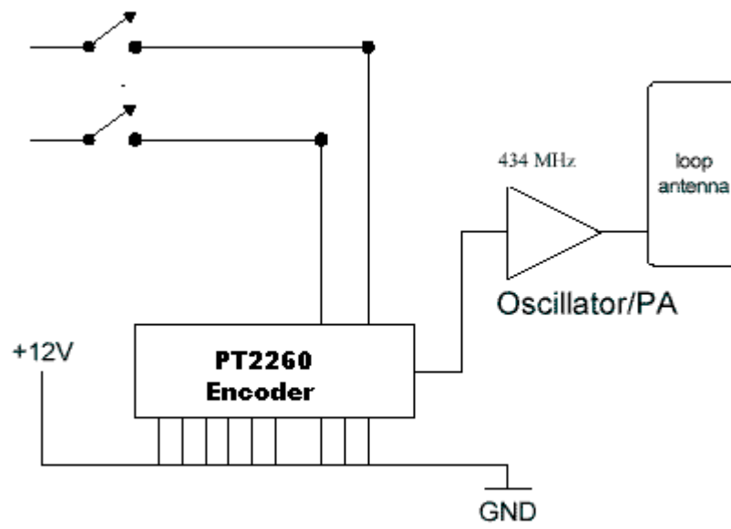
BLOCK DIAGRAM
