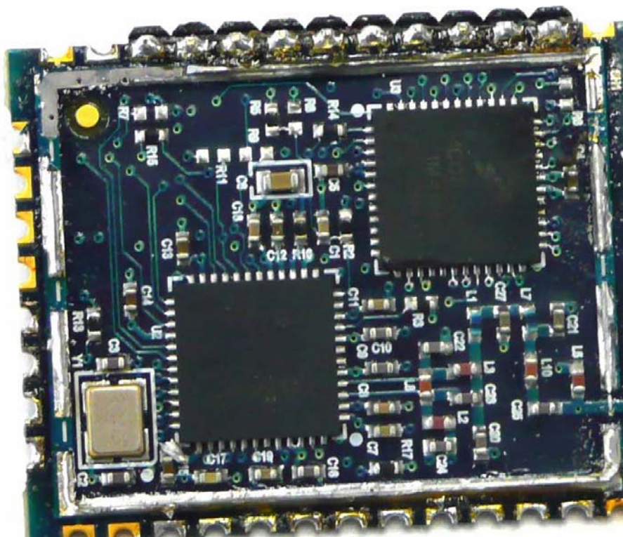
EUT-RF Shielding Cover Removed
