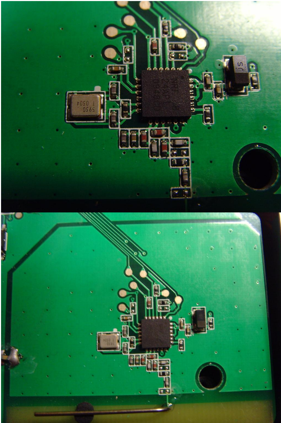
RF part
