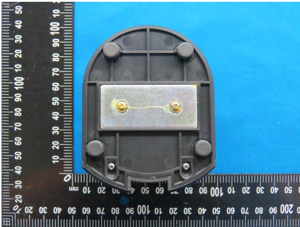
Charging stand - Bottom View
