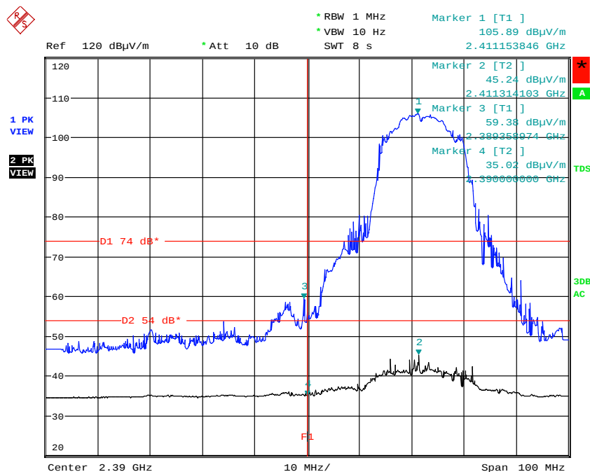
Figure 45: Radiated Emissions at Band Edge, Spectral Diagram, Host FM1S, AC 120V Input Voltage, Mode A (2412MHz)
