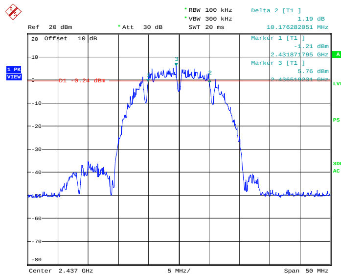
Figure 10: 6dB Bandwidth, Antenna 1, Mode B (2437MHz)
