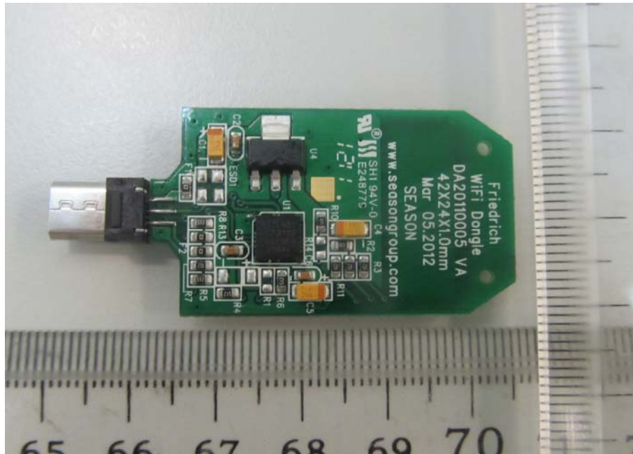
PCB of EUT
