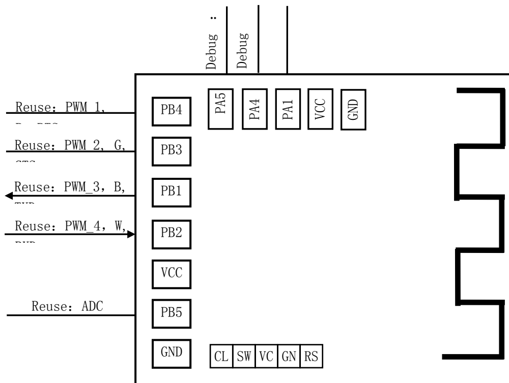
Picture 3-6. Support 4 lines of PWM output
