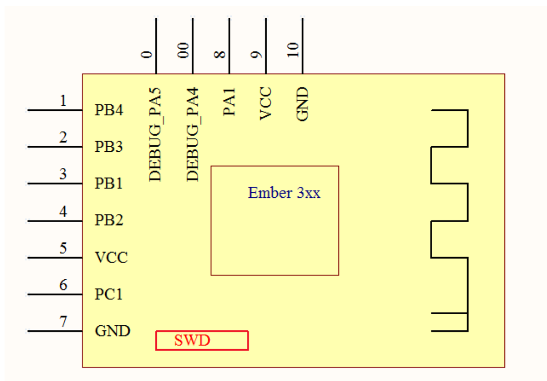
Picture 3-9. Pin Configuration
