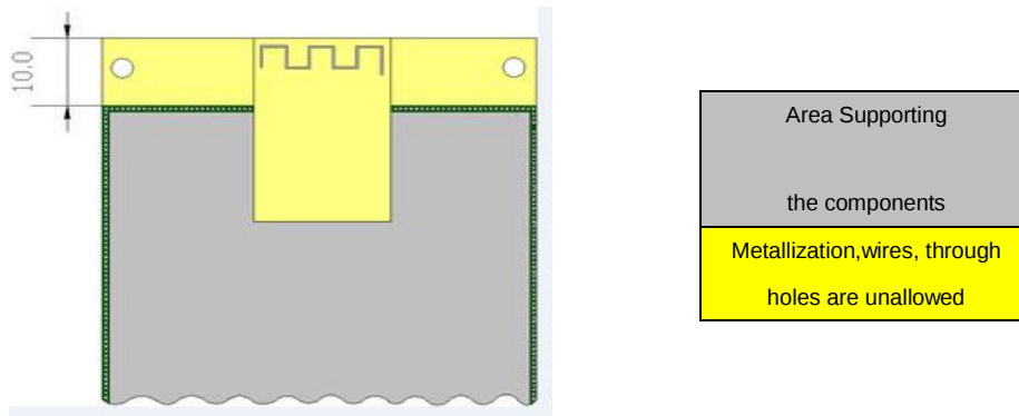
Picture 3-12. PCB antenna location drawing
