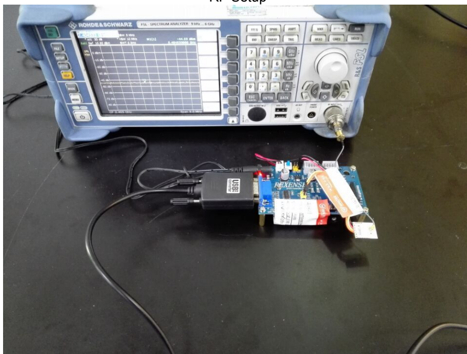
RF Setup
