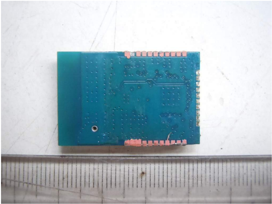
FIGURE 1 802.15.4 / ZIGBEE MODULE (M/N: REX3SP) MAIN BOARD (BACK VIEW)
