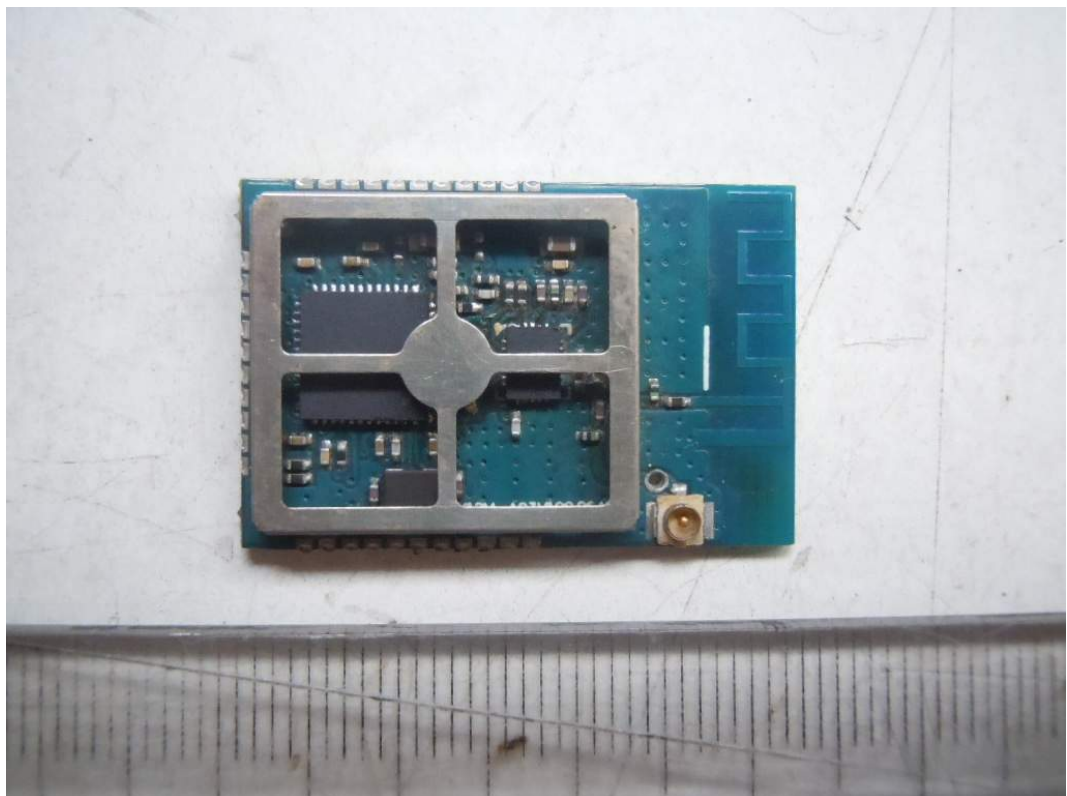
FIGURE 4 802.15.4 / ZIGBEE MODULE (M/N: REX3SP) MAIN BOARD (FRONT VIEW)
