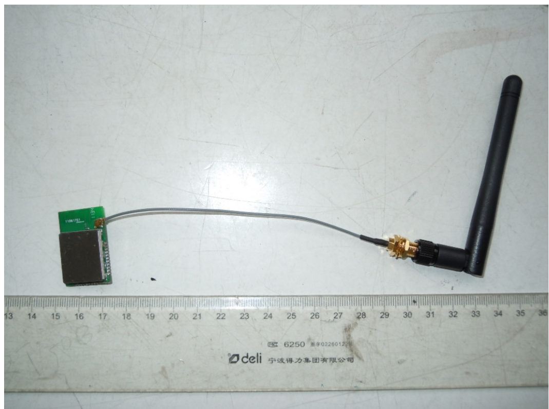
FIGURE 2 802.15.4 / ZIGBEE MODULE (M/N: REX3) GENERAL APPEARANCE WITH SMA ANTENNA
