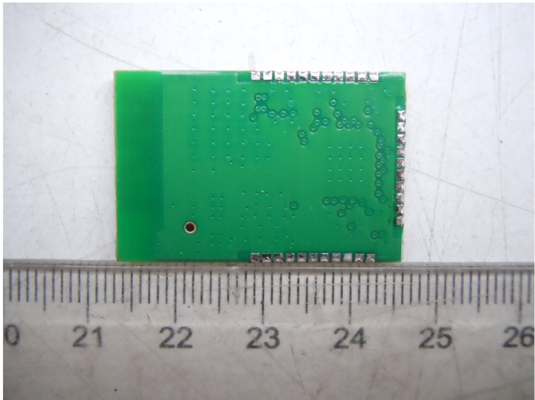
FIGURE 1 802.15.4 / ZIGBEE MODULE (M/N: REX3) MAIN BOARD (BACK VIEW)
