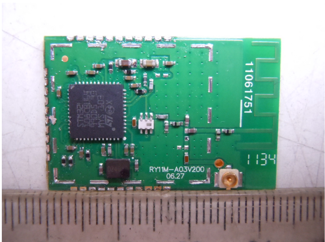
FIGURE 4 802.15.4 / ZIGBEE MODULE (M/N: REX3) MAIN BOARD (FRONT VIEW)
