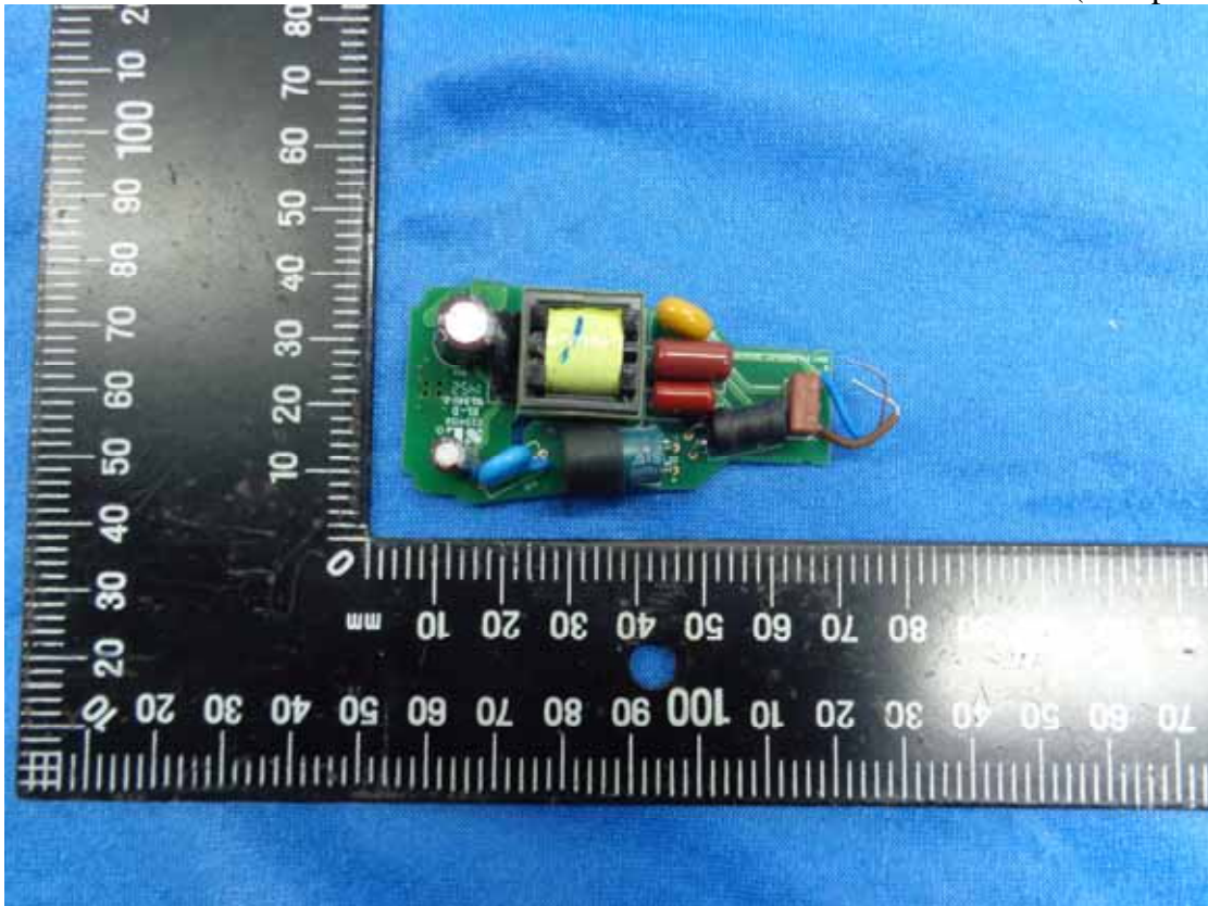
Figure 11 Power Board (Component Side)
