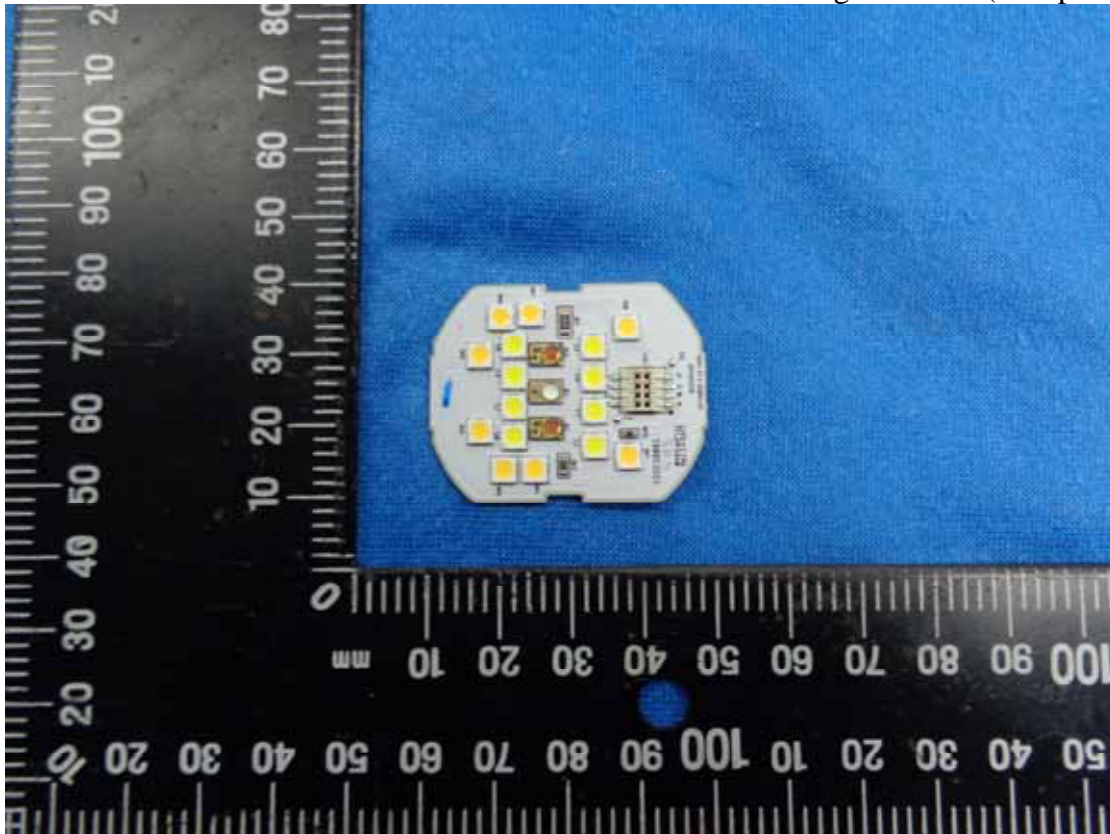
Figure 9 LED Light Board (Component Side)
