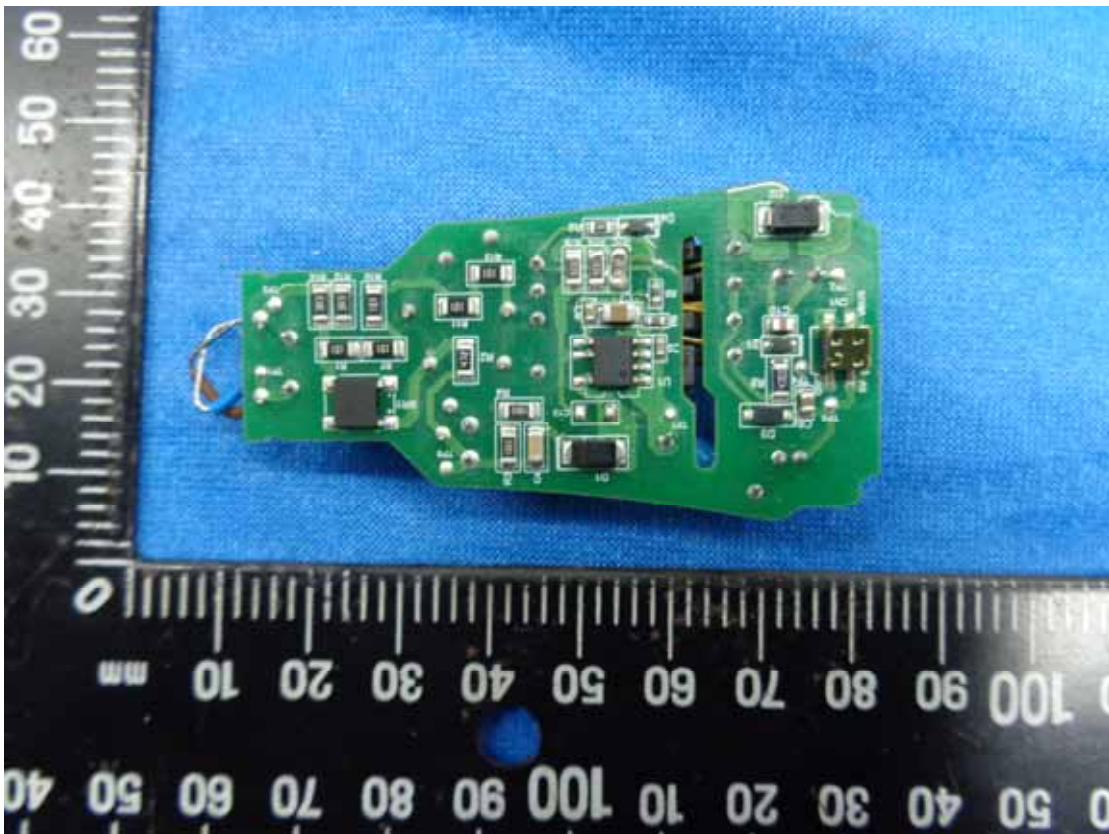
Figure 12 Power Board (Solder Side)
