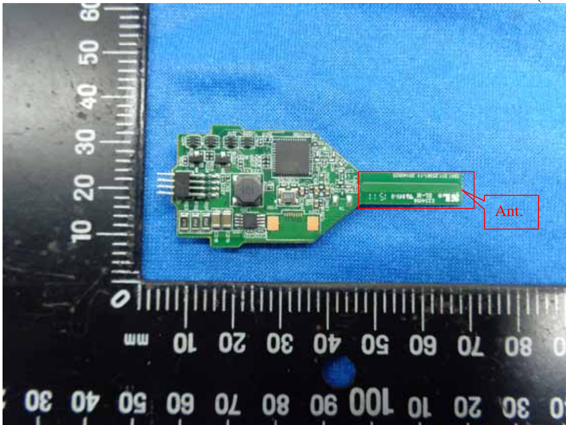
Figure 14 PCB Board (Solder Side)
