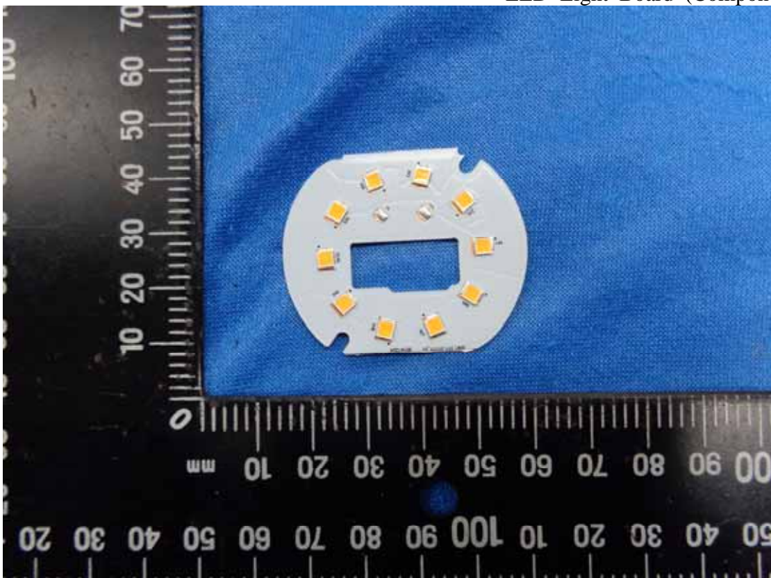
Figure 2 LED Light Board (Component Side)
