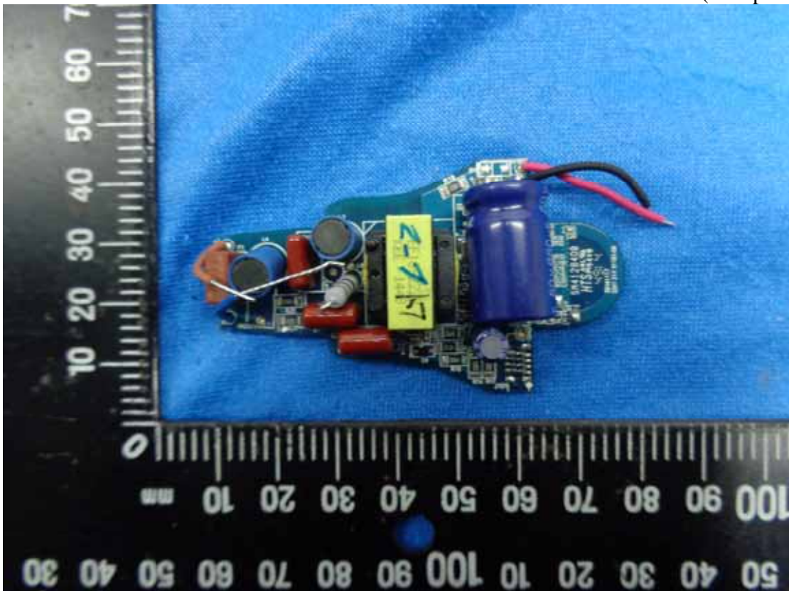
Figure 4 Power Board (Component Side)
