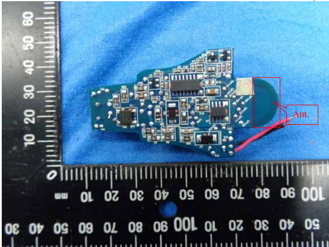
Figure 5 Power Board (Solder Side)
