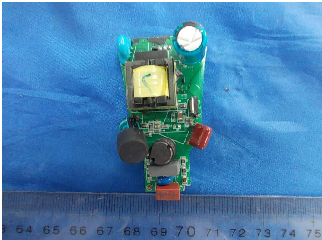
FIGURE 2 LED LAMPS (M/N: 9290002265) LED DRIVER (FRONT VIEW)
