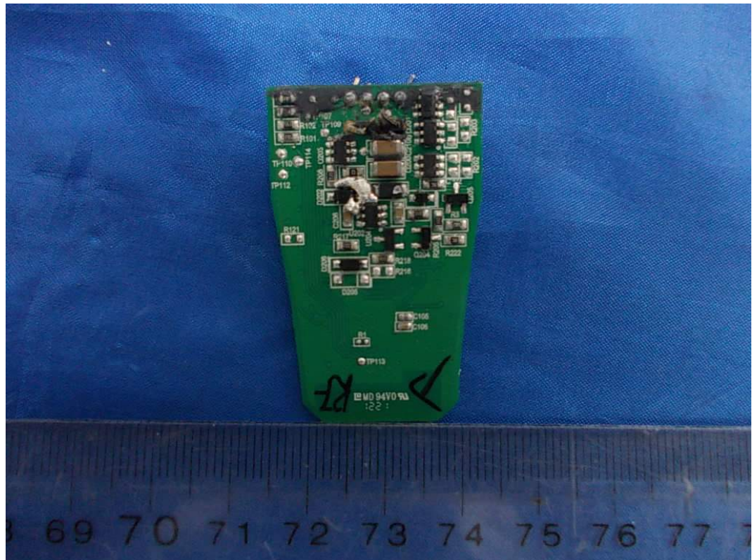
FIGURE 6 LED LAMPS (M/N: 9290002265) RF BOARD (FRONT VIEW)
