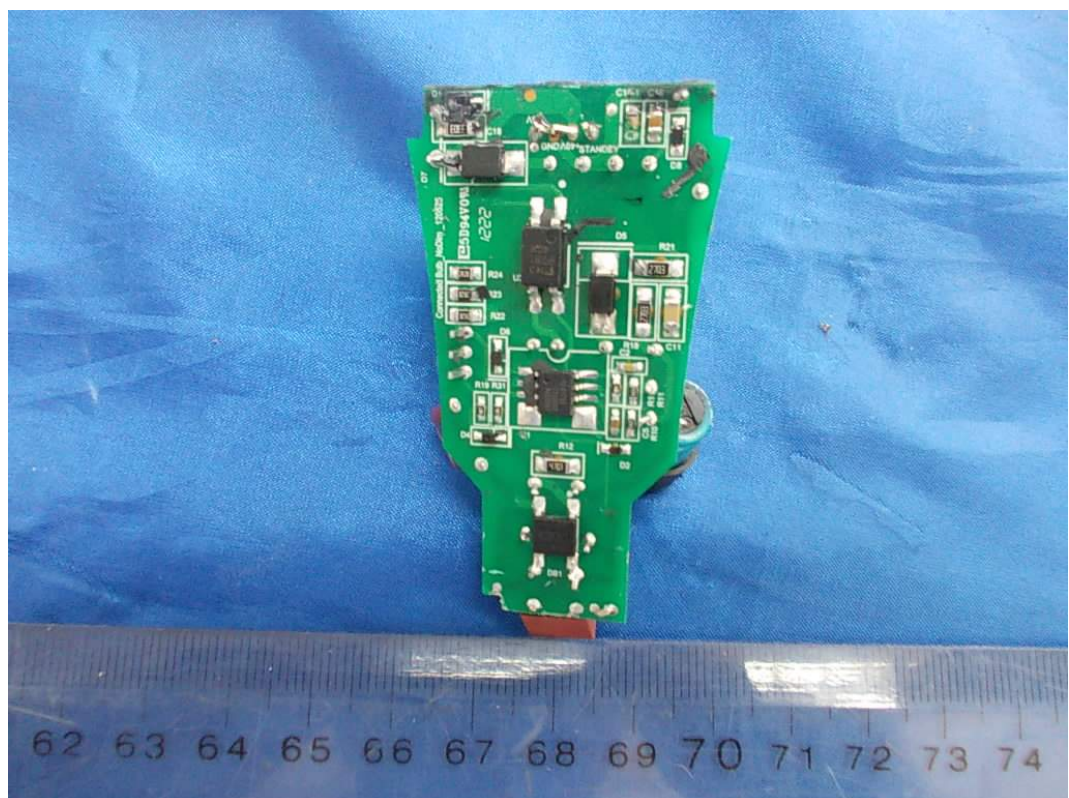
FIGURE 3 LED LAMPS (M/N: 9290002265) LED DRIVER (BACK VIEW)
