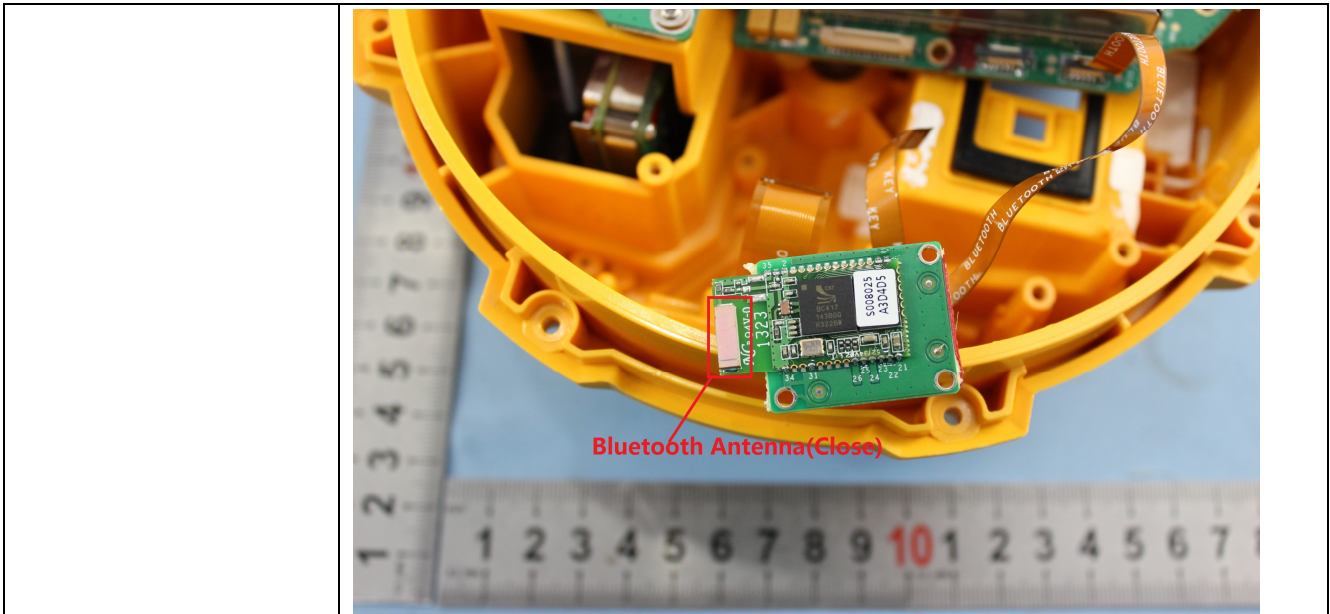
The antenna is integrated on the main PCB and no consideration of replacement. The best case gain of the antenna is 2dBi.
