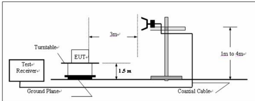
TEST SETUP ABOVE 1GHZ
