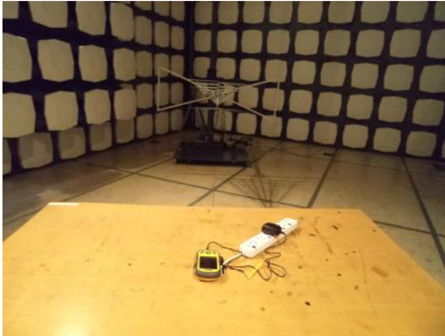
FCC RADIATED EMISSION TEST SETUP-Charging
