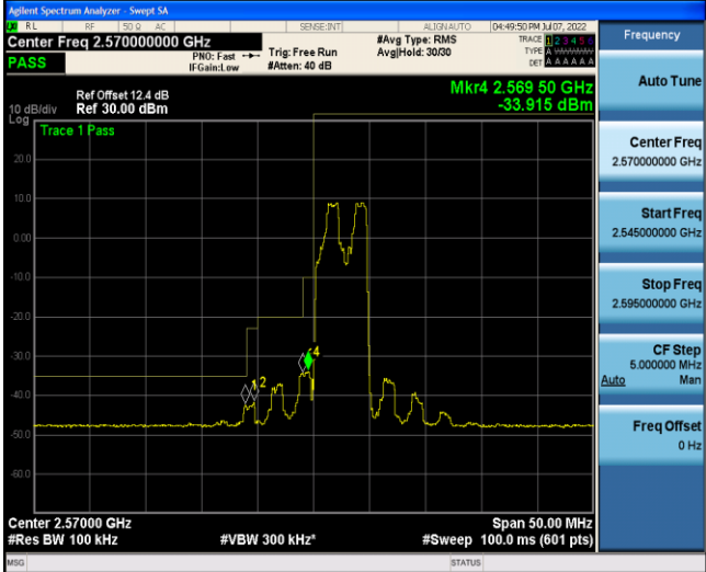
Band38-5MHz-16QAM-37775-25RB#0
