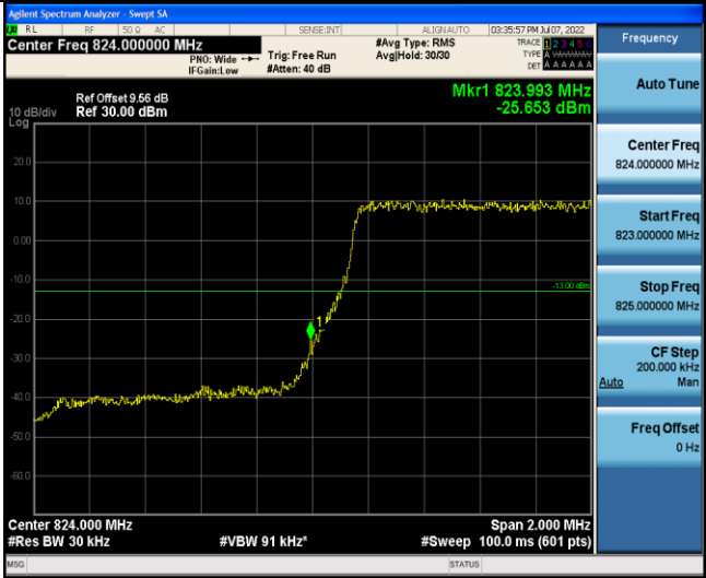
Band5-1.4MHz-QPSK-20643-6RB#0
