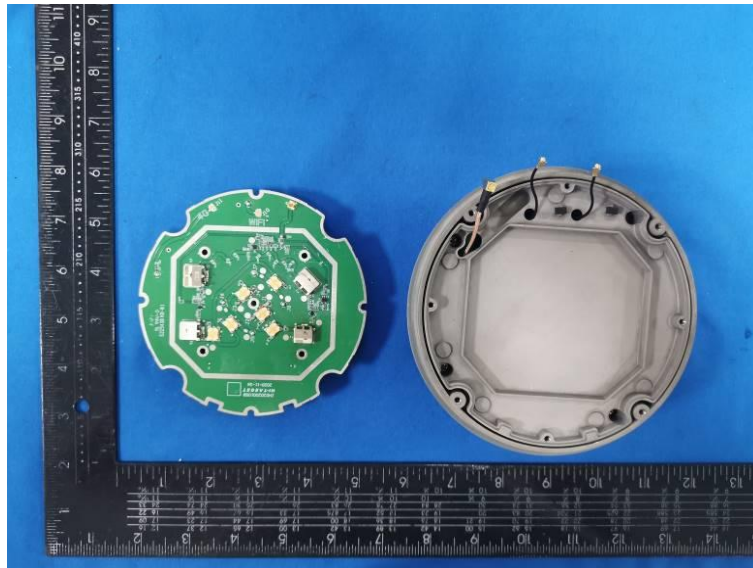
Disc combination antenna(BT/GPS/WIFI/LTE)
