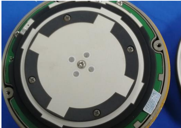
Disc combination antenna
