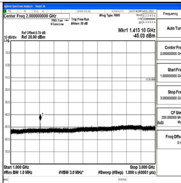
Band17_10MHz_16QAM_23800_1RB#0_1000~3000_1000~3000
