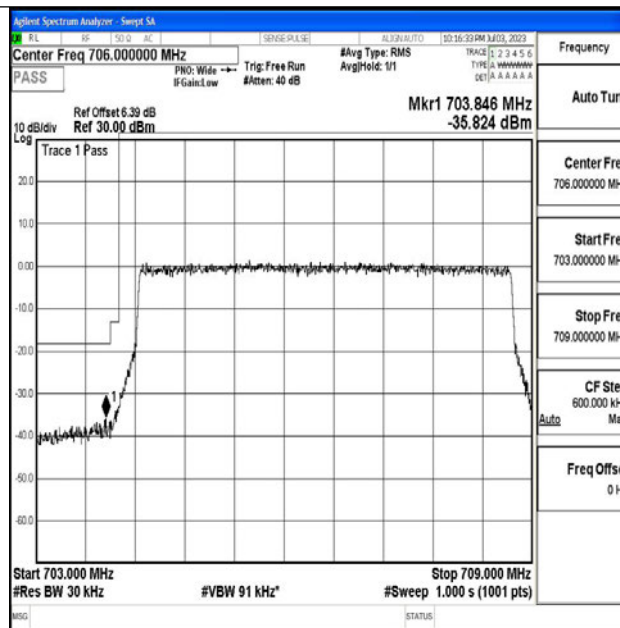
Band17_5MHz_16QAM_23755_25RB#0
