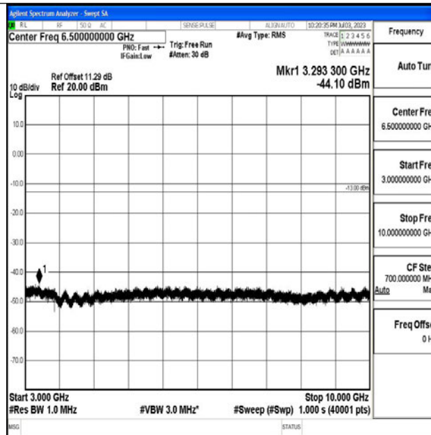
Band17_5MHz_QPSK_23825_1RB#0_3000~10000_3000~10000
