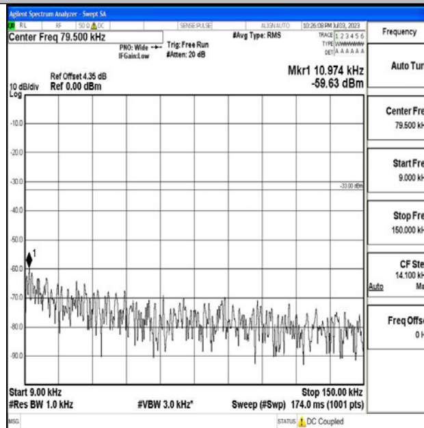
Band17_10MHz_16QAM_23790_1RB#0_0.009~0.15_0.009~0.15
