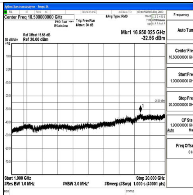
Band7_10MHz_16QAM_21100_1RB#0_1000~20000_1000~20000
