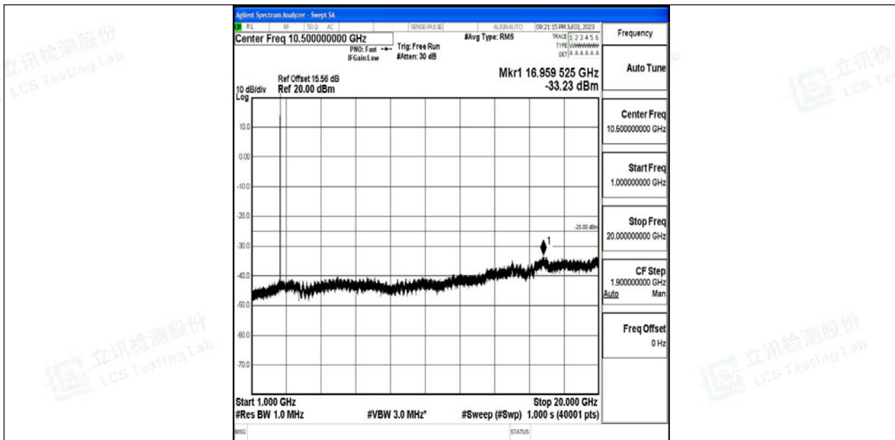
Band7_5MHz_16QAM_21425_1RB#0_1000~20000_1000~20000
