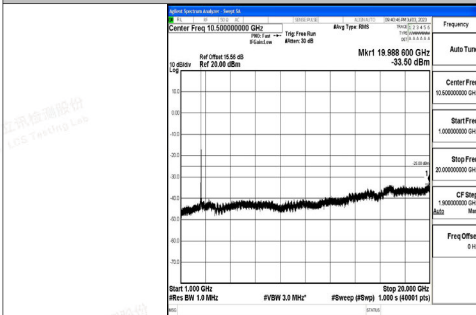
Band7_20MHz_QPSK_21350_1RB#0_1000~20000_1000~20000
