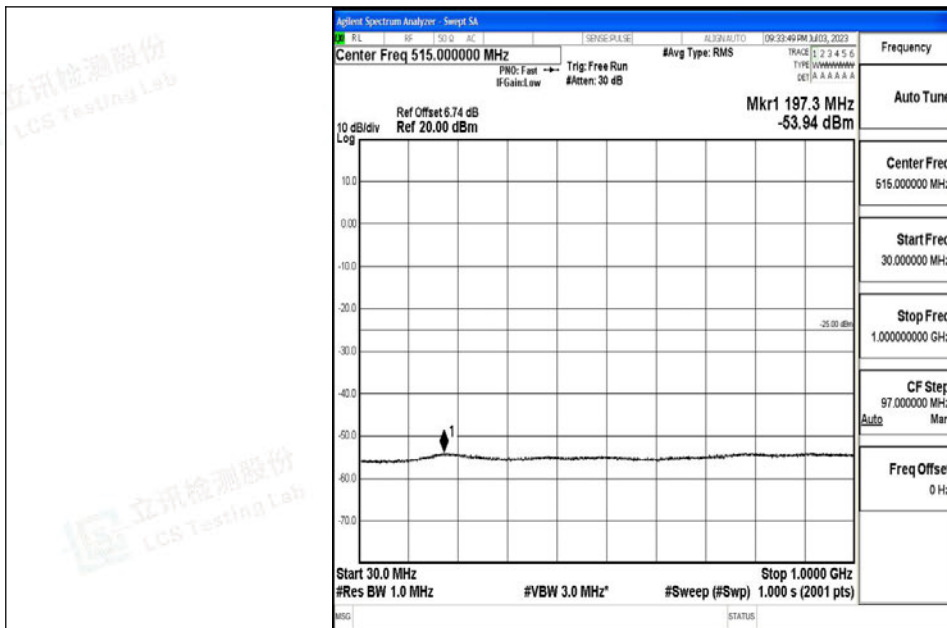
Band7_15MHz_QPSK_21375_1RB#0_30~1000_30~1000
