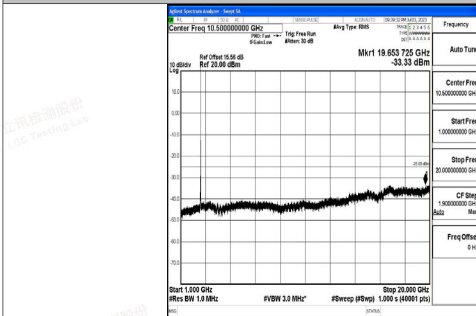
Band7_20MHz_QPSK_21100_1RB#0_1000~20000_1000~20000
