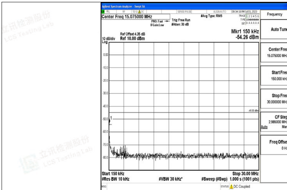
Band7_15MHz_16QAM_21375_1RB#0_0.15~30_0.15~30
