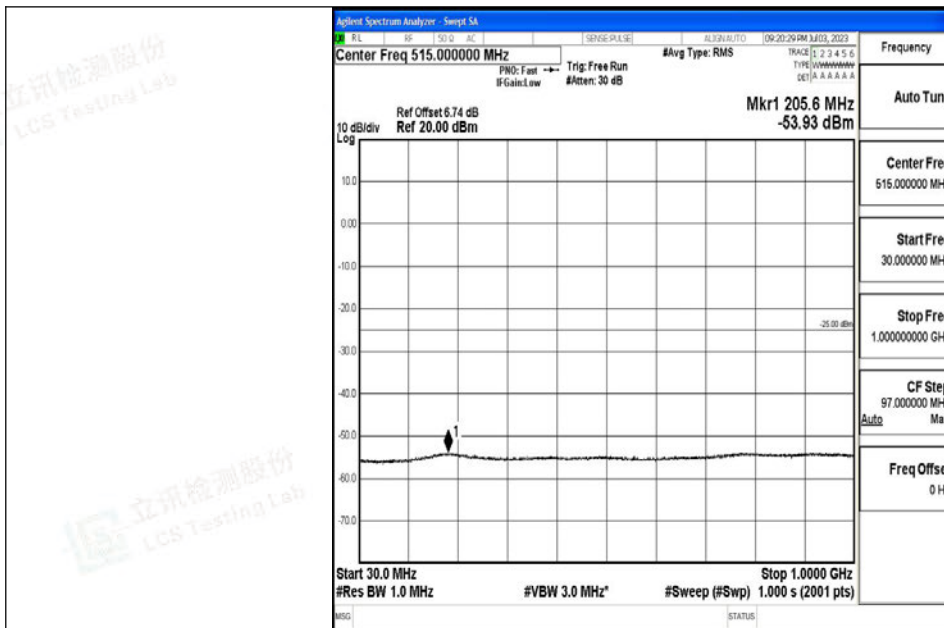
Band7_5MHz_QPSK_21425_1RB#0_30~1000_30~1000
