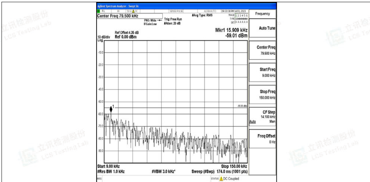
Band7_15MHz_QPSK_21375_1RB#0_0.009~0.15_0.009~0.15
