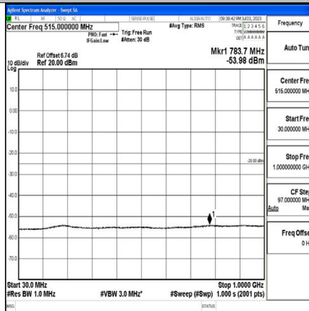
Band7_20MHz_16QAM_20850_1RB#0_30~1000_30~1000
