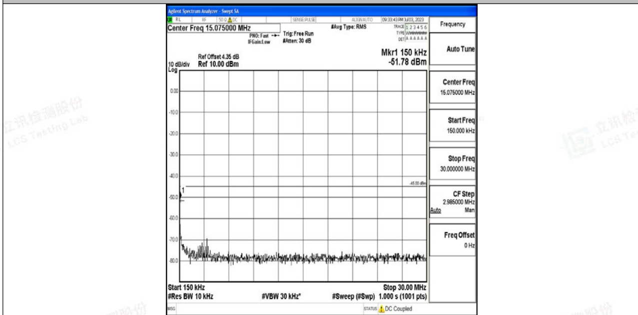
Band7_15MHz_QPSK_21375_1RB#0_0.15~30_0.15~30
