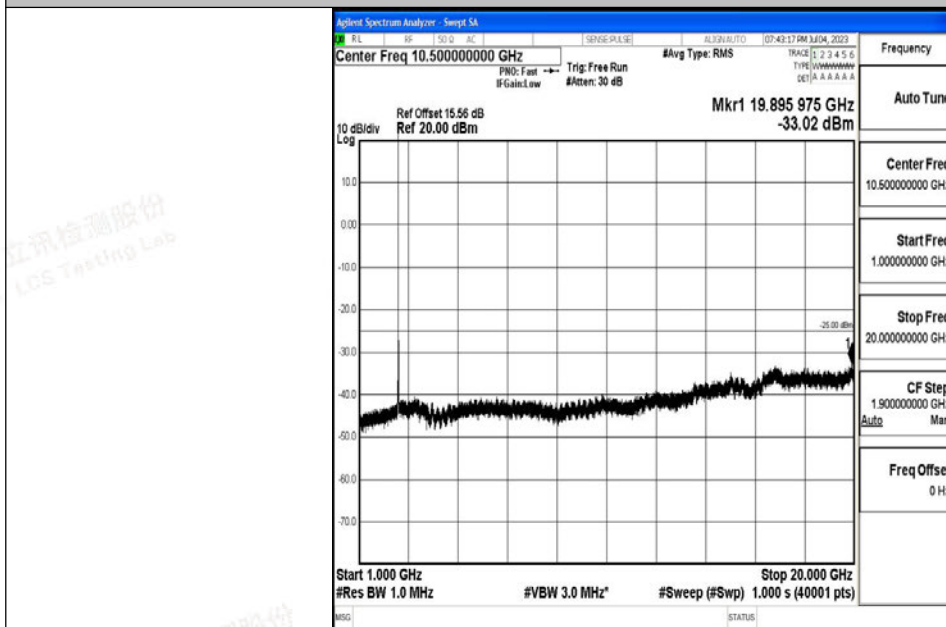
Band7_10MHz_QPSK_20800_1RB#0_1000~20000_1000~20000
