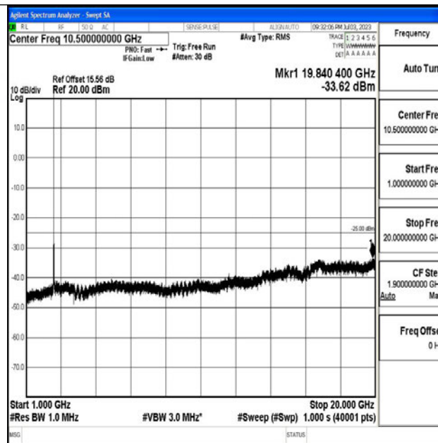
Band7_15MHz_16QAM_20825_1RB#0_1000~20000_1000~20000
