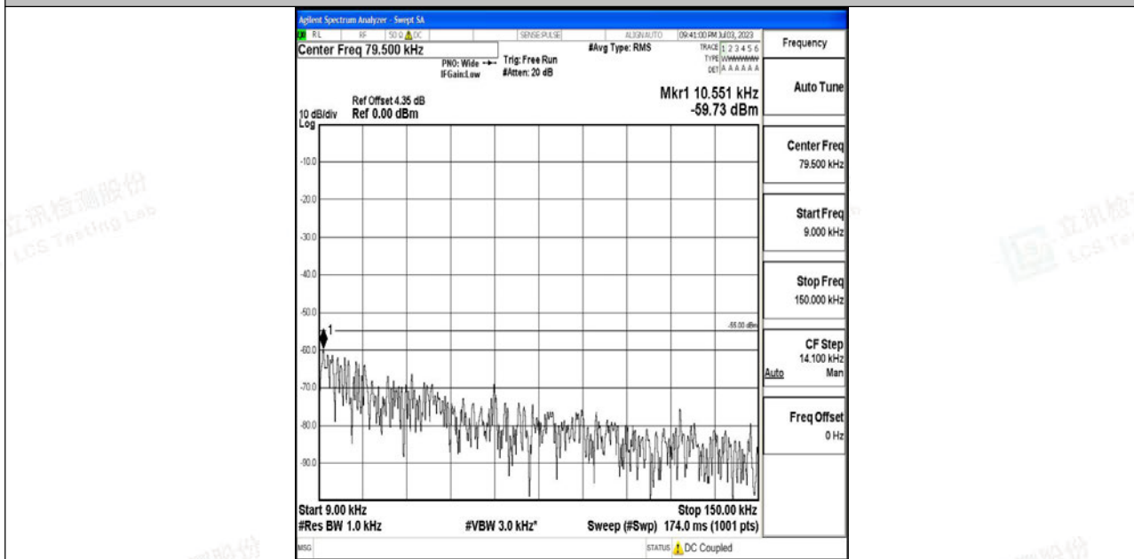
Band7_20MHz_16QAM_21350_1RB#0_0.009~0.15_0.009~0.15
