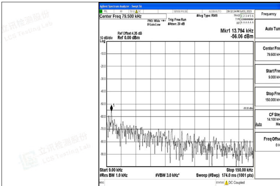
Band7_15MHz_QPSK_21100_1RB#0_0.009~0.15_0.009~0.15
