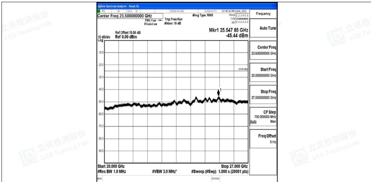
Band7_10MHz_QPSK_21400_1RB#0_20000~27000_20000~27000
