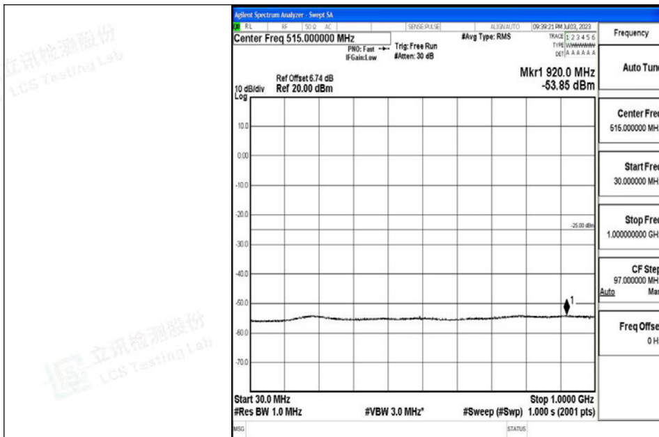
Band7_20MHz_QPSK_21100_1RB#0_30~1000_30~1000
