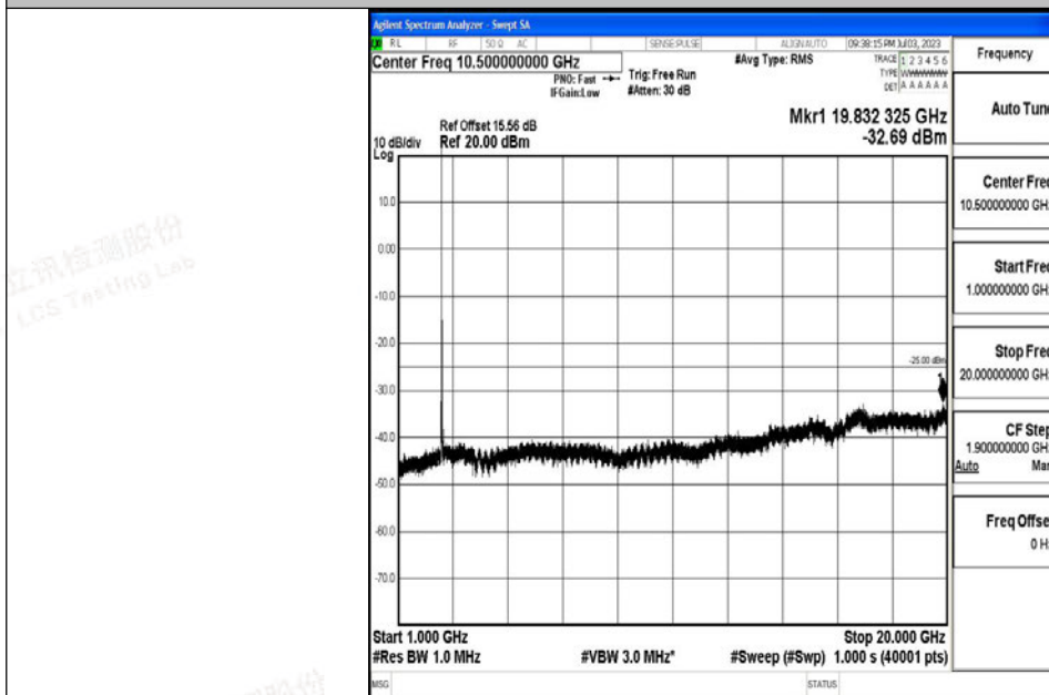
Band7_20MHz_QPSK_20850_1RB#0_1000~20000_1000~20000
