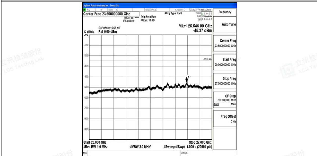
Band7_15MHz_QPSK_20825_1RB#0_20000~27000_20000~27000
