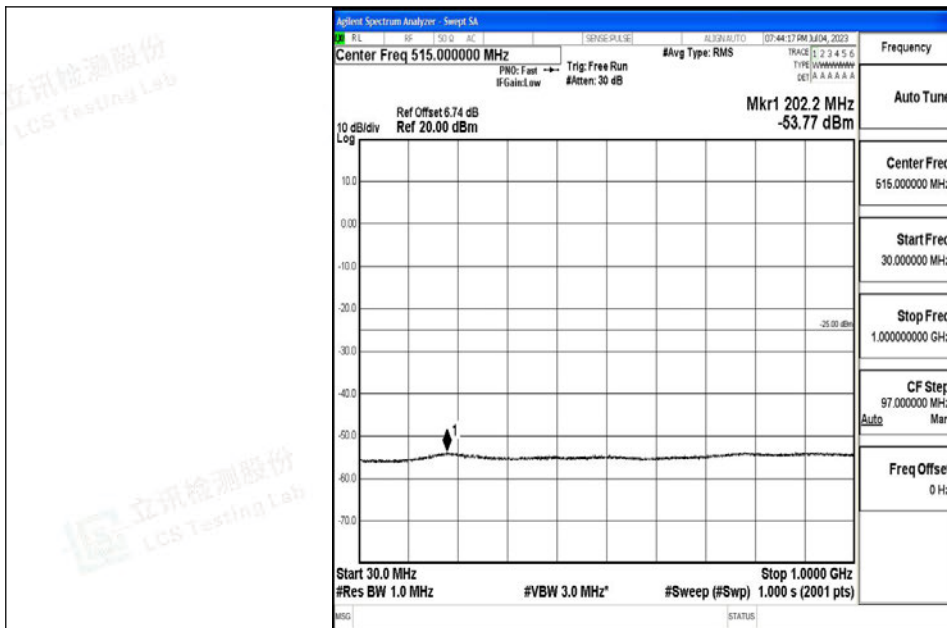
Band7_10MHz_QPSK_21100_1RB#0_30~1000_30~1000
