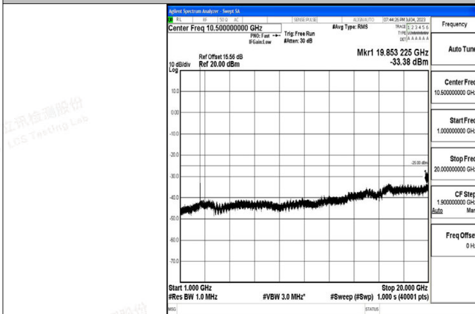
Band7_10MHz_QPSK_21100_1RB#0_1000~20000_1000~20000
