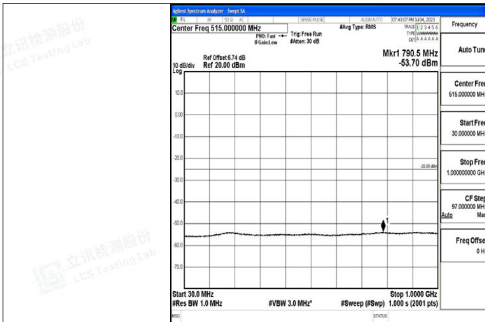
Band7_10MHz_QPSK_20800_1RB#0_30~1000_30~1000
