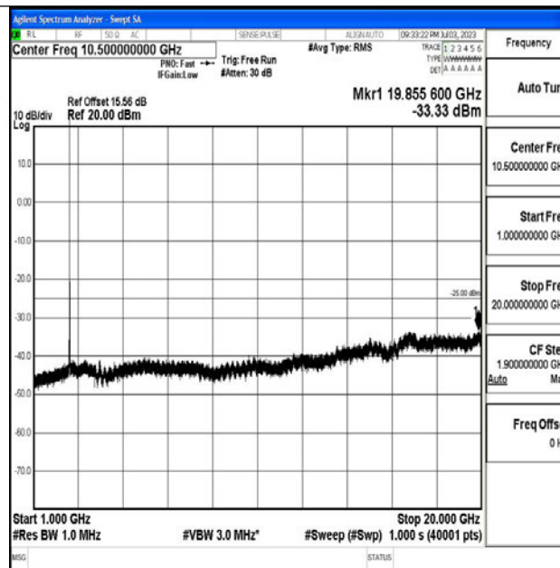
Band7_15MHz_16QAM_21100_1RB#0_1000~20000_1000~20000
