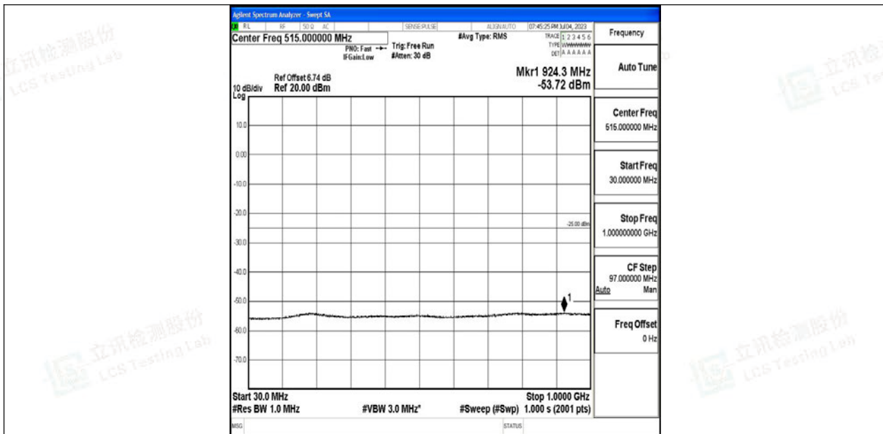
Band7_10MHz_QPSK_21400_1RB#0_30~1000_30~1000
