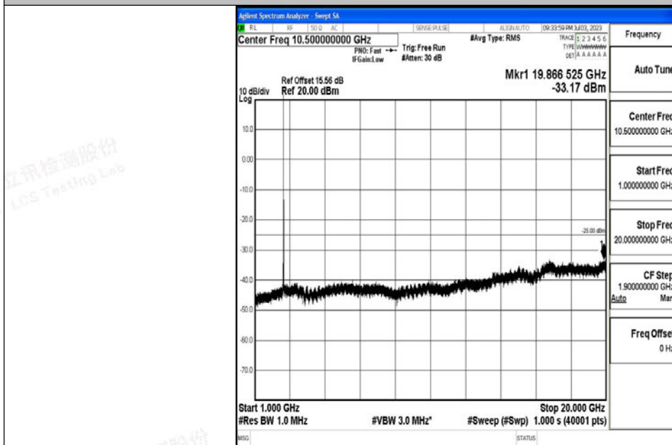
Band7_15MHz_QPSK_21375_1RB#0_1000~20000_1000~20000
