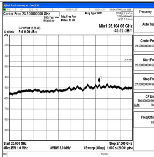
Band7_15MHz_QPSK_21375_1RB#0_20000~27000_20000~27000
