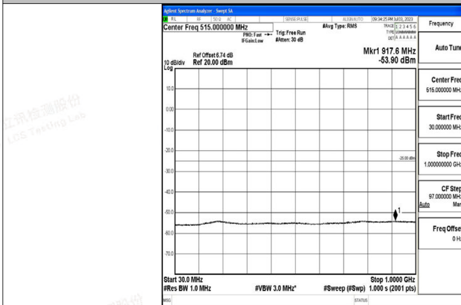
Band7_15MHz_16QAM_21375_1RB#0_30~1000_30~1000
