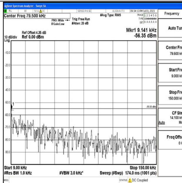
Band7_15MHz_16QAM_21375_1RB#0_0.009~0.15_0.009~0.15
