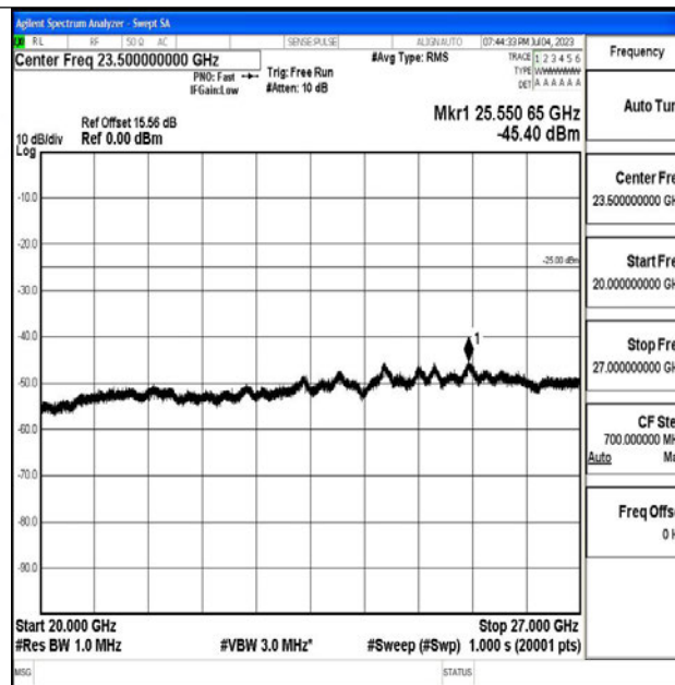
Band7_10MHz_QPSK_21100_1RB#0_20000~27000_20000~27000
