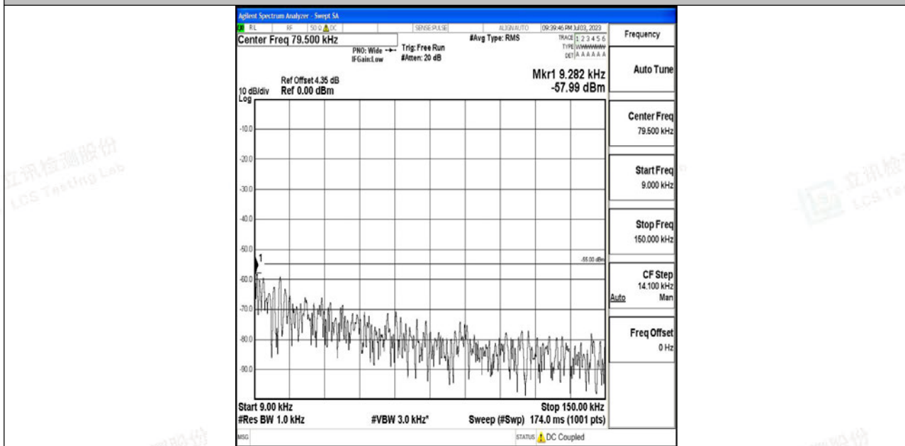
Band7_20MHz_16QAM_21100_1RB#0_0.009~0.15_0.009~0.15
