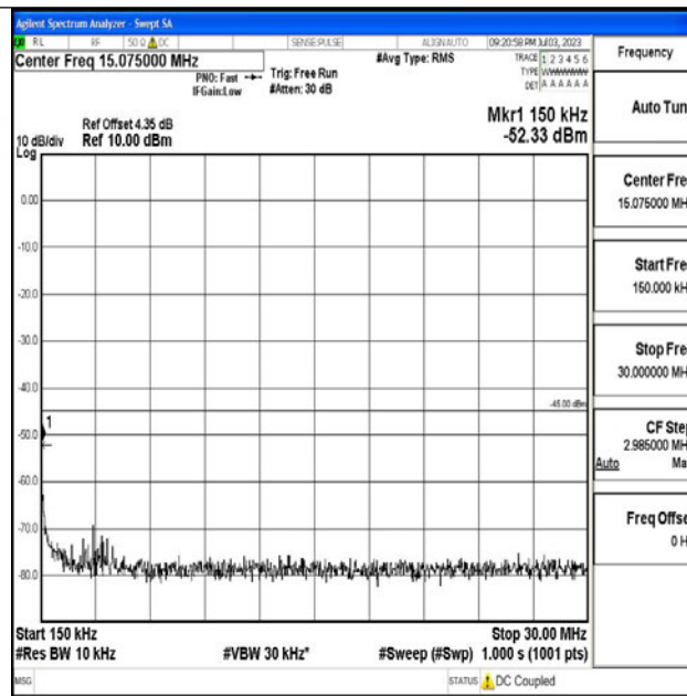
Band7_5MHz_16QAM_21425_1RB#0_0.15~30_0.15~30
