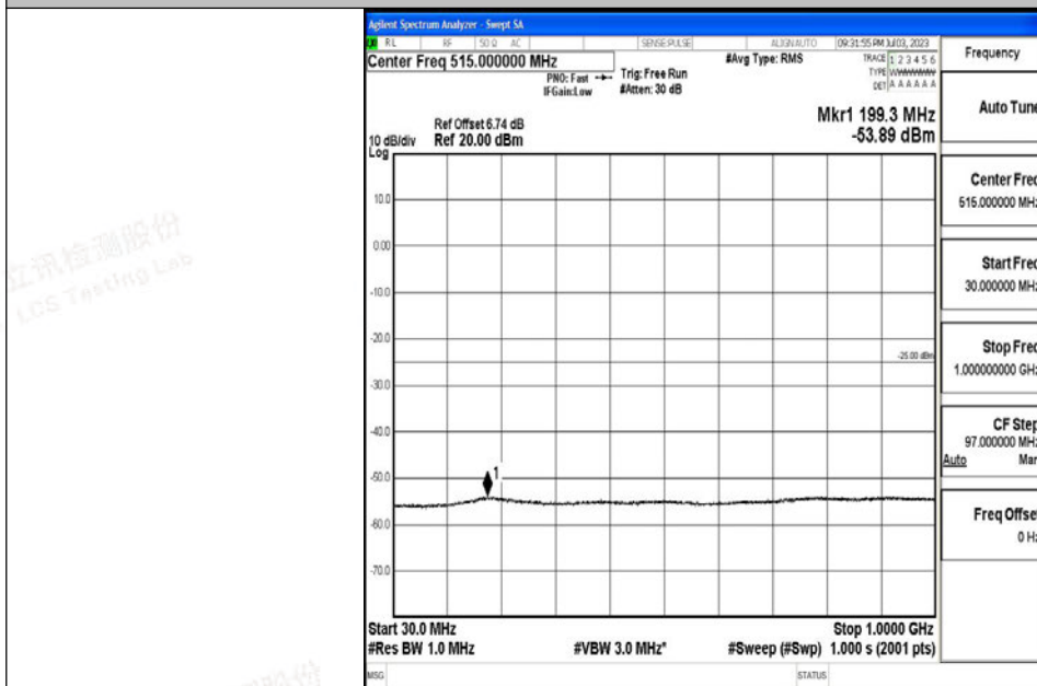
Band7_15MHz_16QAM_20825_1RB#0_30~1000_30~1000
