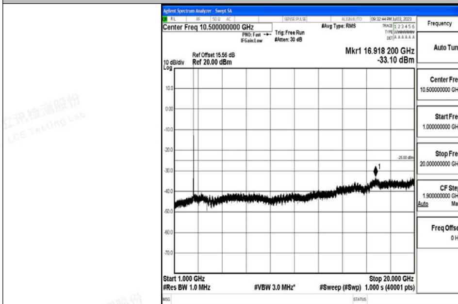
Band7_15MHz_QPSK_21100_1RB#0_1000~20000_1000~20000
