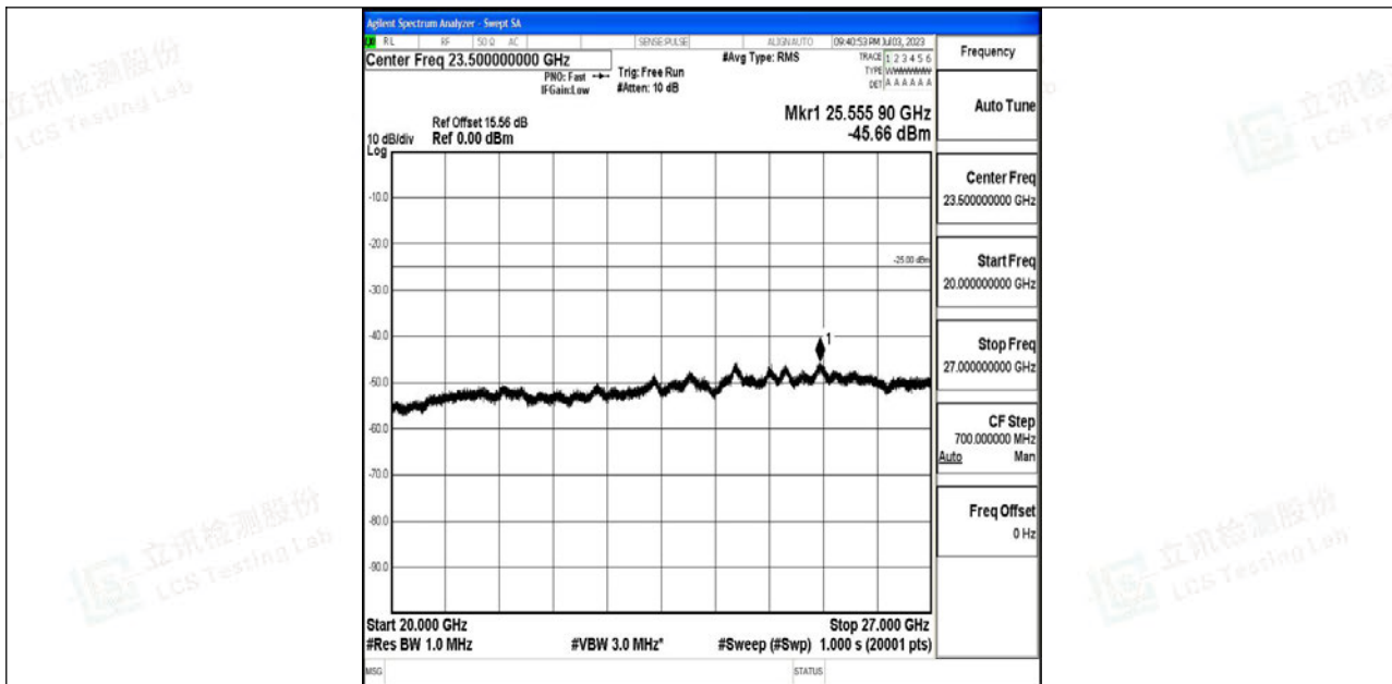
Band7_20MHz_QPSK_21350_1RB#0_20000~27000_20000~27000
