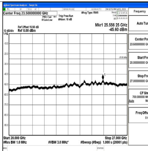
Band7_15MHz_QPSK_21100_1RB#0_20000~27000_20000~27000
