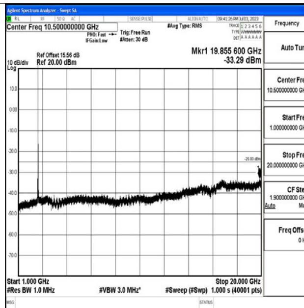
Band7_20MHz_16QAM_21350_1RB#0_1000~20000_1000~20000
