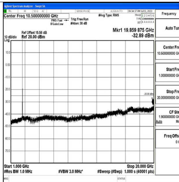
Band7_15MHz_16QAM_21375_1RB#0_1000~20000_1000~20000
