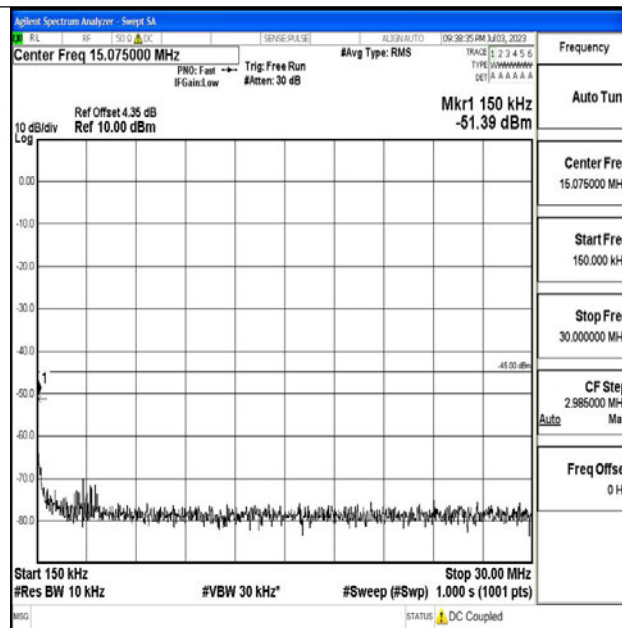
Band7_20MHz_16QAM_20850_1RB#0_0.15~30_0.15~30
