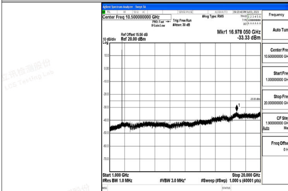
Band7_5MHz_QPSK_21425_1RB#0_1000~20000_1000~20000
