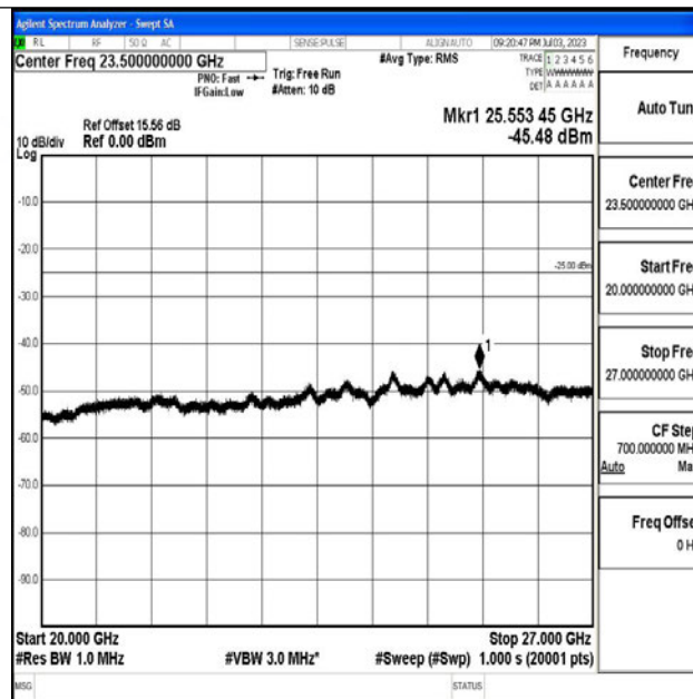
Band7_5MHz_QPSK_21425_1RB#0_20000~27000_20000~27000
