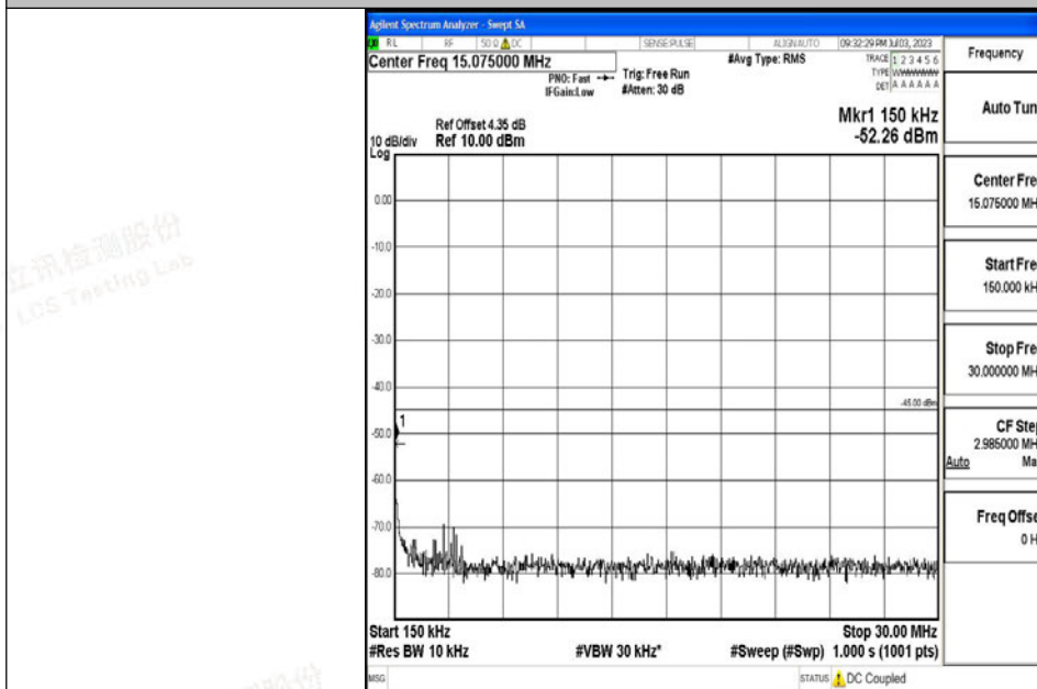
Band7_15MHz_QPSK_21100_1RB#0_0.15~30_0.15~30
