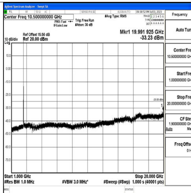
Band7_20MHz_16QAM_20850_1RB#0_1000~20000_1000~20000
