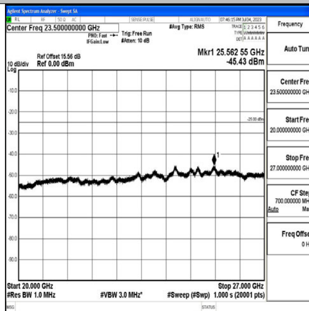
Band7_10MHz_16QAM_21400_1RB#0_20000~27000_20000~27000
