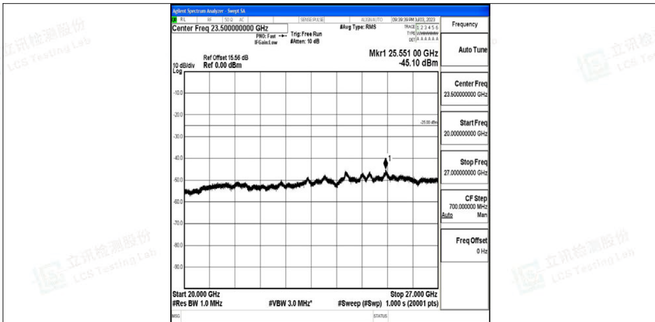
Band7_20MHz_QPSK_21100_1RB#0_20000~27000_20000~27000
