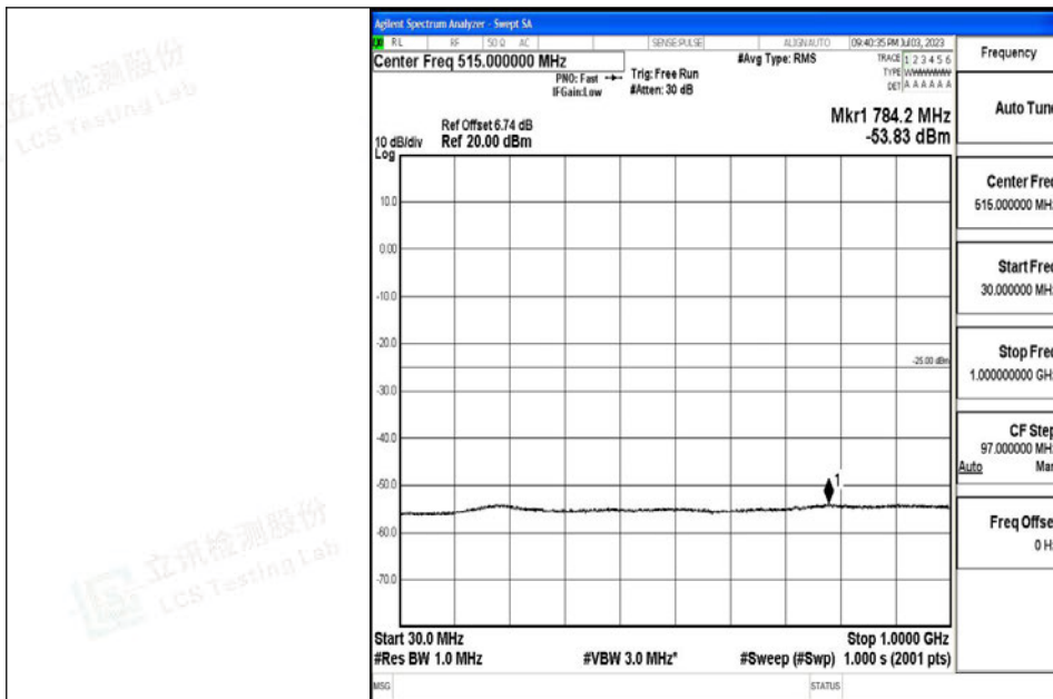
Band7_20MHz_QPSK_21350_1RB#0_30~1000_30~1000
