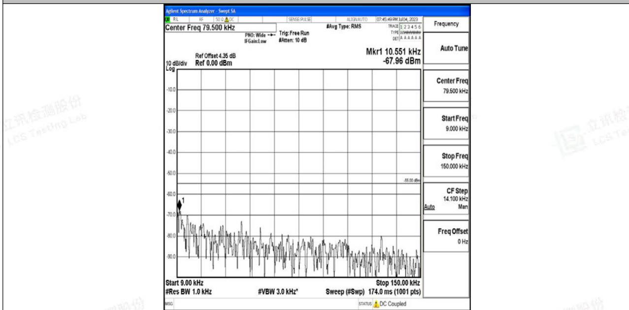
Band7_10MHz_16QAM_21400_1RB#0_0.009~0.15_0.009~0.15
