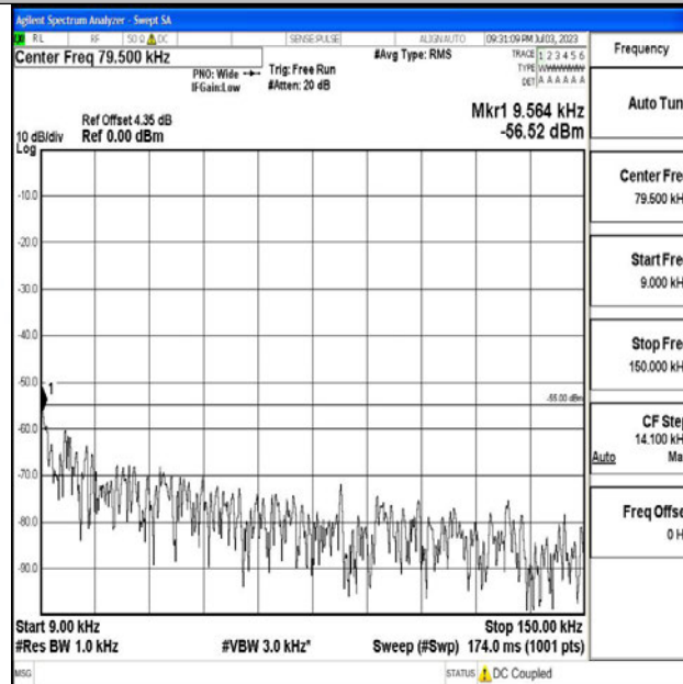
Band7_15MHz_QPSK_20825_1RB#0_0.009~0.15_0.009~0.15
