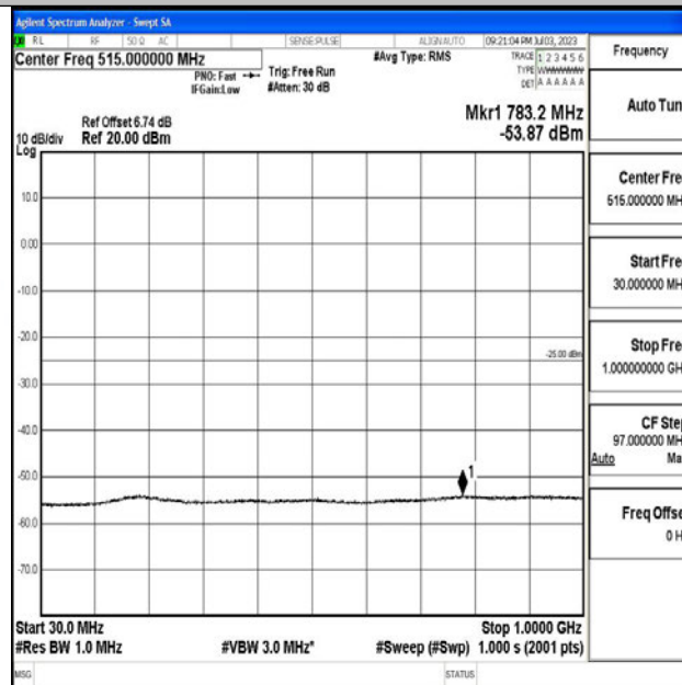
Band7_5MHz_16QAM_21425_1RB#0_30~1000_30~1000
