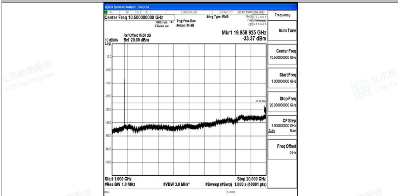
Band7_10MHz_QPSK_21400_1RB#0_1000~20000_1000~20000
