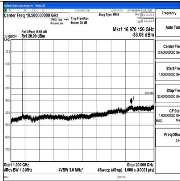
Band7_10MHz_16QAM_21400_1RB#0_1000~20000_1000~20000
