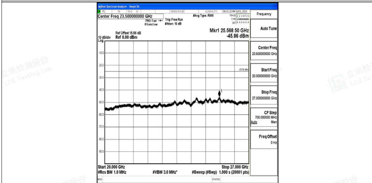
Band7_5MHz_16QAM_21425_1RB#0_20000~27000_20000~27000
