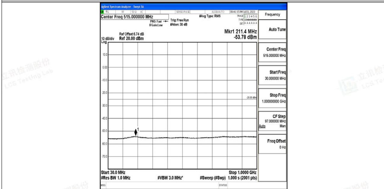
Band7_20MHz_16QAM_21350_1RB#0_30~1000_30~1000
