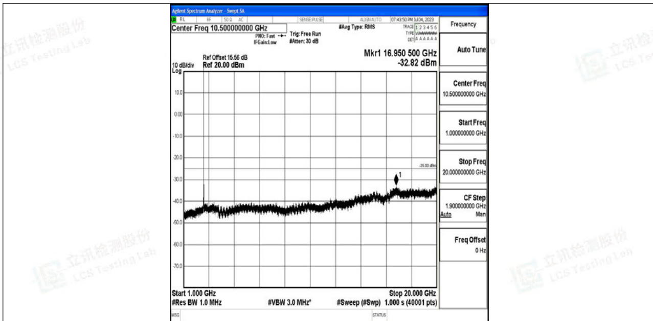
Band7_10MHz_16QAM_20800_1RB#0_1000~20000_1000~20000
