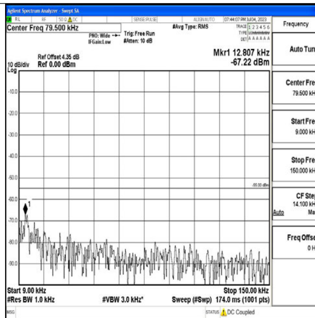
Band7_10MHz_QPSK_21100_1RB#0_0.009~0.15_0.009~0.15
