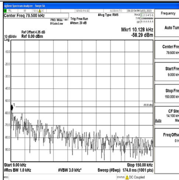
Band7_5MHz_16QAM_21425_1RB#0_0.009~0.15_0.009~0.15
