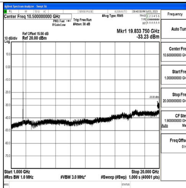
Band7_20MHz_16QAM_21100_1RB#0_1000~20000_1000~20000
