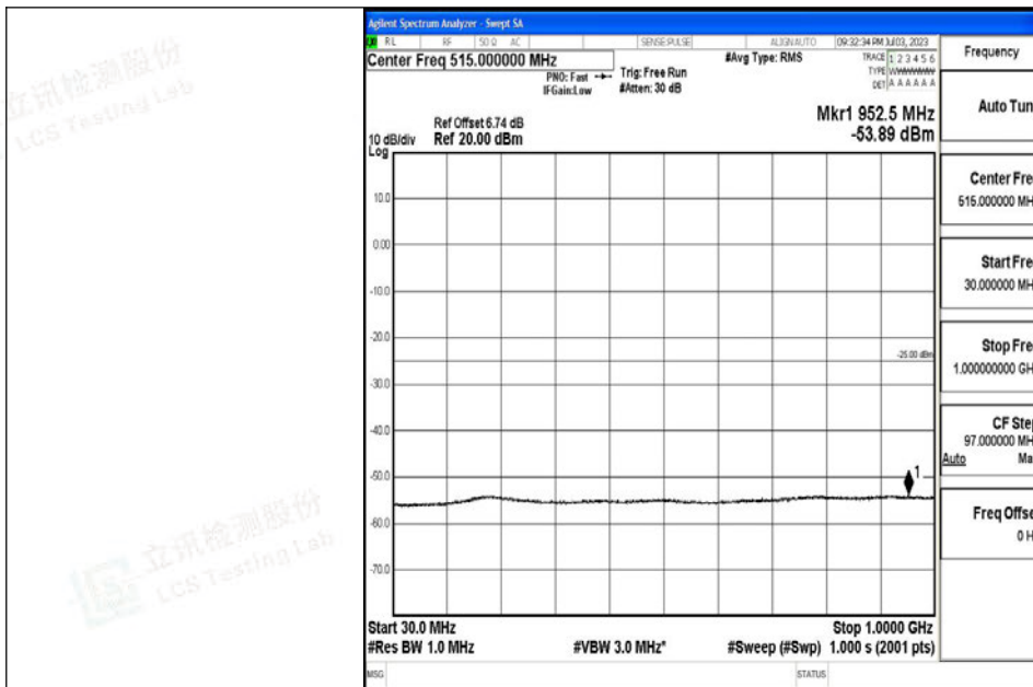
Band7_15MHz_QPSK_21100_1RB#0_30~1000_30~1000
