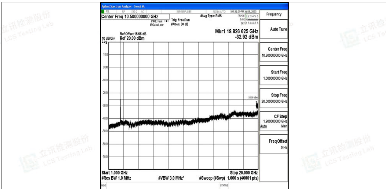
Band7_15MHz_QPSK_20825_1RB#0_1000~20000_1000~20000
