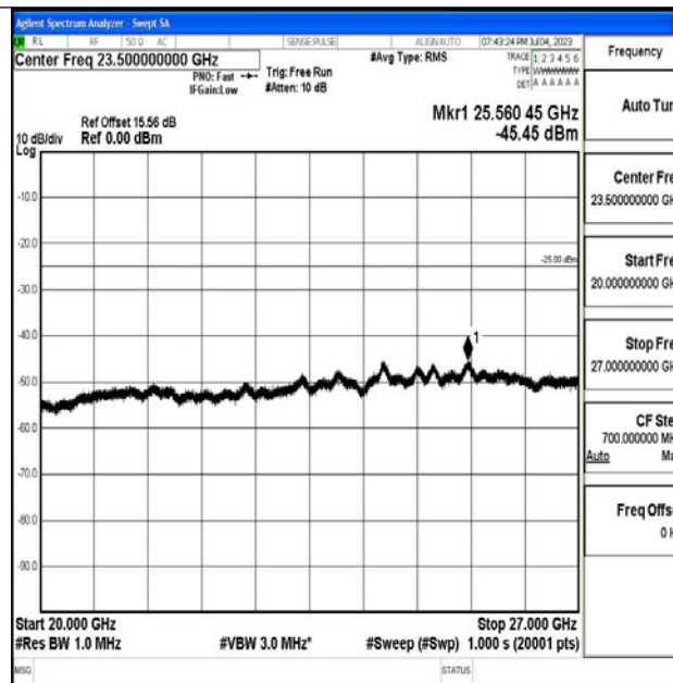
Band7_10MHz_QPSK_20800_1RB#0_20000~27000_20000~27000
