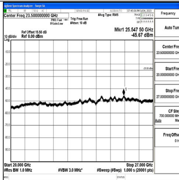
Band7_10MHz_16QAM_21100_1RB#0_20000~27000_20000~27000
