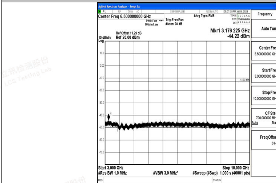
Band5_5MHz_16QAM_20625_1RB#0_3000~10000_3000~10000
