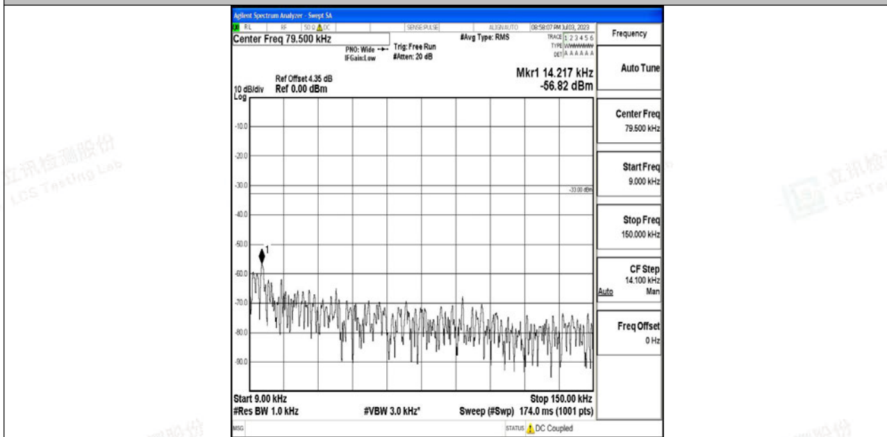
Band5_3MHz_16QAM_20525_1RB#0_0.009~0.15_0.009~0.15
