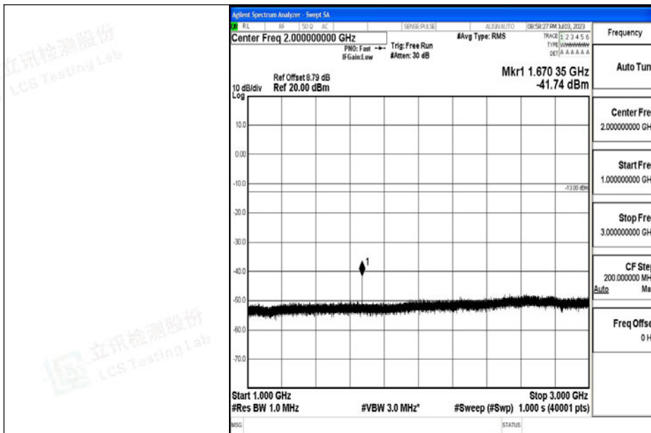
Band5_3MHz_16QAM_20525_1RB#0_1000~3000_1000~3000
