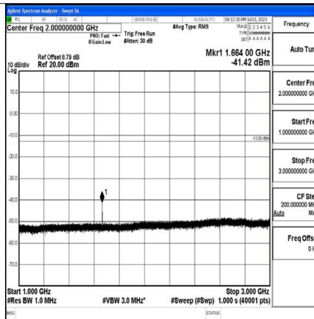
Band5_10MHz_16QAM_20525_1RB#0_1000~3000_1000~3000
