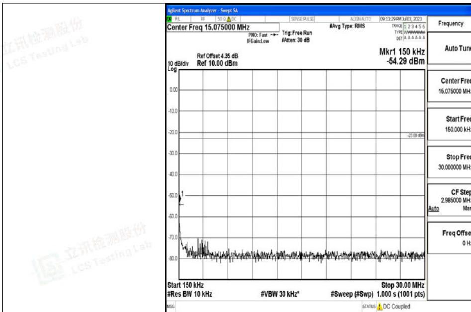
Band5_10MHz_16QAM_20600_1RB#0_0.15~30_0.15~30
