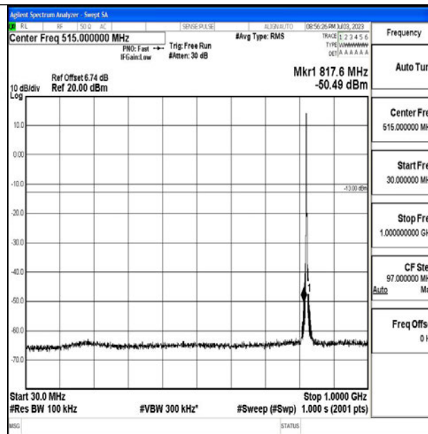
Band5_3MHz_QPSK_20415_1RB#0_30~1000_30~1000
