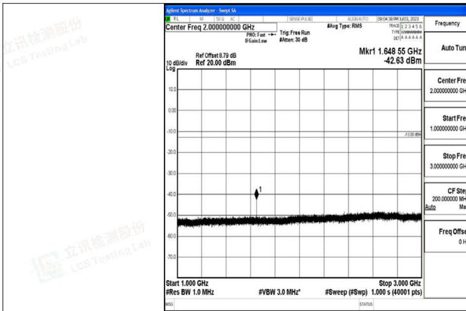
Band5_5MHz_16QAM_20425_1RB#0_1000~3000_1000~3000
