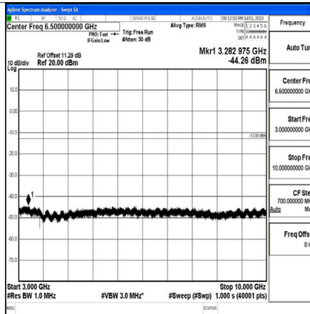
Band5_10MHz_QPSK_20525_1RB#0_3000~10000_3000~10000
