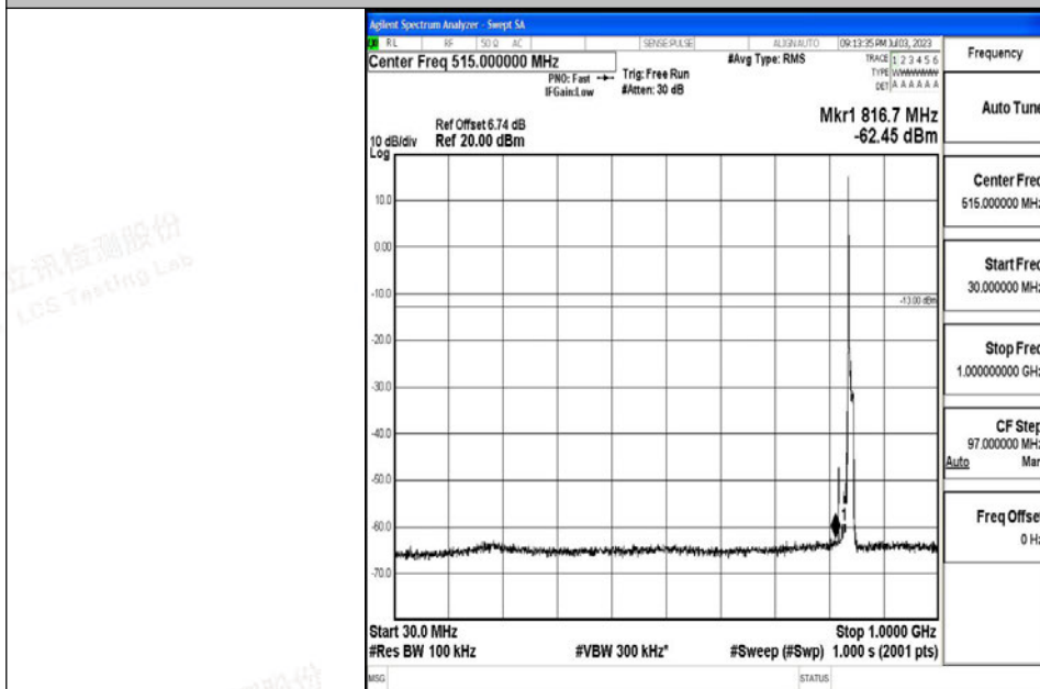
Band5_10MHz_16QAM_20600_1RB#0_30~1000_30~1000
