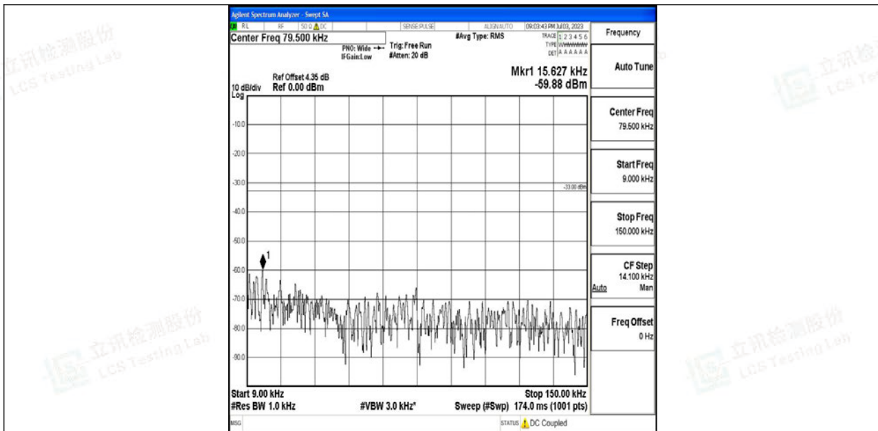
Band5_5MHz_QPSK_20425_1RB#0_0.009~0.15_0.009~0.15
