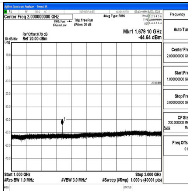
Band5_10MHz_16QAM_20600_1RB#0_1000~3000_1000~3000
