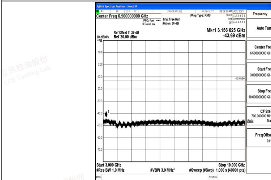
Band5_3MHz_16QAM_20525_1RB#0_3000~10000_3000~10000
