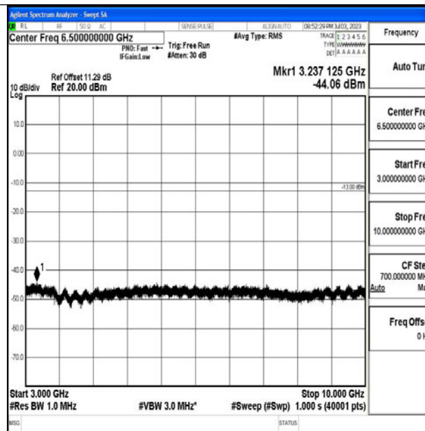
Band5_1.4MHz_QPSK_20643_1RB#0_3000~10000_3000~10000
