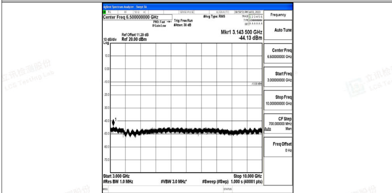
Band5_3MHz_16QAM_20635_1RB#0_3000~10000_3000~10000
