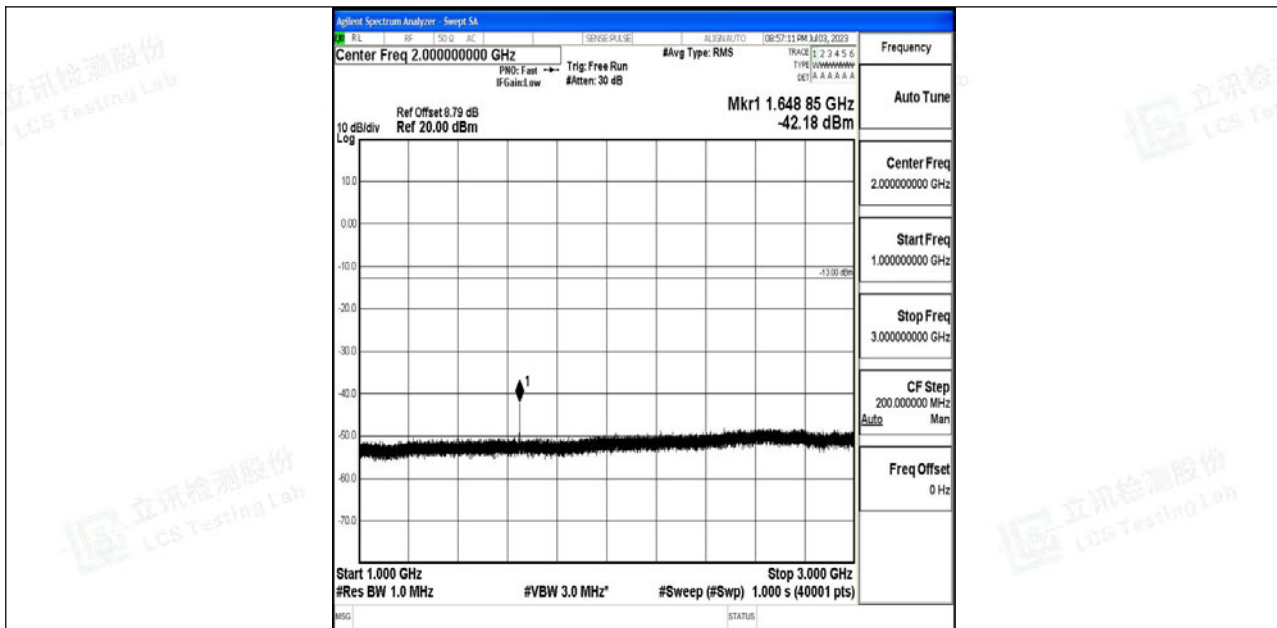
Band5_3MHz_16QAM_20415_1RB#0_1000~3000_1000~3000
