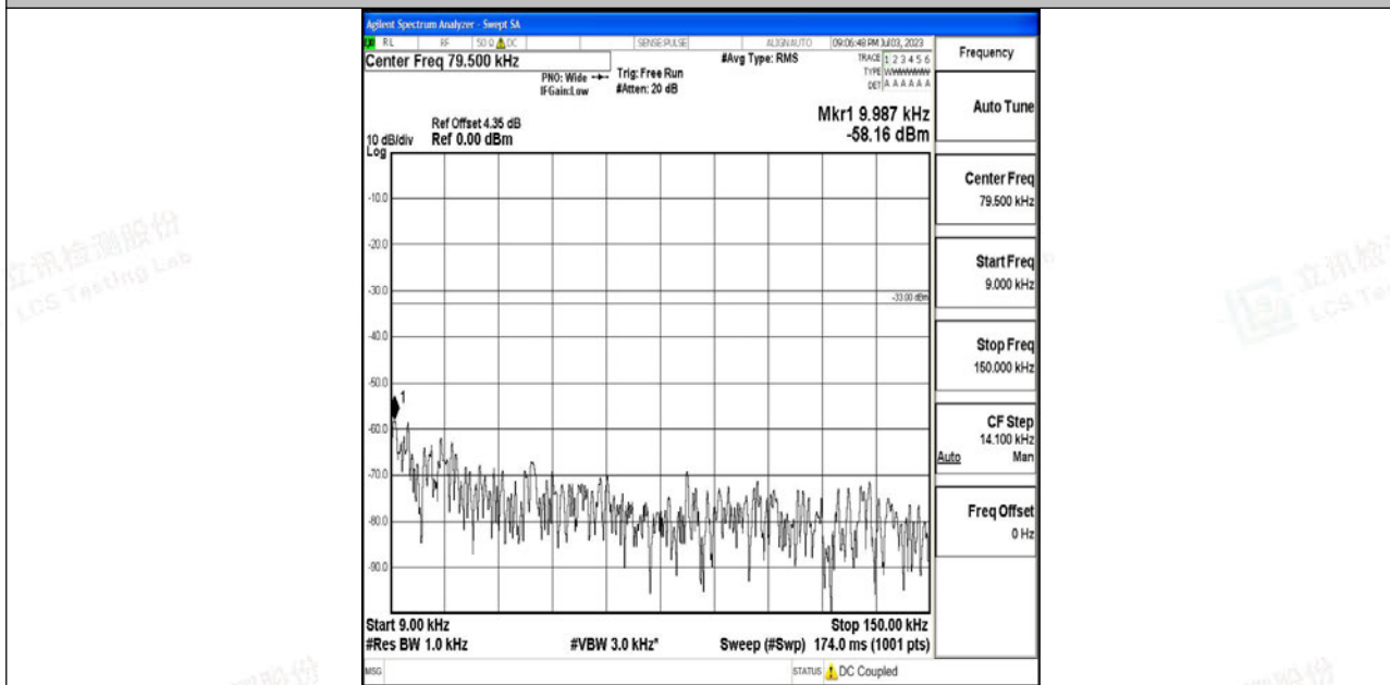
Band5_5MHz_16QAM_20625_1RB#0_0.009~0.15_0.009~0.15
