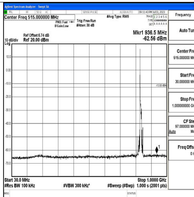
Band5_10MHz_QPSK_20525_1RB#0_30~1000_30~1000
