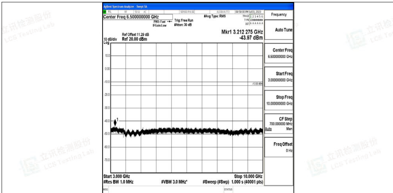
Band5_3MHz_QPSK_20525_1RB#0_3000~10000_3000~10000
