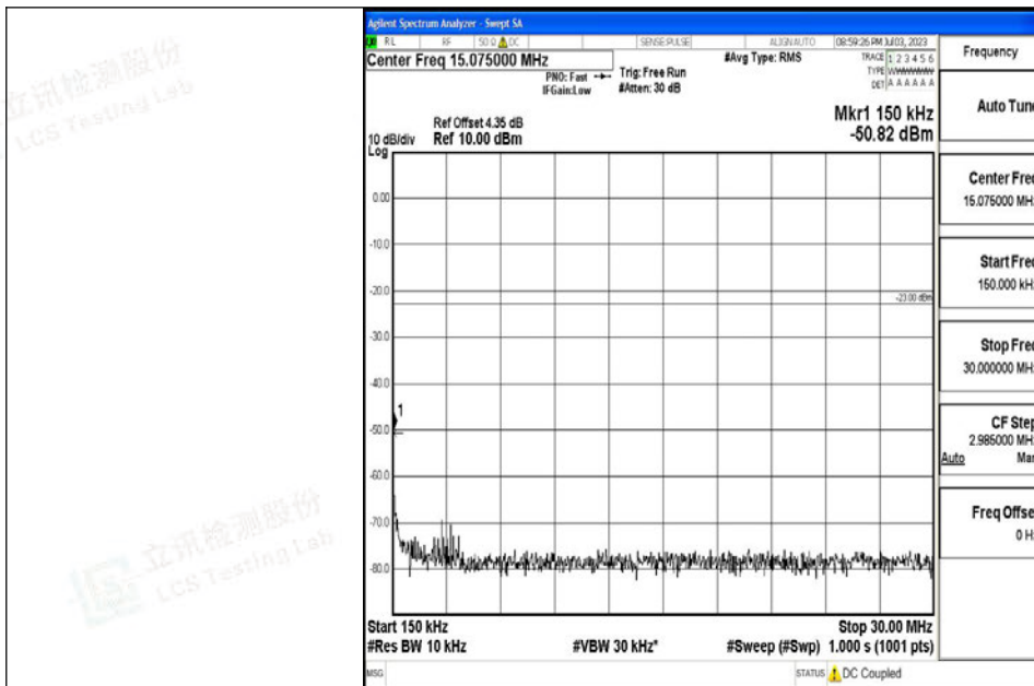
Band5_3MHz_16QAM_20635_1RB#0_0.15~30_0.15~30
