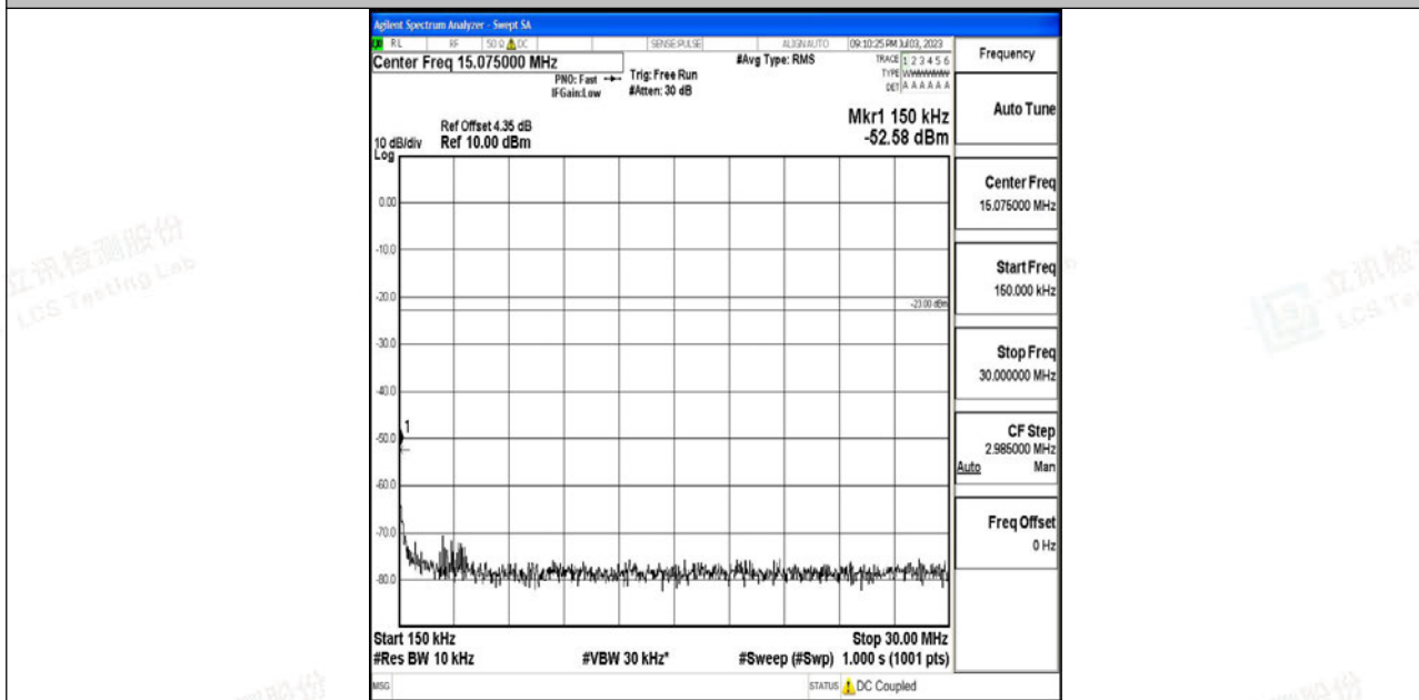
Band5_10MHz_QPSK_20450_1RB#0_0.15~30_0.15~30
