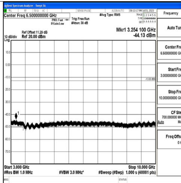
Band5_10MHz_QPSK_20600_1RB#0_3000~10000_3000~10000
