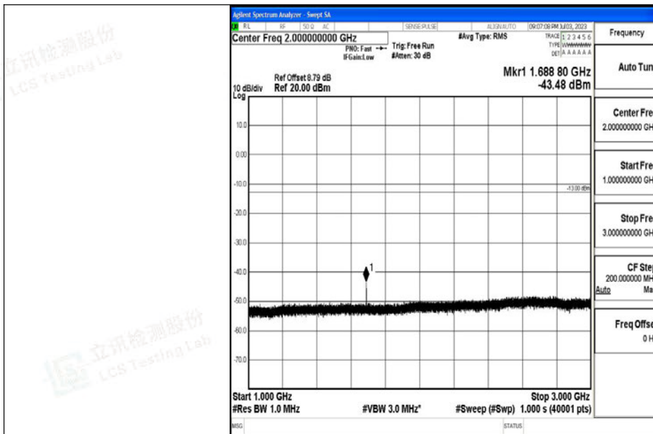
Band5_5MHz_16QAM_20625_1RB#0_1000~3000_1000~3000
