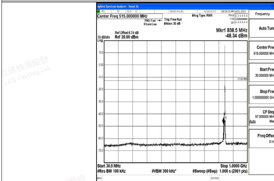
Band5_3MHz_16QAM_20635_1RB#0_30~1000_30~1000
