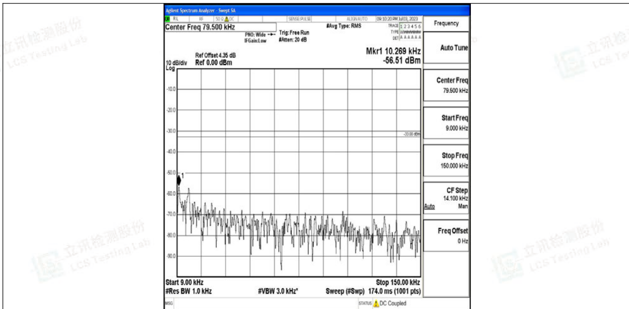
Band5_10MHz_QPSK_20450_1RB#0_0.009~0.15_0.009~0.15
