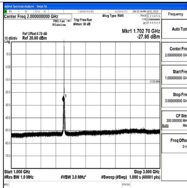
Band4_3MHz_QPSK_19965_1RB#0_1000~3000_1000~3000
