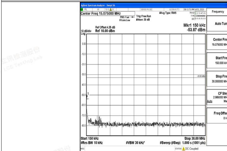
Band4_1.4MHz_16QAM_20393_1RB#0_0.15~30_0.15~30
