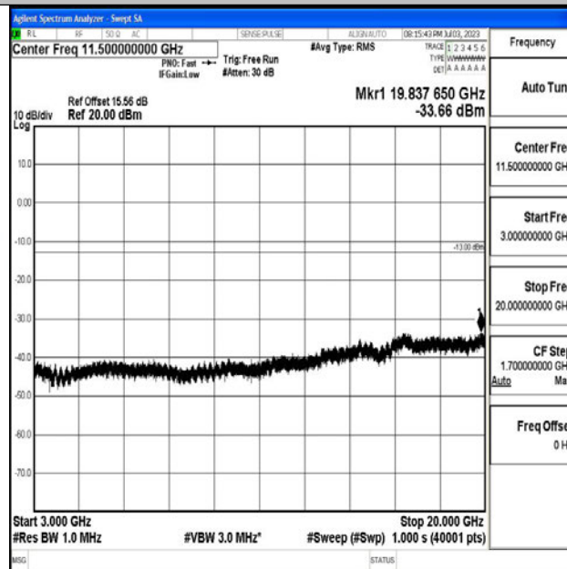
Band4_3MHz_QPSK_19965_1RB#0_3000~20000_3000~20000
