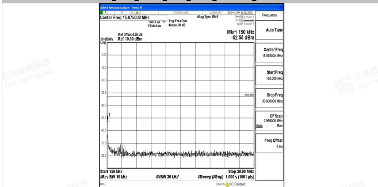
Band4_5MHz_16QAM_20175_1RB#0_0.15~30_0.15~30
