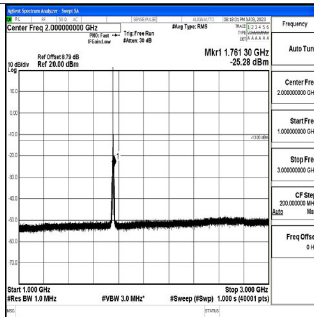
Band4_3MHz_QPSK_20385_1RB#0_1000~3000_1000~3000
