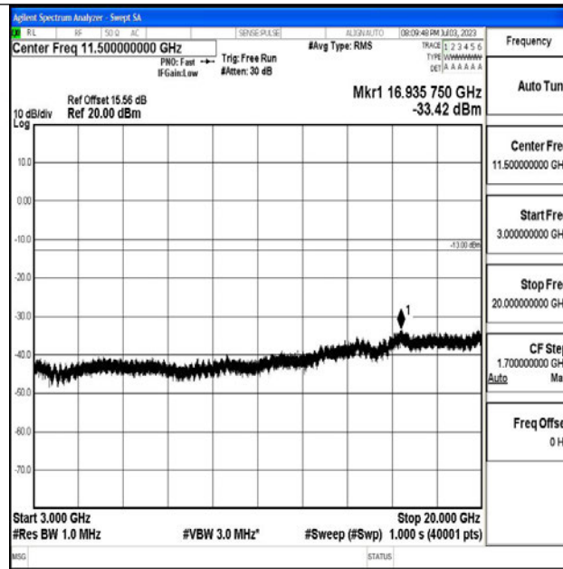
Band4_1.4MHz_16QAM_19957_1RB#0_3000~20000_3000~20000
