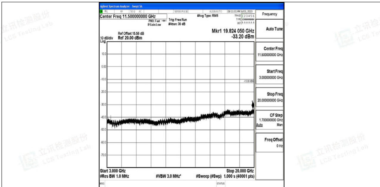
Band4_1.4MHz_16QAM_20175_1RB#0_3000~20000_3000~20000
