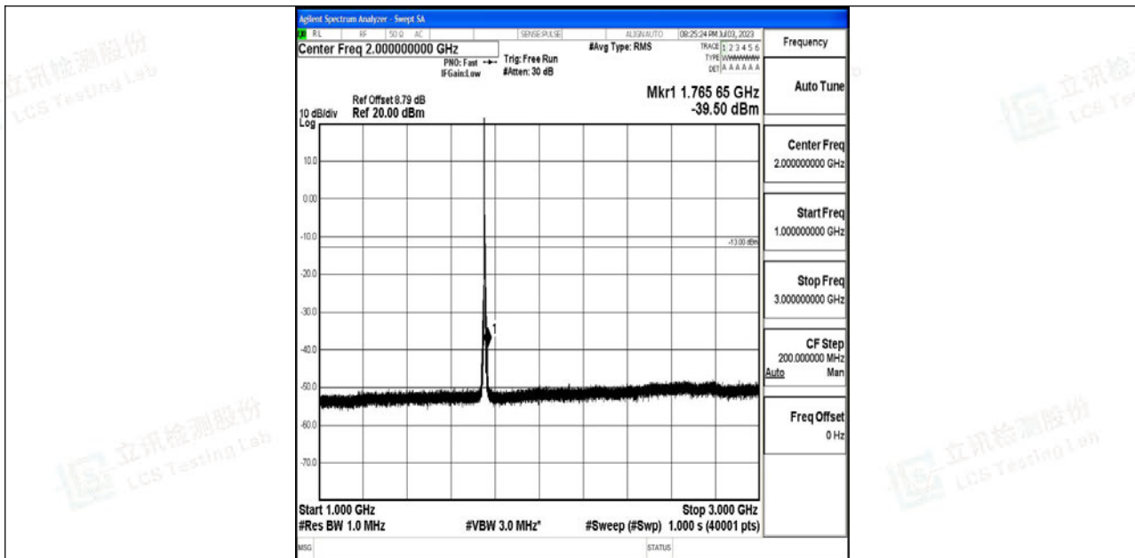
Band4_5MHz_QPSK_20375_1RB#0_1000~3000_1000~3000
