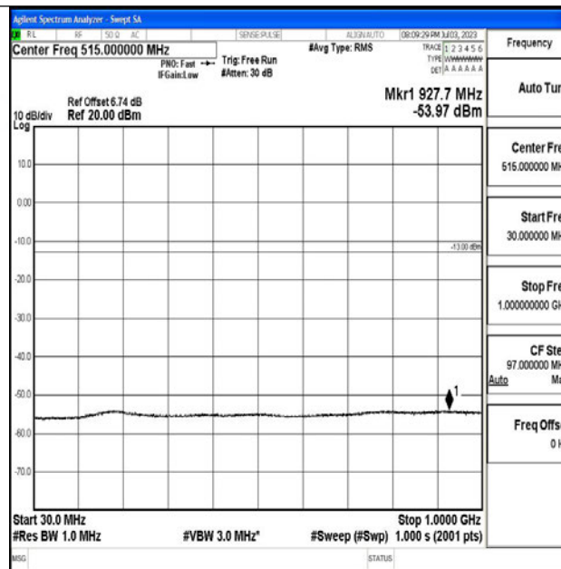
Band4_1.4MHz_16QAM_19957_1RB#0_30~1000_30~1000
