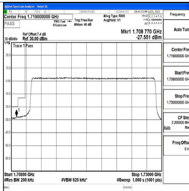
Band4_20MHz_QPSK_20050_100RB#0
