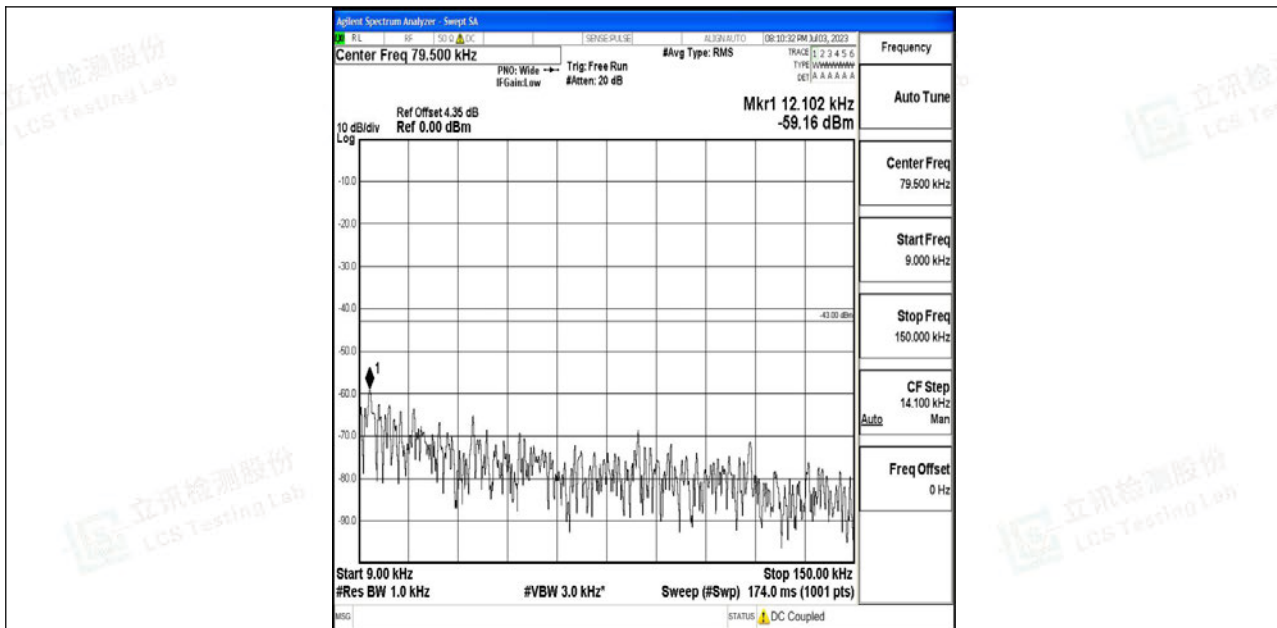
Band4_1.4MHz_16QAM_20175_1RB#0_0.009~0.15_0.009~0.15
