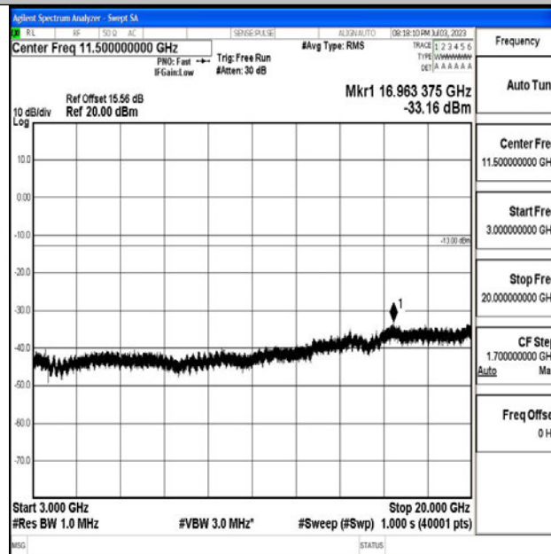
Band4_3MHz_QPSK_20385_1RB#0_3000~20000_3000~20000
