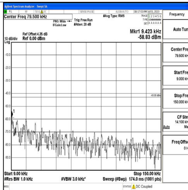
Band4_3MHz_16QAM_20175_1RB#0_0.009~0.15_0.009~0.15
