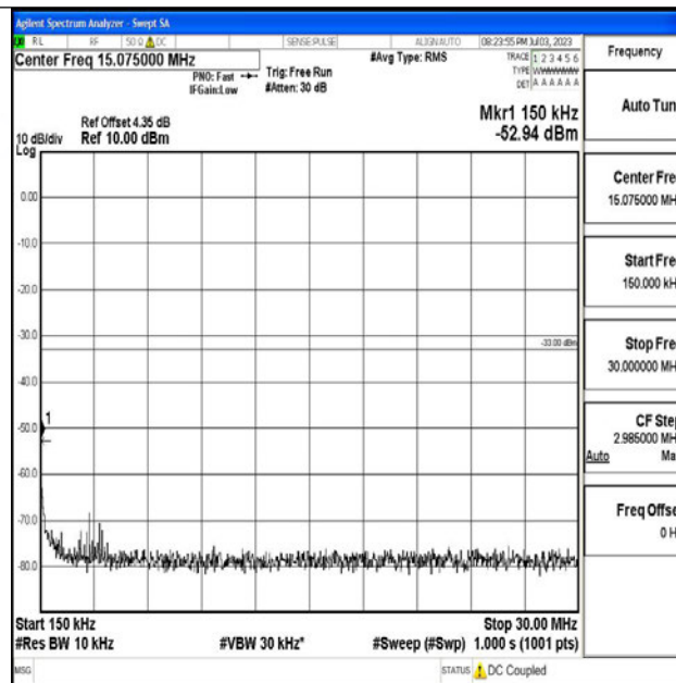
Band4_5MHz_QPSK_20175_1RB#0_0.15~30_0.15~30
