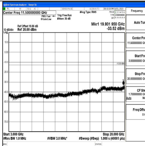
Band4_1.4MHz_QPSK_20175_1RB#0_3000~20000_3000~20000
