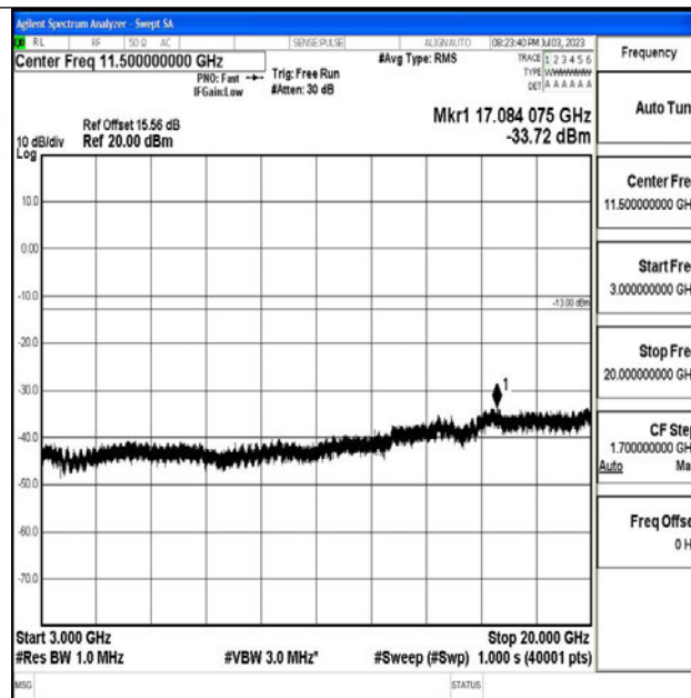
Band4_5MHz_16QAM_19975_1RB#0_3000~20000_3000~20000
