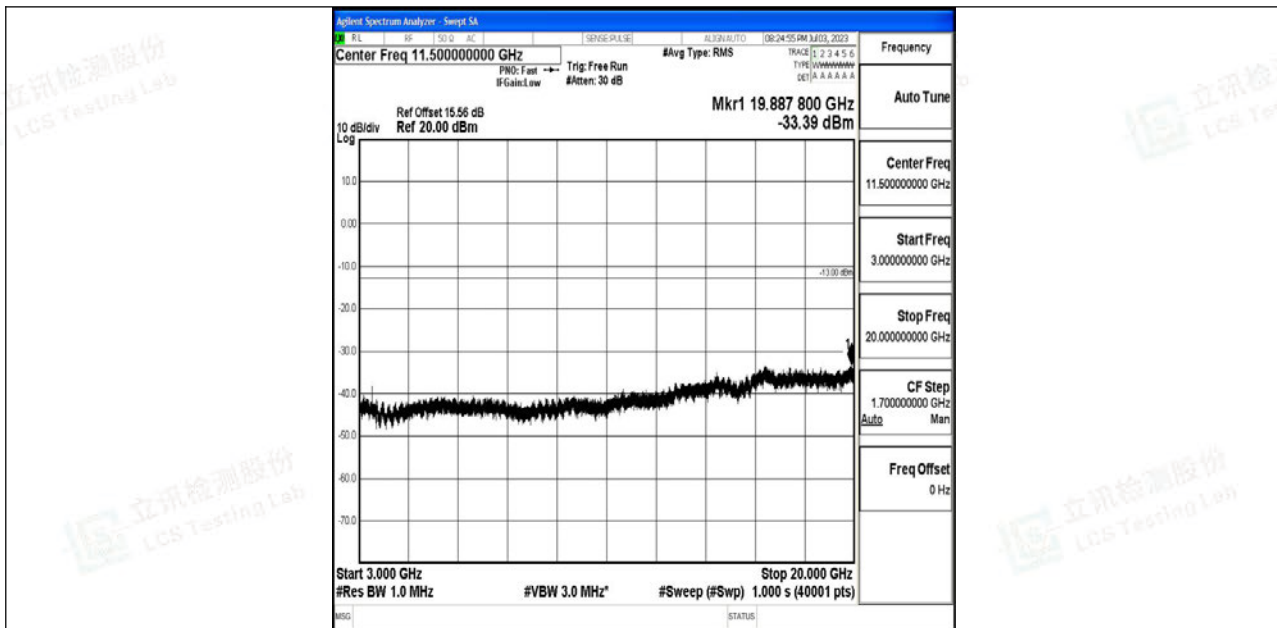
Band4_5MHz_16QAM_20175_1RB#0_3000~20000_3000~20000
