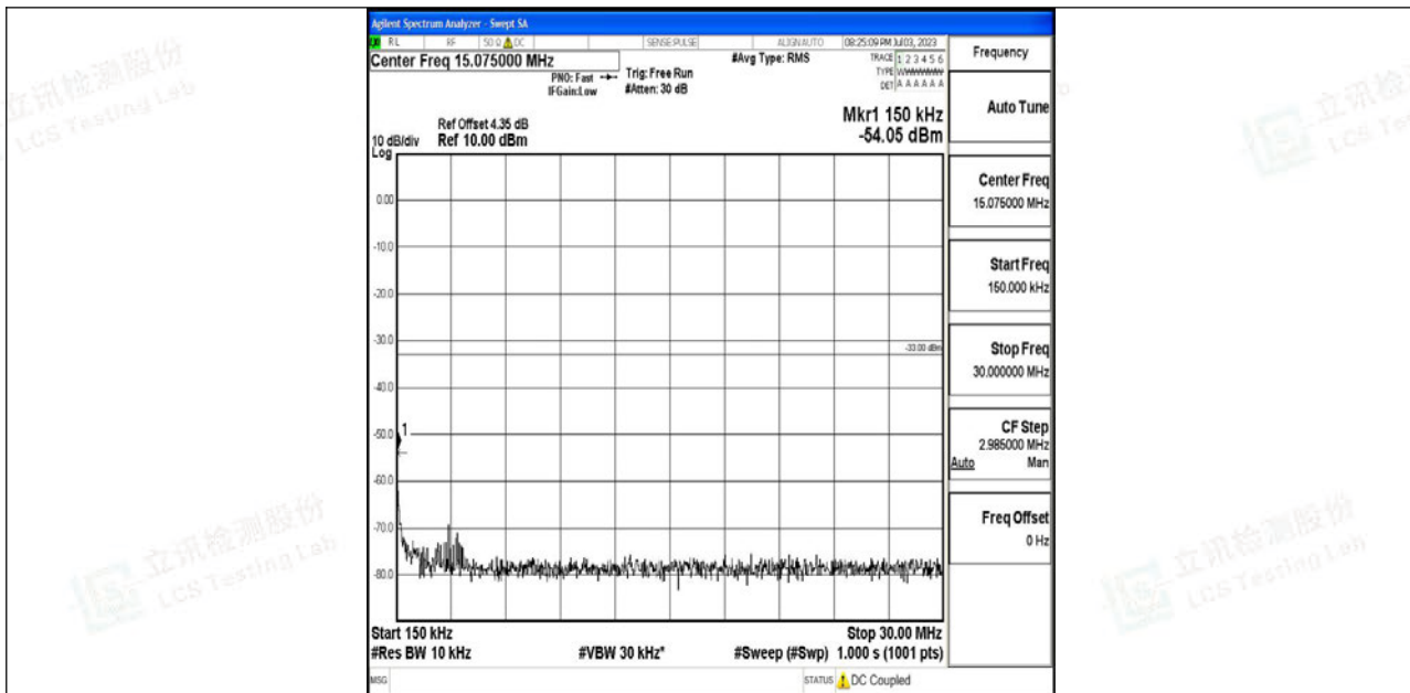
Band4_5MHz_QPSK_20375_1RB#0_0.15~30_0.15~30
