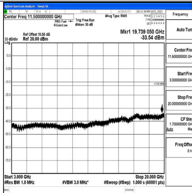
Band4_1.4MHz_QPSK_20393_1RB#0_3000~20000_3000~20000
