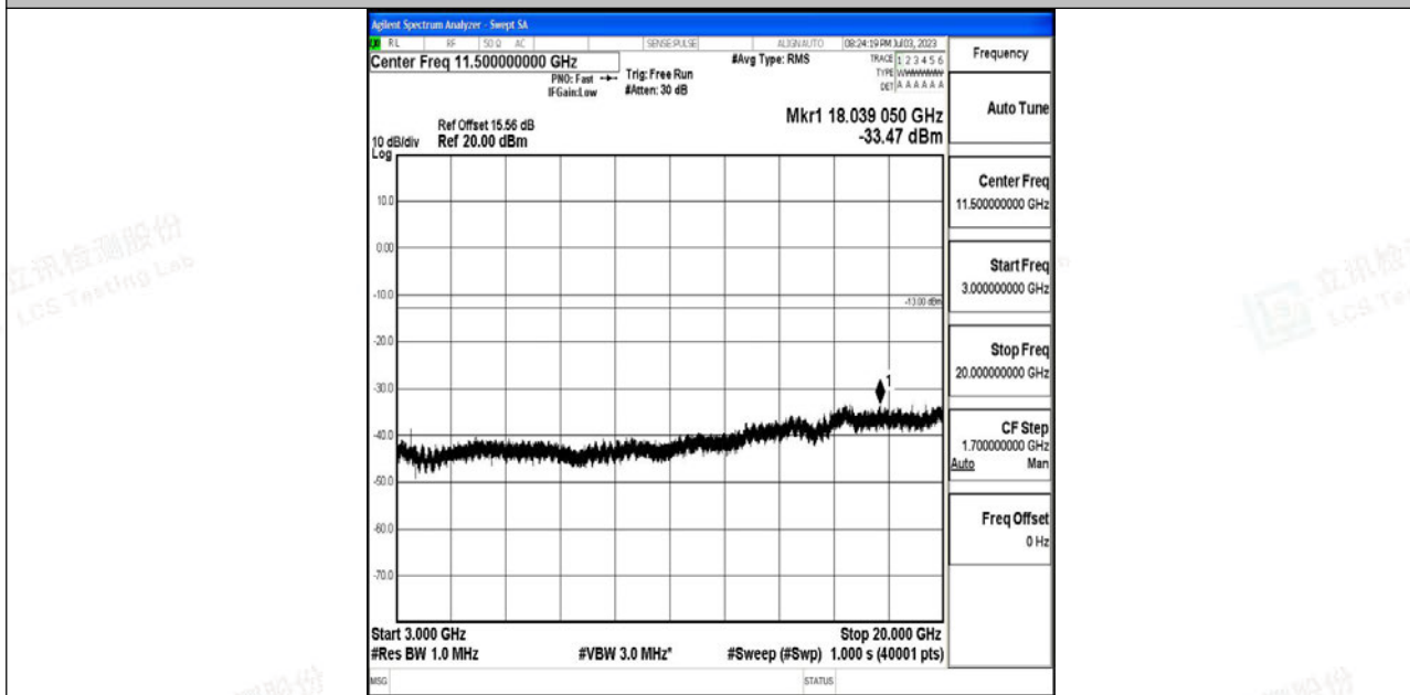
Band4_5MHz_QPSK_20175_1RB#0_3000~20000_3000~20000
