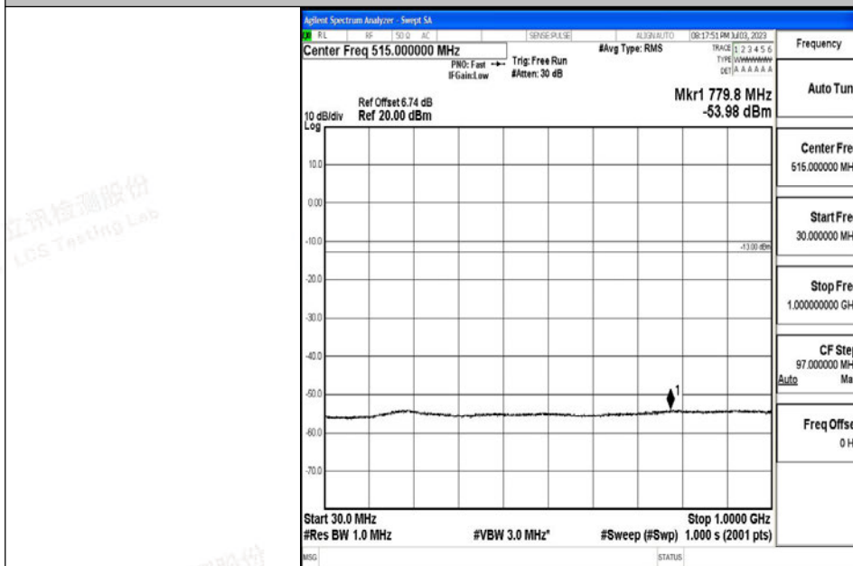
Band4_3MHz_QPSK_20385_1RB#0_30~1000_30~1000
