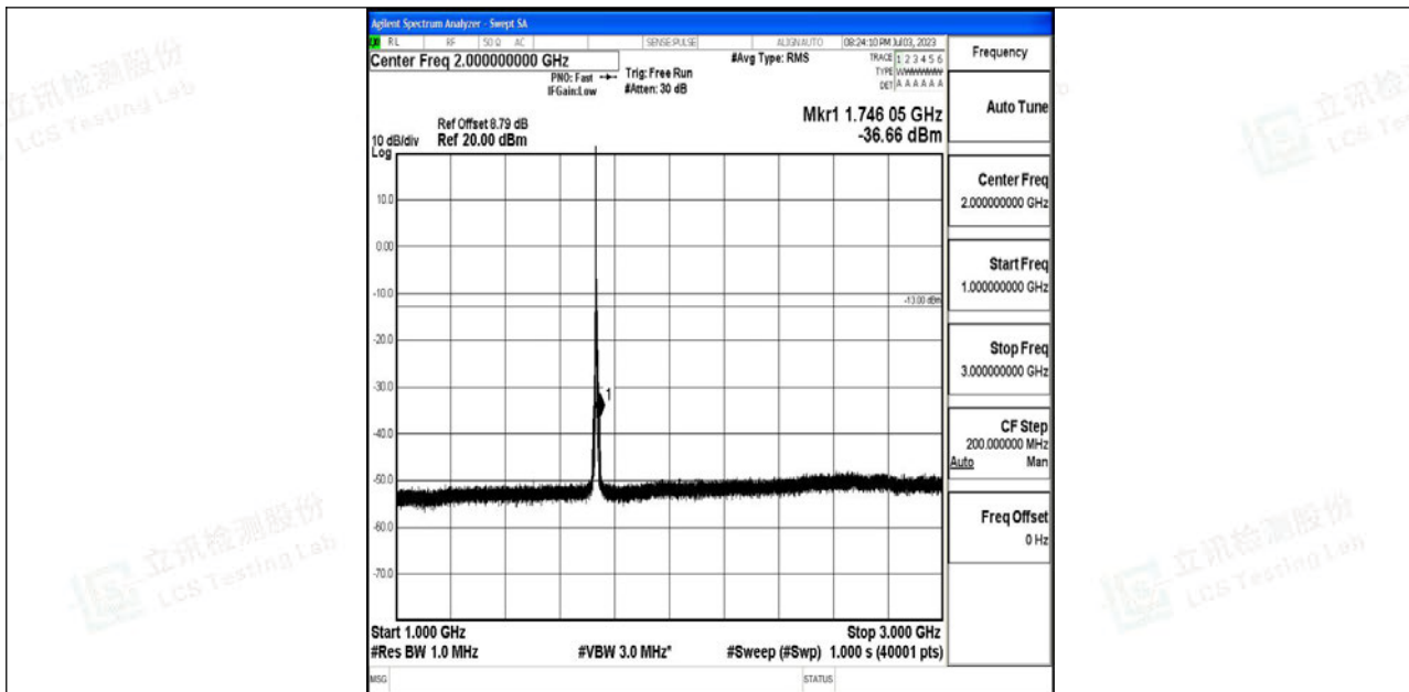
Band4_5MHz_QPSK_20175_1RB#0_1000~3000_1000~3000
