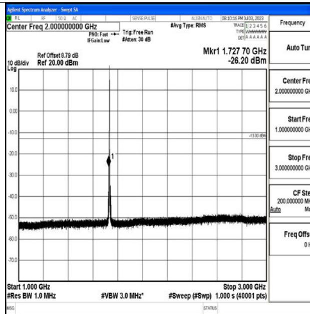
Band4_1.4MHz_QPSK_20175_1RB#0_1000~3000_1000~3000
