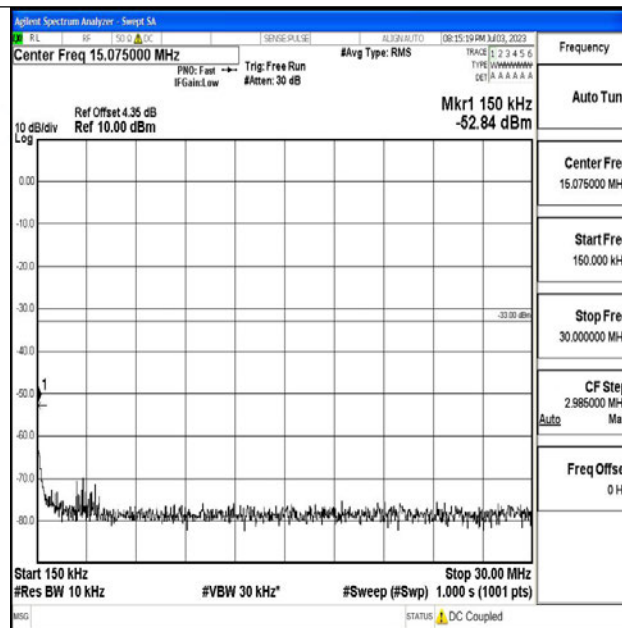
Band4_3MHz_QPSK_19965_1RB#0_0.15~30_0.15~30
