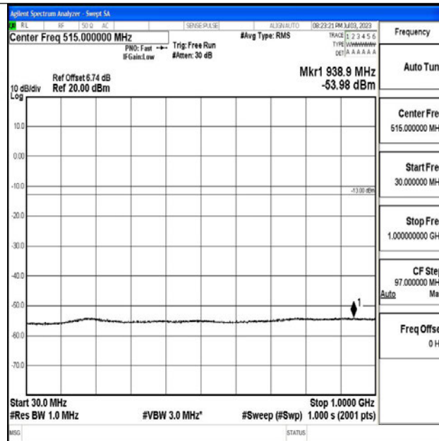
Band4_5MHz_16QAM_19975_1RB#0_30~1000_30~1000
