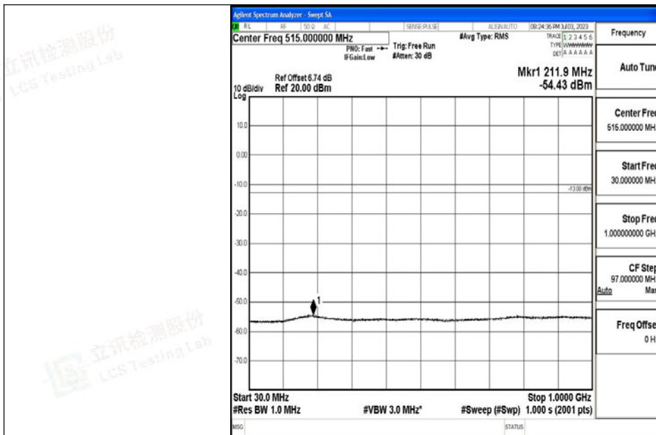
Band4_5MHz_16QAM_20175_1RB#0_30~1000_30~1000
