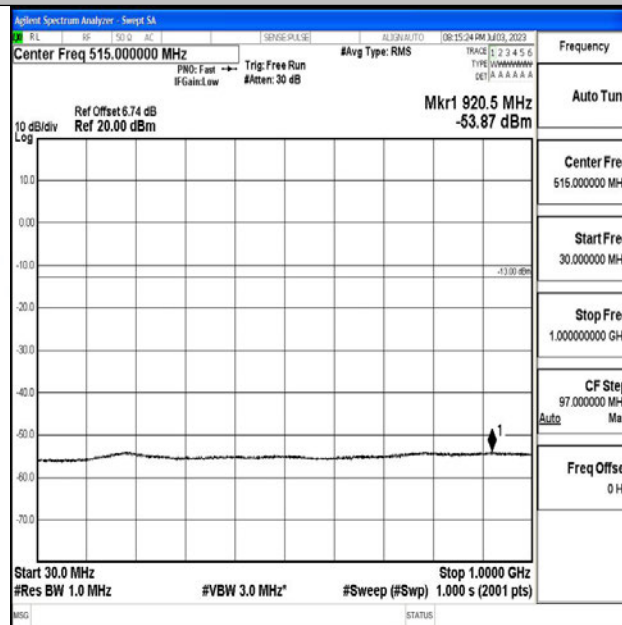
Band4_3MHz_QPSK_19965_1RB#0_30~1000_30~1000
