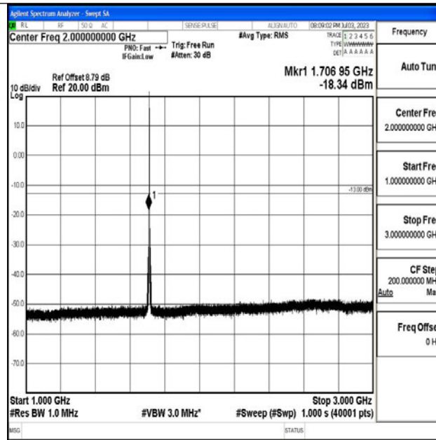
Band4_1.4MHz_QPSK_19957_1RB#0_1000~3000_1000~3000
