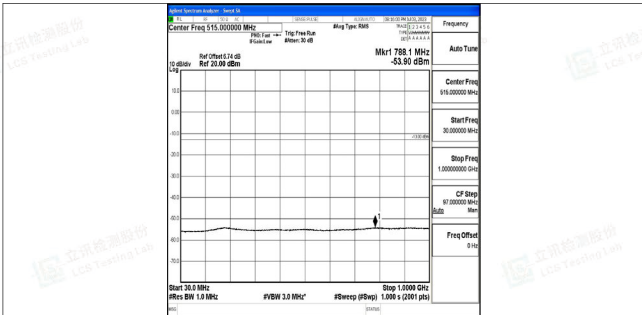
Band4_3MHz_16QAM_19965_1RB#0_30~1000_30~1000
