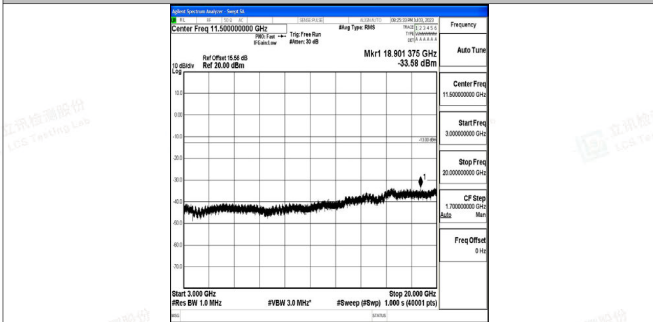
Band4_5MHz_QPSK_20375_1RB#0_3000~20000_3000~20000
