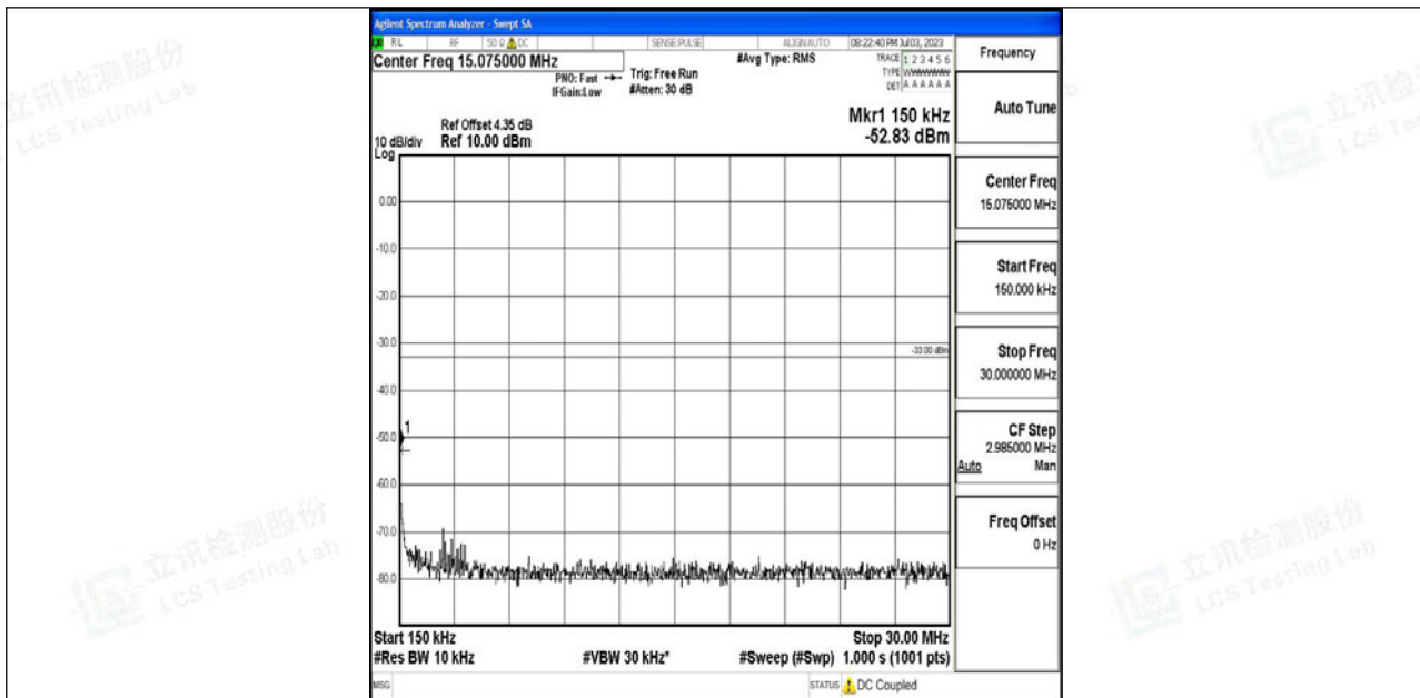
Band4_5MHz_QPSK_19975_1RB#0_0.15~30_0.15~30
