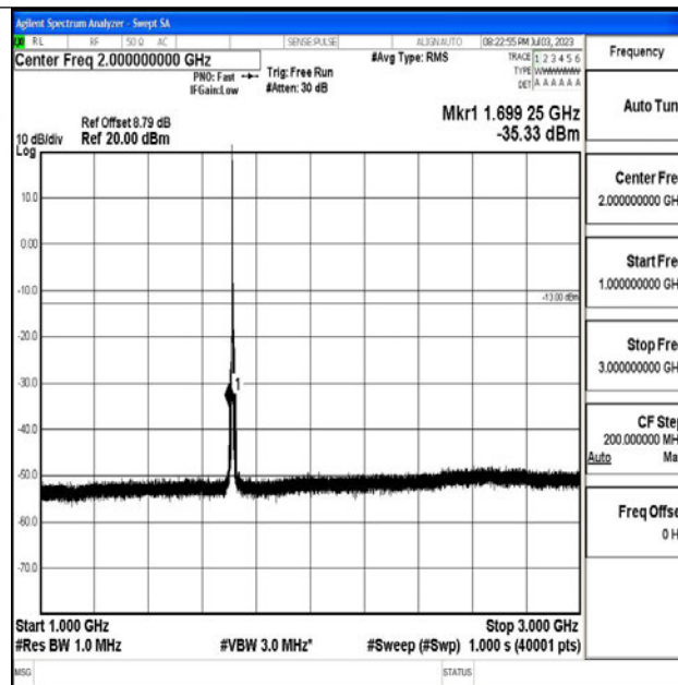
Band4_5MHz_QPSK_19975_1RB#0_1000~3000_1000~3000
