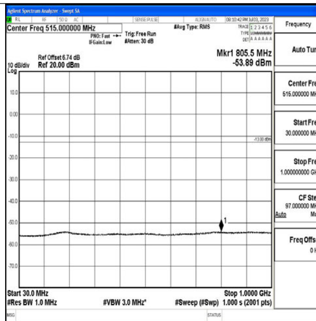
Band4_1.4MHz_16QAM_20175_1RB#0_30~1000_30~1000
