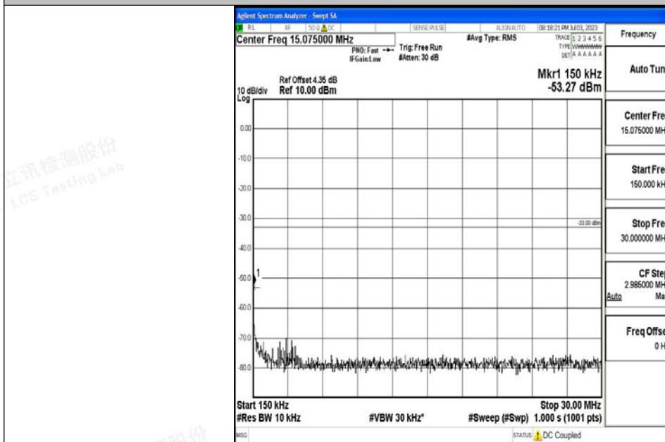
Band4_3MHz_16QAM_20385_1RB#0_0.15~30_0.15~30
