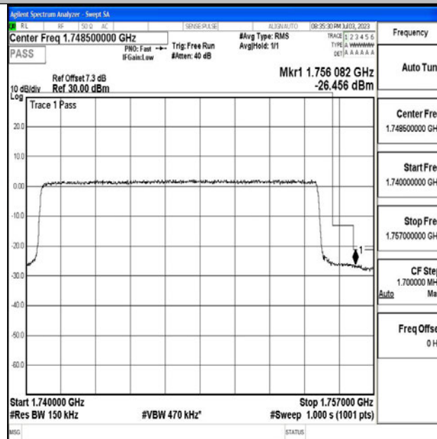
Band4_15MHz_16QAM_20325_75RB#0
