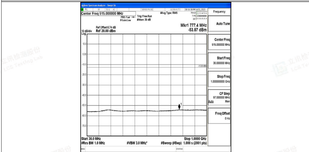
Band4_3MHz_QPSK_20175_1RB#0_30~1000_30~1000
