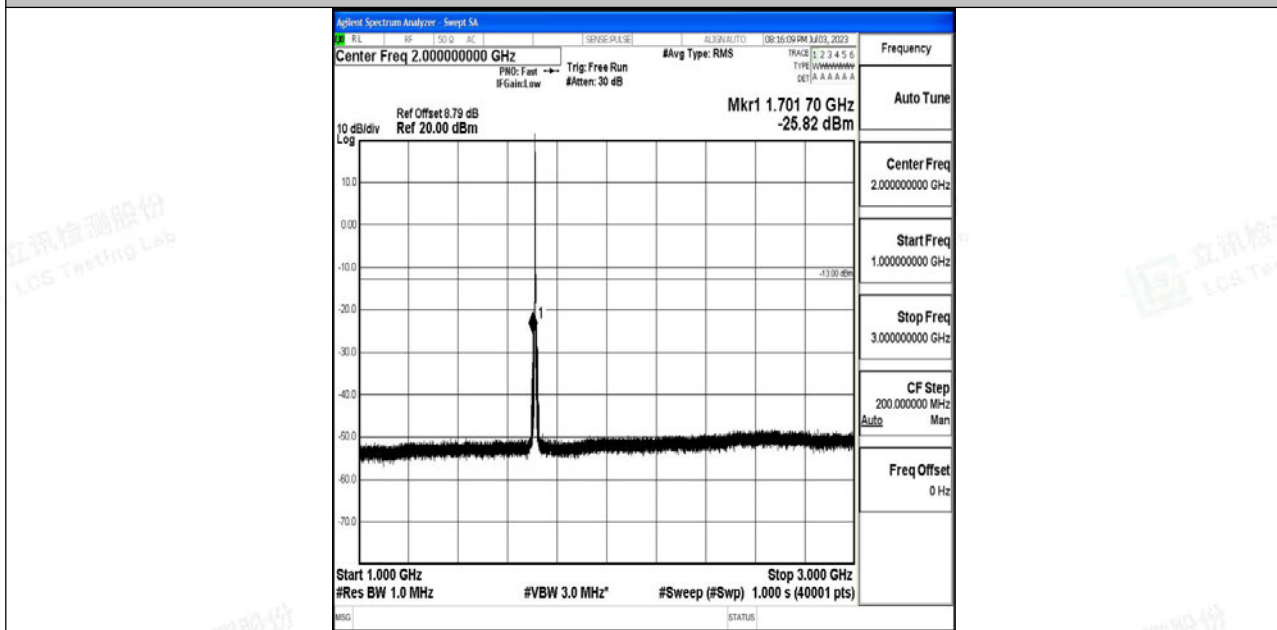
Band4_3MHz_16QAM_19965_1RB#0_1000~3000_1000~3000
