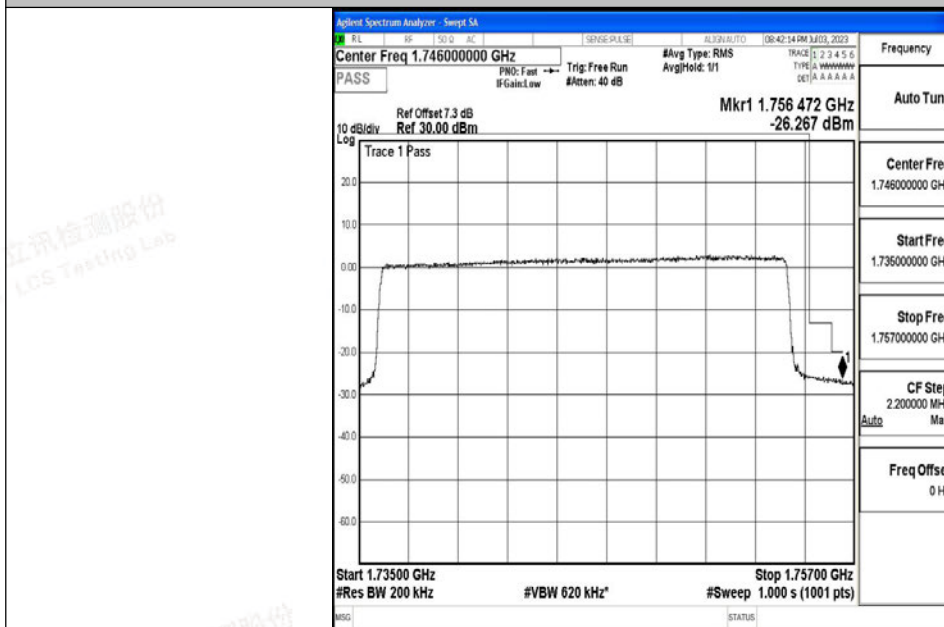
Band4_20MHz_16QAM_20300_100RB#0
