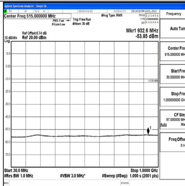
Band4_5MHz_QPSK_20175_1RB#0_30~1000_30~1000
