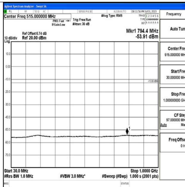
Band4_1.4MHz_16QAM_20393_1RB#0_30~1000_30~1000
