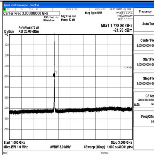
Band4_1.4MHz_16QAM_20175_1RB#0_1000~3000_1000~3000
