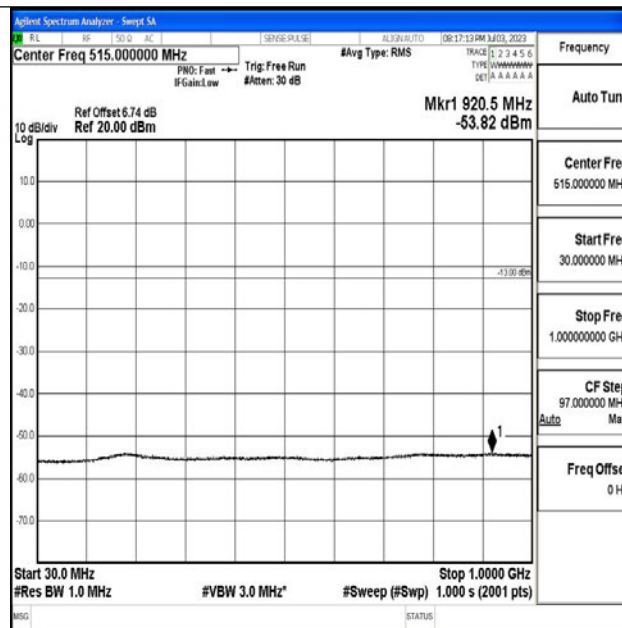
Band4_3MHz_16QAM_20175_1RB#0_30~1000_30~1000
