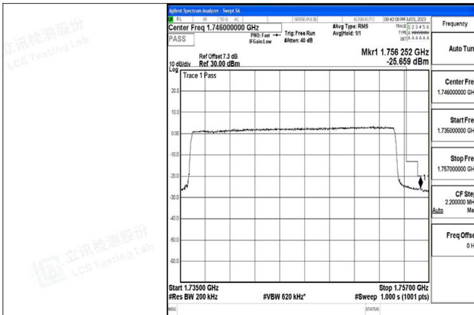
Band4_20MHz_QPSK_20300_100RB#0
