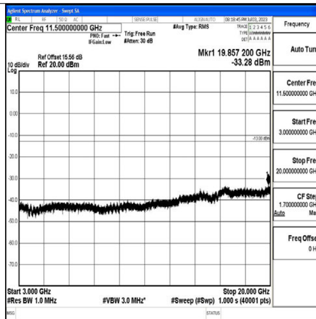
Band4_3MHz_16QAM_20385_1RB#0_3000~20000_3000~20000
