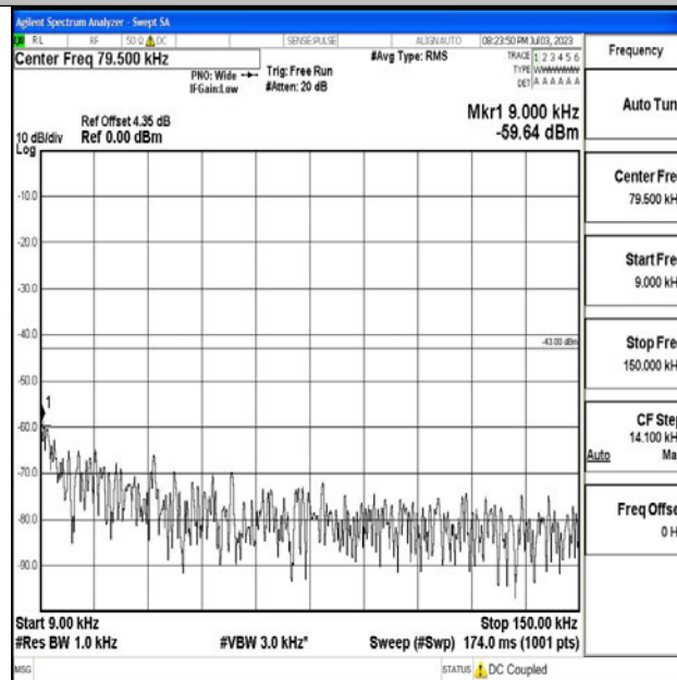
Band4_5MHz_QPSK_20175_1RB#0_0.009~0.15_0.009~0.15
