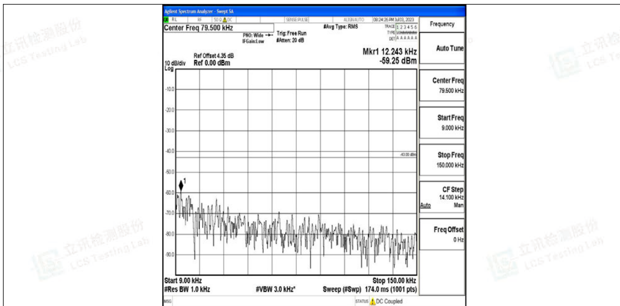
Band4_5MHz_16QAM_20175_1RB#0_0.009~0.15_0.009~0.15
