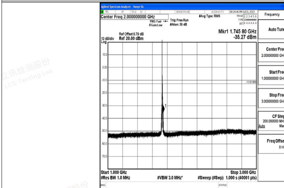
Band4_5MHz_16QAM_20175_1RB#0_1000~3000_1000~3000
