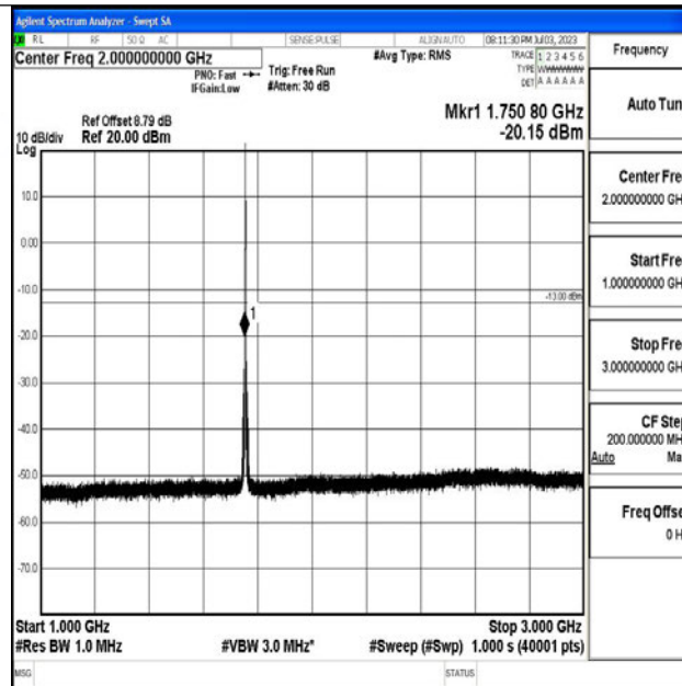
Band4_1.4MHz_QPSK_20393_1RB#0_1000~3000_1000~3000
