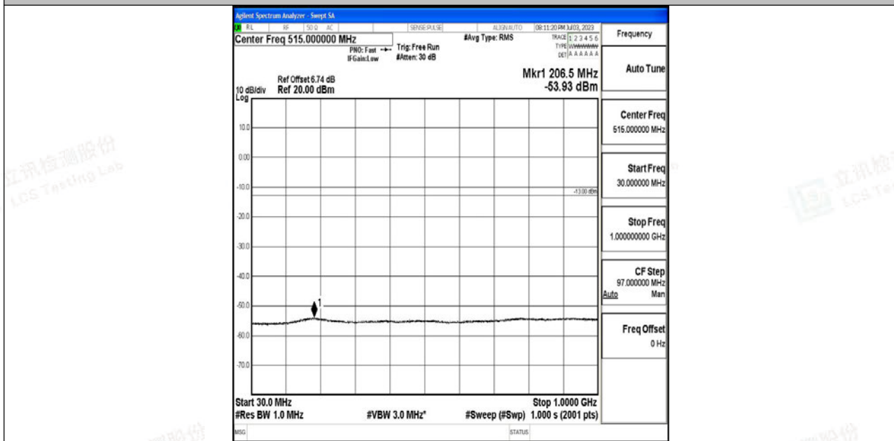
Band4_1.4MHz_QPSK_20393_1RB#0_30~1000_30~1000
