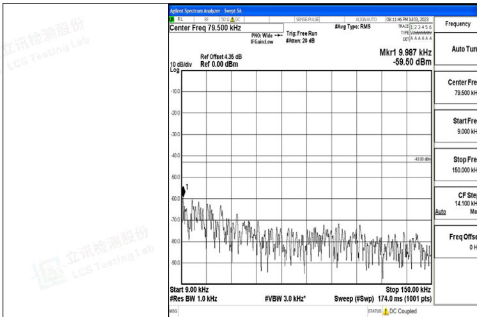
Band4_1.4MHz_16QAM_20393_1RB#0_0.009~0.15_0.009~0.15
