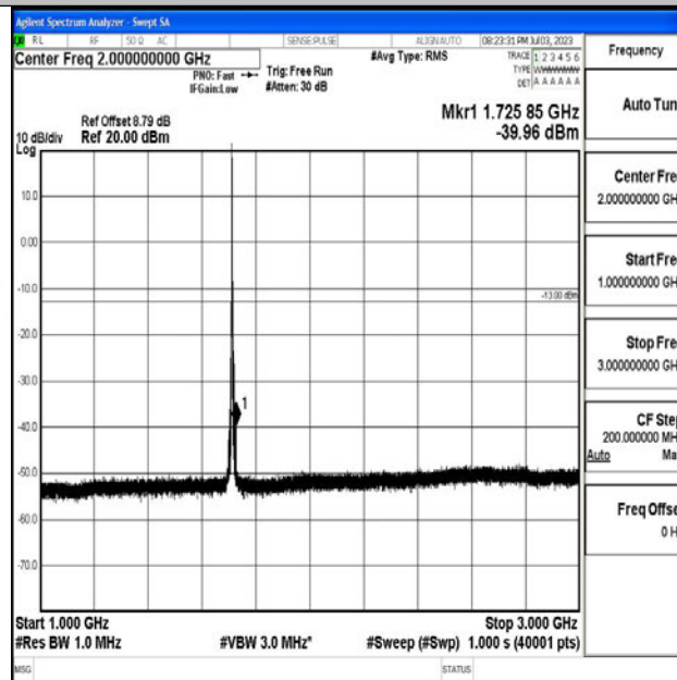
Band4_5MHz_16QAM_19975_1RB#0_1000~3000_1000~3000
