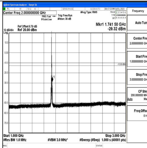
Band4_3MHz_16QAM_20175_1RB#0_1000~3000_1000~3000
