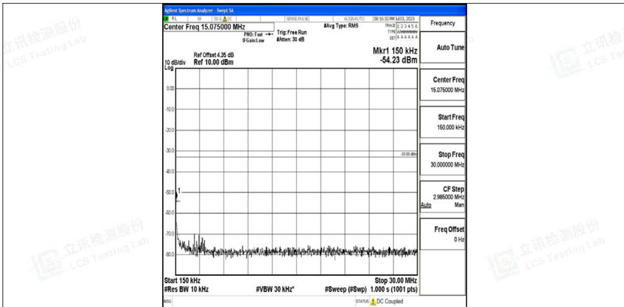
Band4_3MHz_QPSK_20175_1RB#0_0.15~30_0.15~30
