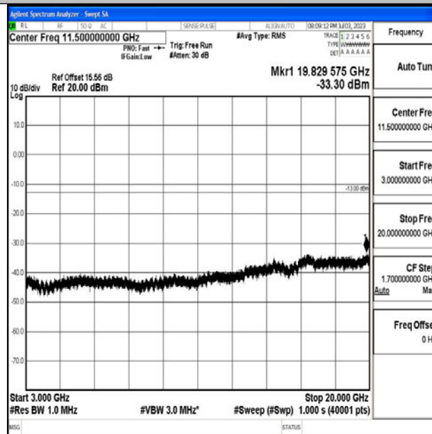
Band4_1.4MHz_QPSK_19957_1RB#0_3000~20000_3000~20000
