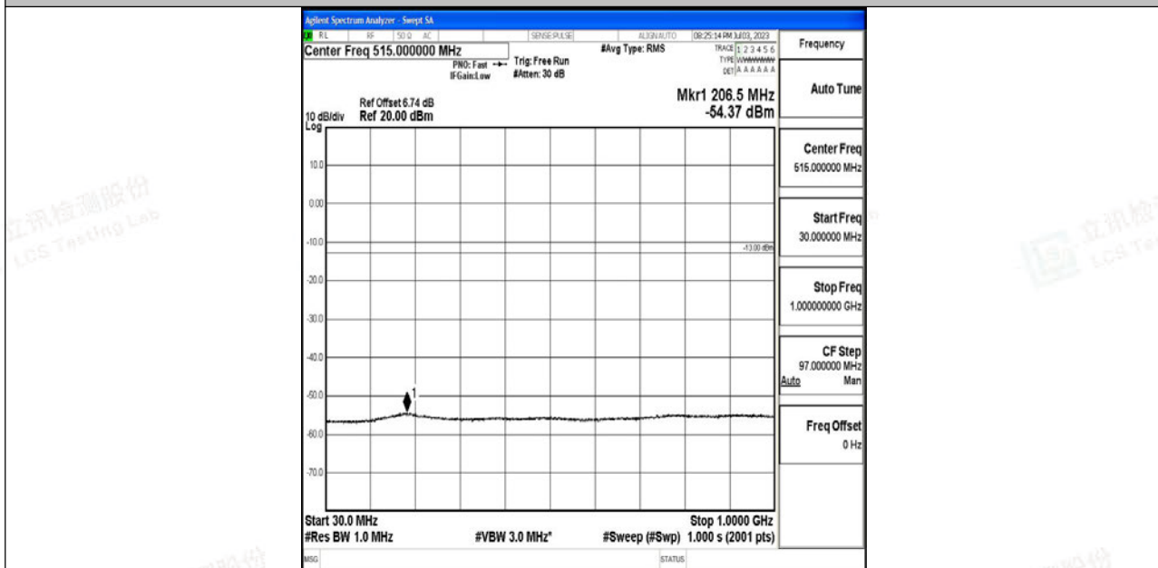
Band4_5MHz_QPSK_20375_1RB#0_30~1000_30~1000
