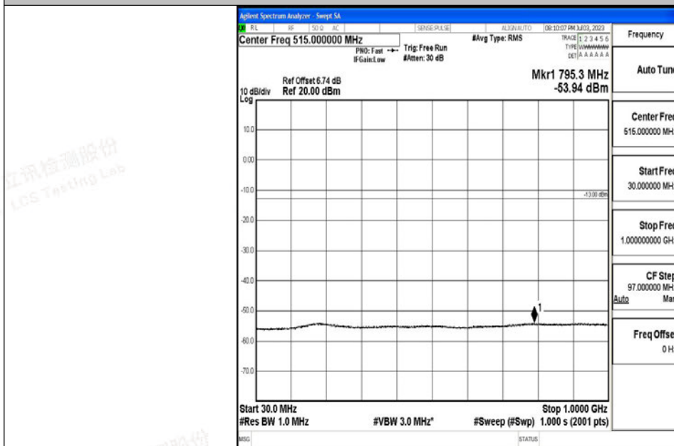
Band4_1.4MHz_QPSK_20175_1RB#0_30~1000_30~1000
