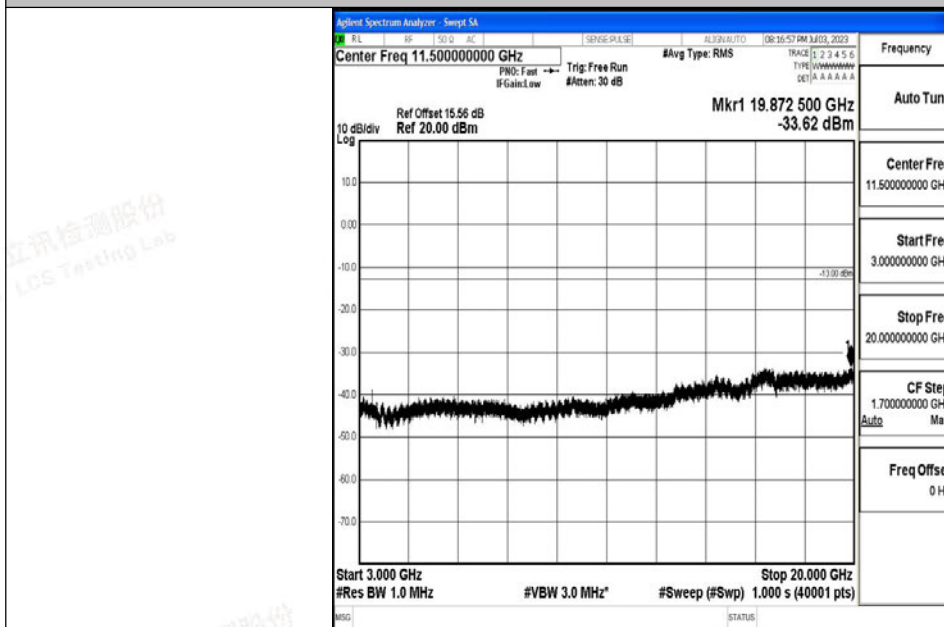
Band4_3MHz_QPSK_20175_1RB#0_3000~20000_3000~20000
