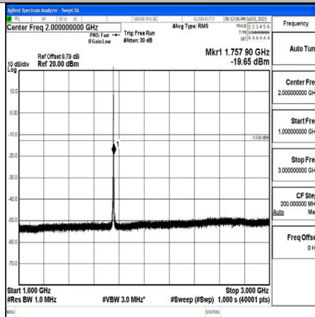
Band4_1.4MHz_16QAM_20393_1RB#0_1000~3000_1000~3000
