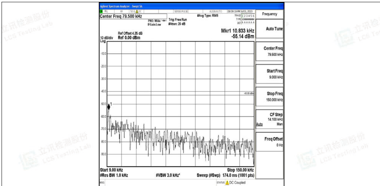
Band4_1.4MHz_16QAM_19957_1RB#0_0.009~0.15_0.009~0.15
