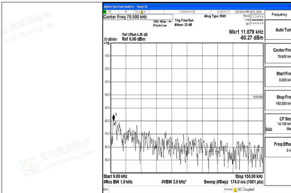
Band4_3MHz_16QAM_20385_1RB#0_0.009~0.15_0.009~0.15
