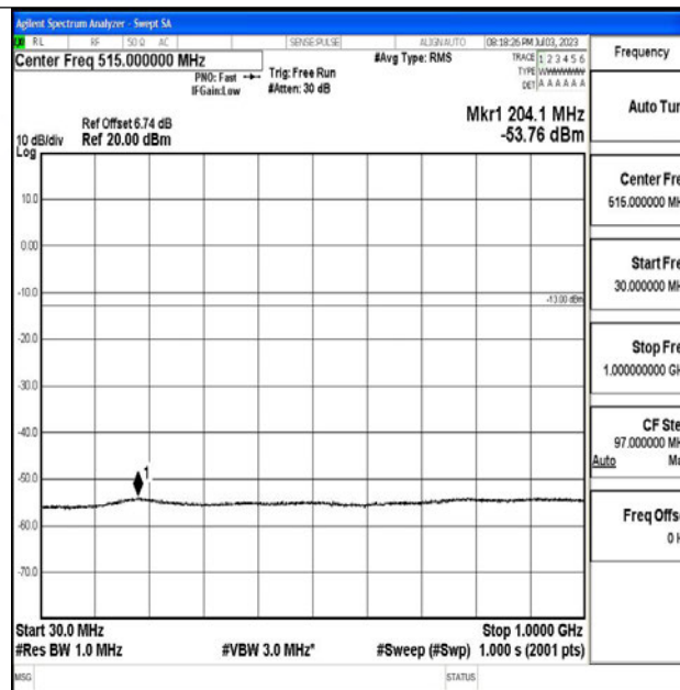
Band4_3MHz_16QAM_20385_1RB#0_30~1000_30~1000
