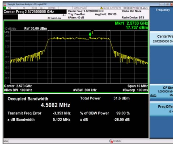
Band38-5MHz-QPSK-38000-25RB#0-4.5088
