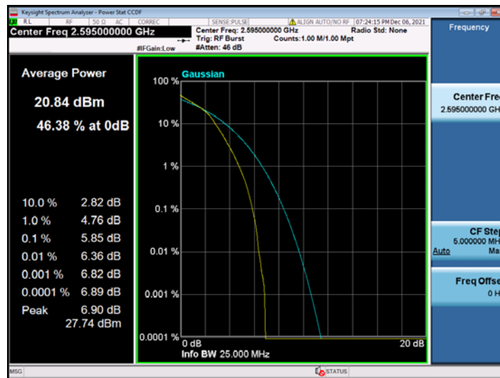
Band38-20MHz-16QAM-38150-100RB#0
