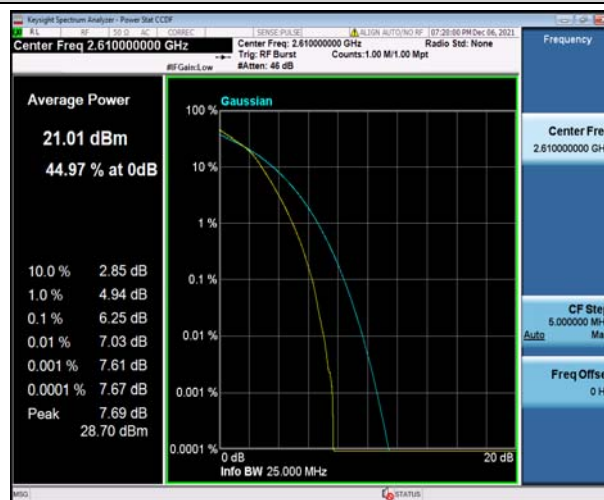
Band38-20MHz-16QAM-38150-100RB#0
