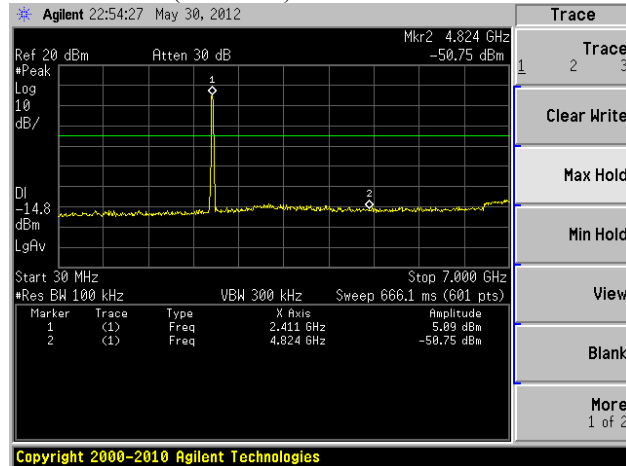
Figure 5. Spurious RF conducted emissions (continued)
