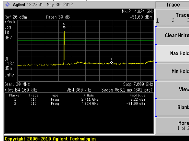
Figure 5. Spurious RF conducted emissions
