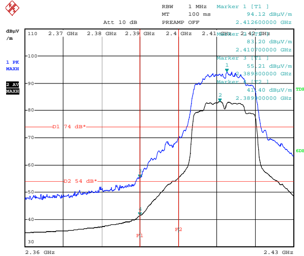
Figure 4. Plot of the Band Edge (Radiated) 802.11g mode:
