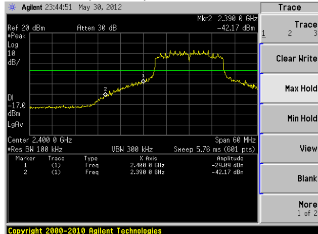
Figure 3. Plot of the Band Edge (Conducted)
