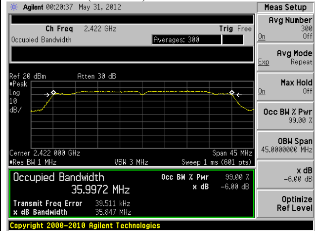
Figure 1. Plot of the 6dB Bandwidth &amp; Occupied Bandwidth (99%) (continued)
