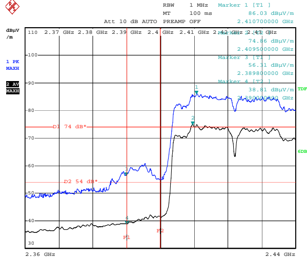
Figure 4. Plot of the Band Edge (Radiated) 802.11n HT40 mode:
