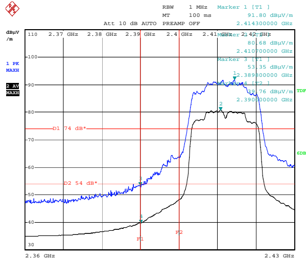
Figure 4. Plot of the Band Edge (Radiated) 802.11n HT20 mode:
